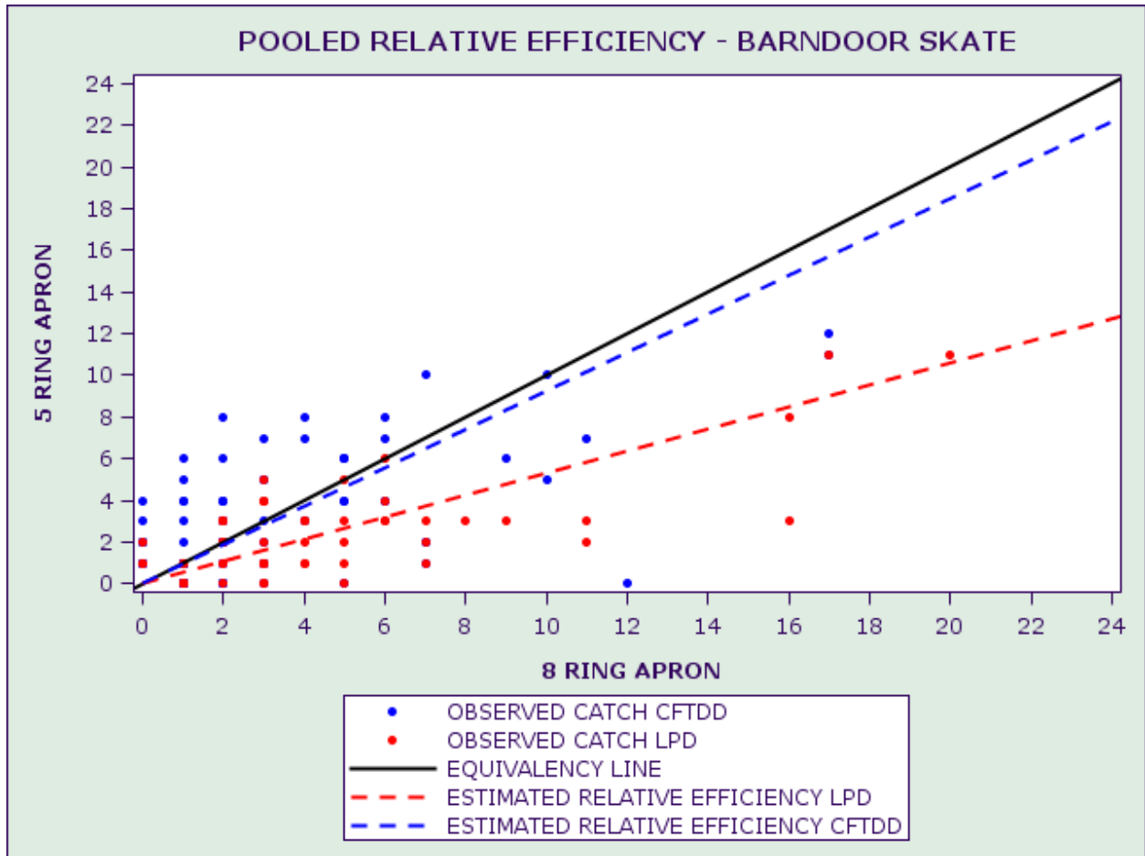
Figure 6 Total pooled catches for barndoor skate for the Experimental Dredge vs. the Control dredge. Model output from the analysis of the pooled data indicated that dredge frame was a significant factor and the two estimated relative efficiencies are show as the red and blue dashed lines. The black line has a slope of one.
