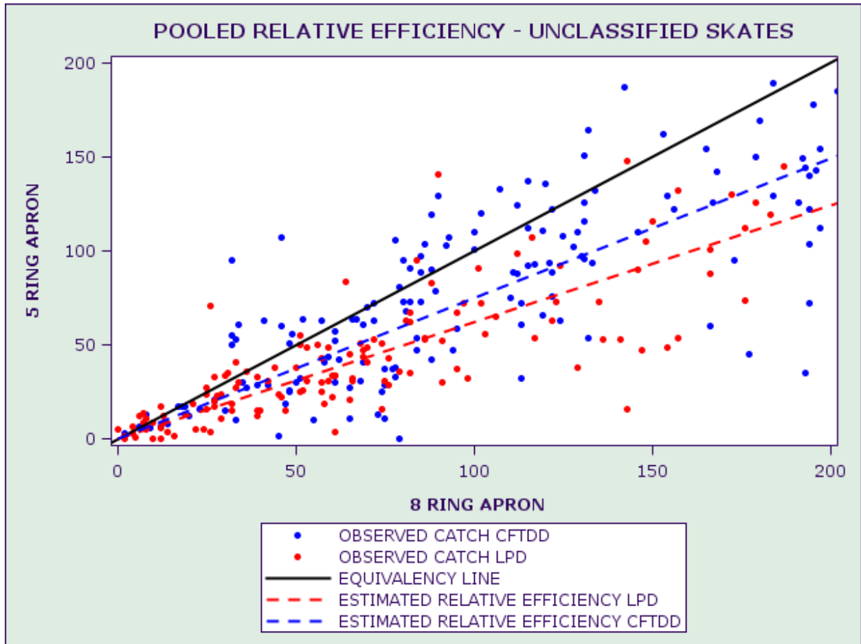
Figure 7 Total pooled catches for unclassified skate for the Experimental Dredge vs. the Control dredge. Model output from the analysis of the pooled data indicated that dredge frame was a significant factor and the two estimated relative efficiencies are show as the red and blue dashed lines. The black line has a slope of one.
