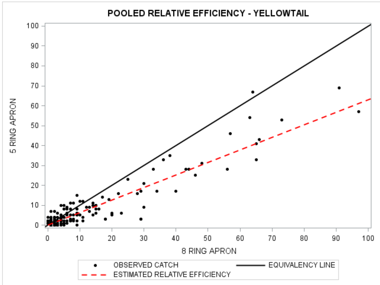
Figure 8 Total pooled catches for yellowtail flounder for the Experimental Dredge vs. the Control dredge. Model output from the analysis of the pooled data indicated that the intercept only model was the most appropriate specification. The estimated relative efficiency is show as the red dashed line. The black line has a slope of one.
