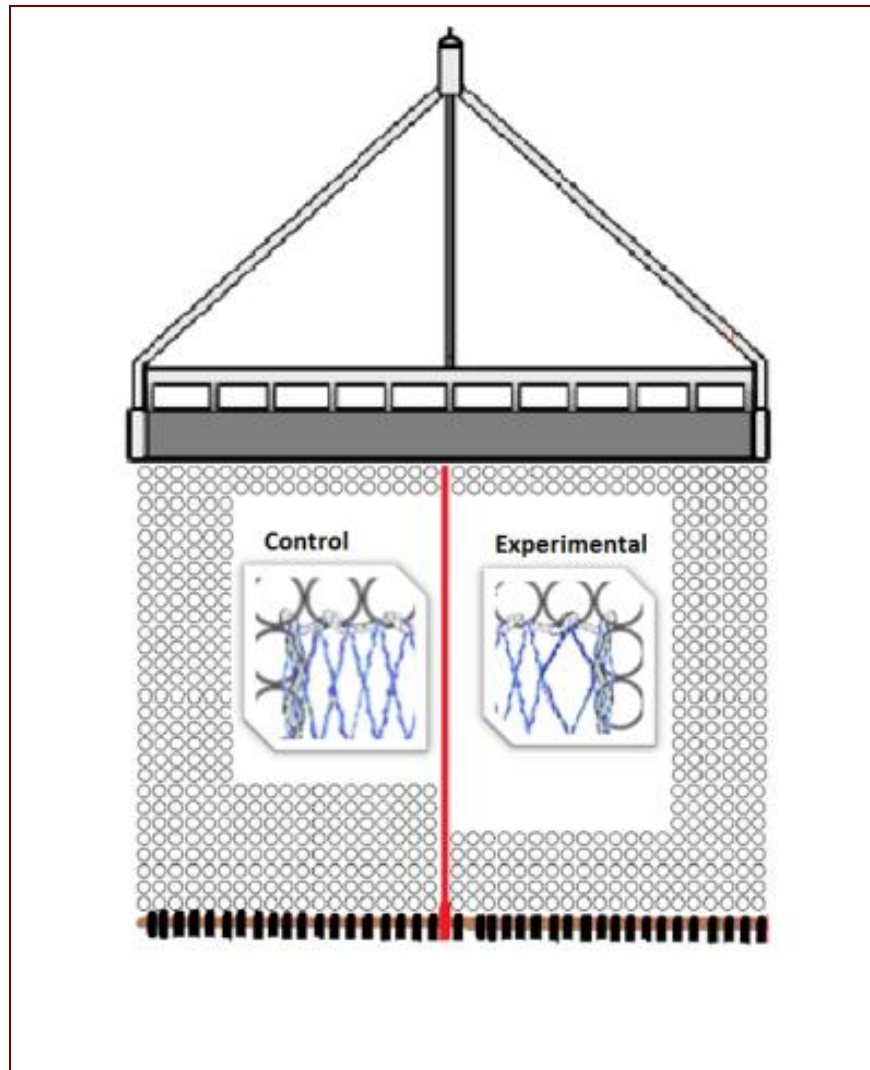
Figure 2 Diagram of the differences between the control and experimental bag design. The control dredge (left) has an 8 row apron and 60 mesh twine (2 meshes: 1 ring) and the experimental dredge (right) has a 5 row apron and a 45 mesh twine top (1.5 meshes: 1 ring).
