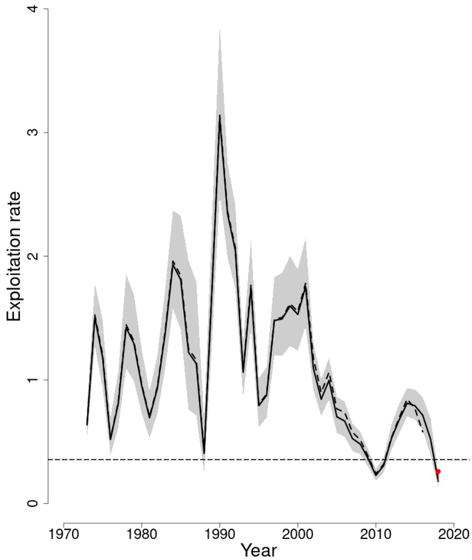
Figure 35: Trends in the fully selected fishing mortality ( F_{Full} ) of Southern New England-Mid Atlantic yellowtail flounder between 1973 and 2018 from the current (solid line) and previous (dashed line) assessment and the corresponding F_{Threshold} ( F_{MSY} proxy=0.355; horizontal dashed line). F_{Full} was adjusted for a retrospective pattern and the adjustment is shown in red based on the 2019 assessment. The approximate 90% lognormal confidence intervals are shown.
