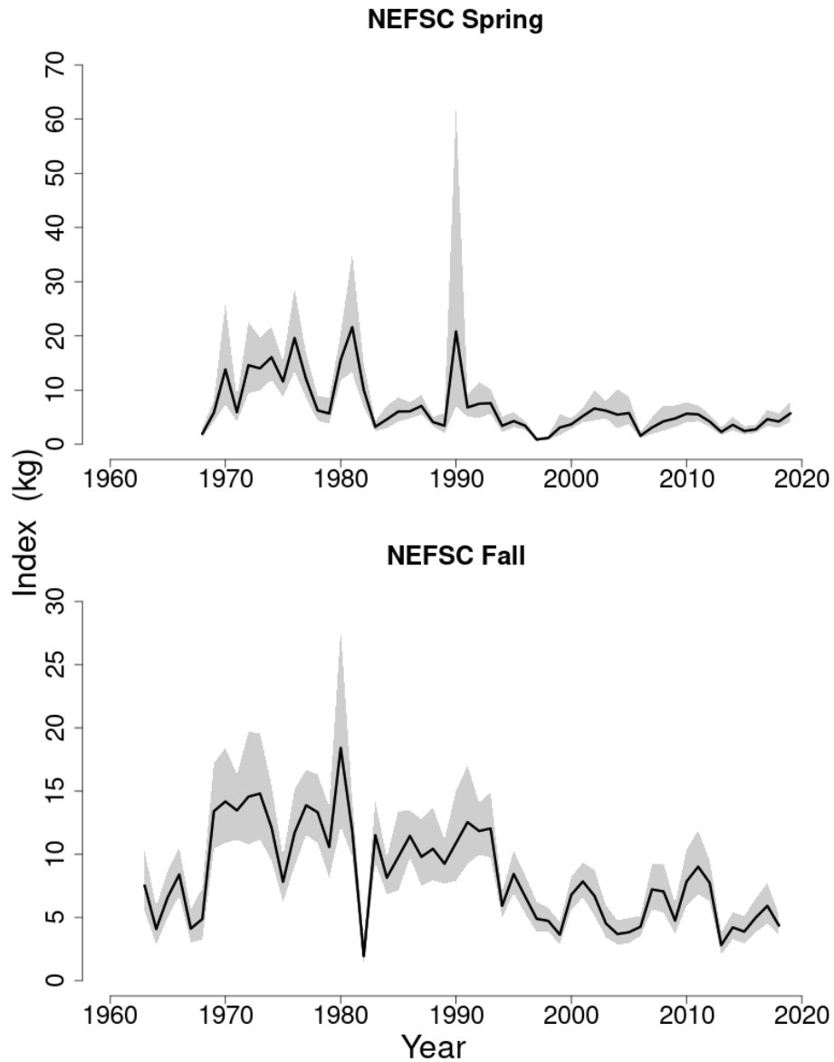
Figure 57: Indices of biomass for the white hake between 1963 and 2019 for the Northeast Fisheries Science Center (NEFSC) spring and fall bottom trawl surveys. The approximate 90% lognormal confidence intervals are shown.
