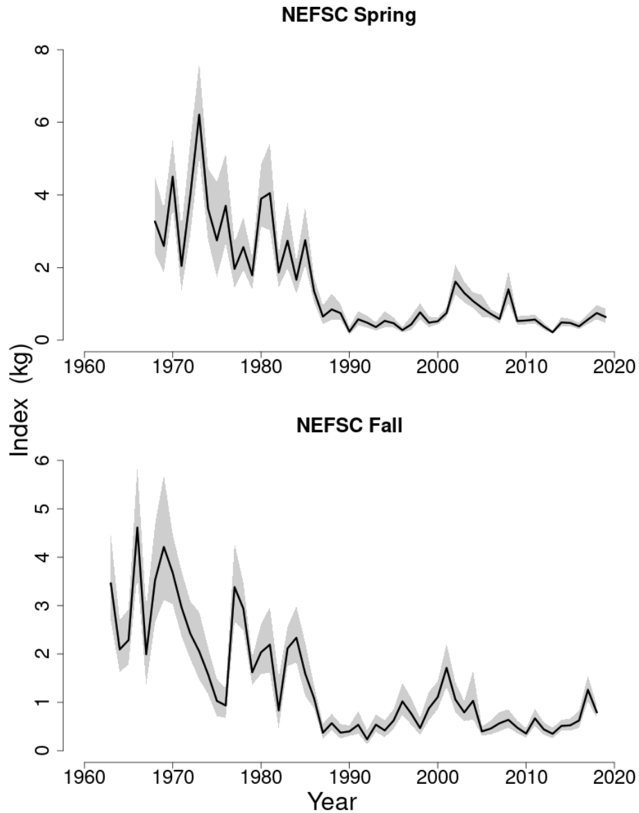
Figure 52: Indices of biomass for the witch flounder between 1963 (Fall) and 2019 (Spring) for the Northeast Fisheries Science Center (NEFSC) spring and fall bottom trawl surveys. The approximate 90% lognormal confidence intervals are shown.
