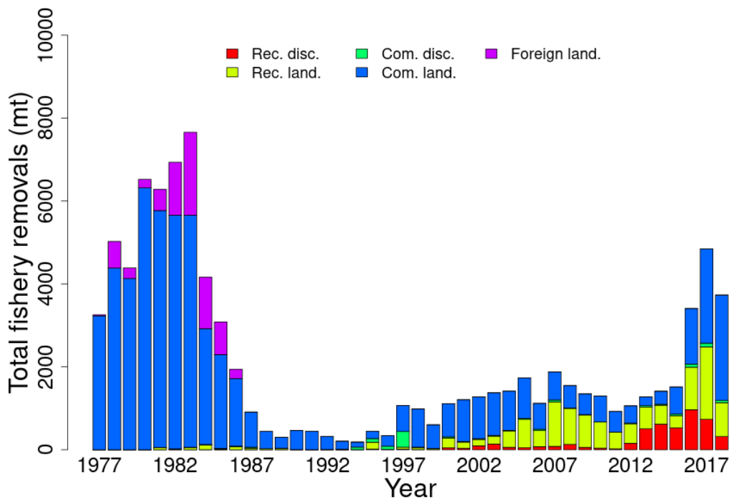
Figure 27: Total catch of Gulf of Maine haddock between 1977 and 2018 by fleet (commercial, recreational, or foreign) and disposition (landings and discards).
