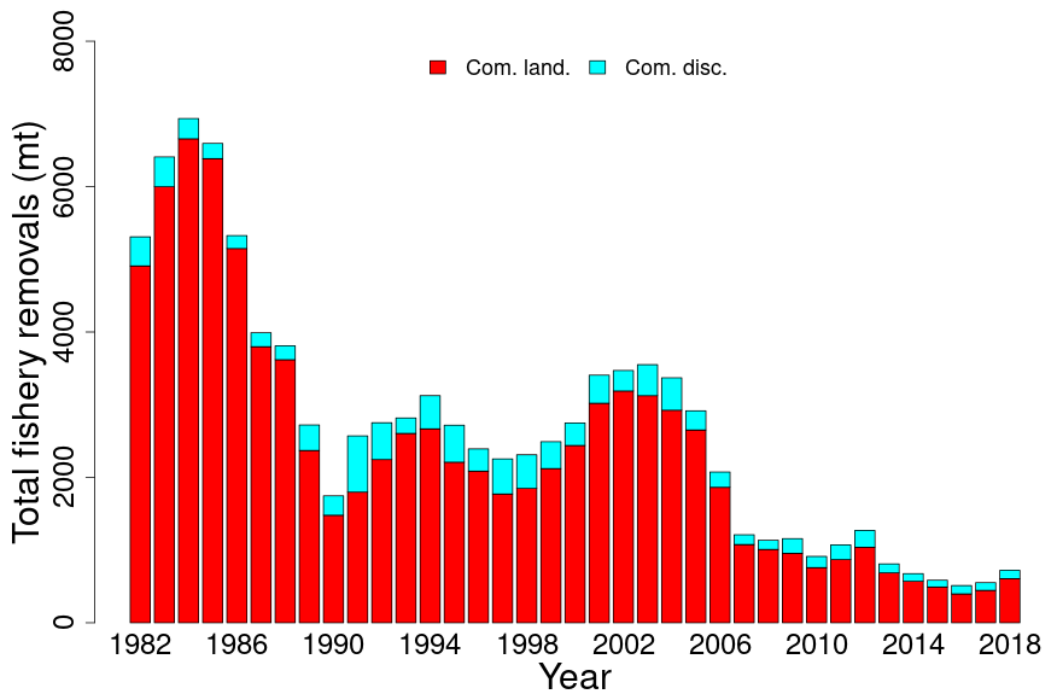
Figure 51: Total catch of witch flounder between 1982 and 2018 by fleet (commercial) and disposition (landings or discards).
