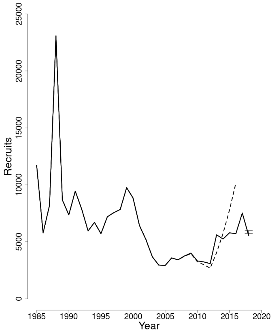
Figure 31: Trends in Recruits (age 1) (000s) of Cape Cod-Gulf of Maine yellowtail flounder between 1985 and 2018 from the current (solid line) and previous (dashed line) assessment. The 90% bootstrap probability intervals are shown.
