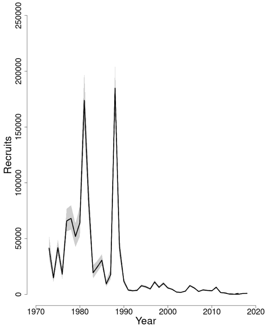
Figure 36: Trends in Recruitment (age 1) (000s) of Southern New England-Mid Atlantic yellowtail flounder between 1973 and 2018 from the current (solid line) and previous (dashed line) assessment. The approximate 90% lognormal confidence intervals are shown.
