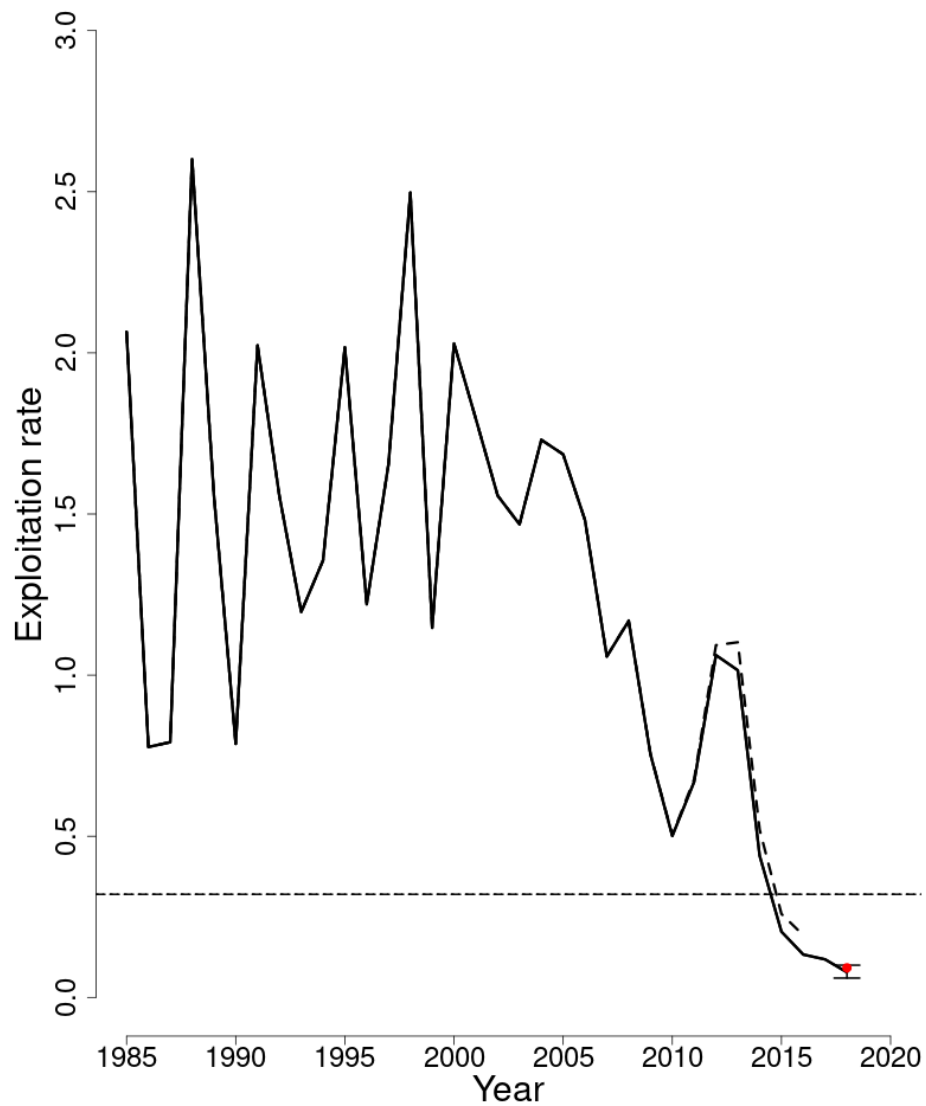
Figure 30: Trends in the fully selected fishing mortality ( F_{Full} ) of Cape Cod-Gulf of Maine yellowtail flounder between 1985 and 2018 from the current (solid line) and previous (dashed line) assessment and the corresponding F_{Threshold} ( F_{MSY} proxy=0.32; horizontal dashed line). F_{Full} was adjusted for a retrospective pattern and the adjustment is shown in red based on the 2019 assessment. The 90% bootstrap probability intervals are shown.
