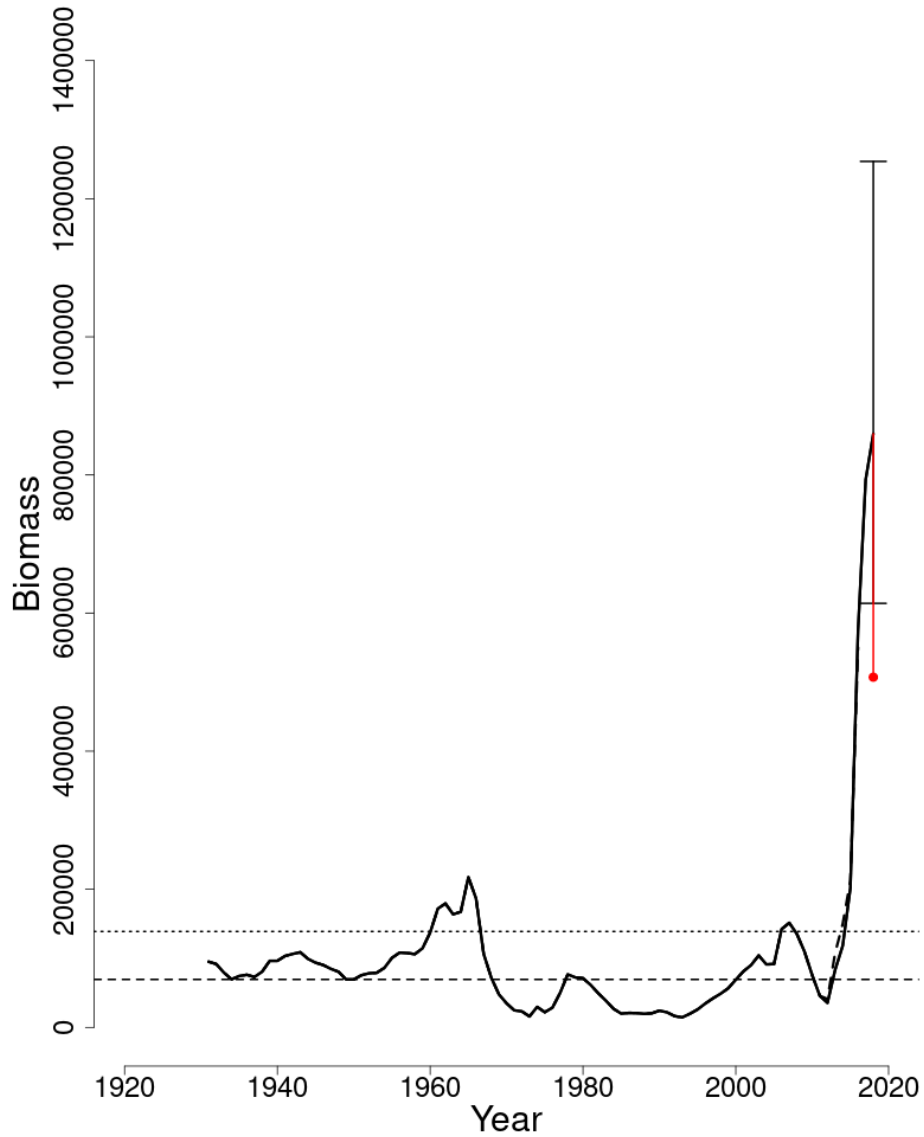
Figure 19: Trends in spawning stock biomass of Georges Bank haddock between 1931 and 2018 from the current (solid line) and previous (dashed line) assessment and the corresponding SSB_{Threshold} ( \frac{1}{2} SSB_{MSY} proxy; horizontal dashed line) as well as SSB_{Target} ( SSB_{MSY} proxy; horizontal dotted line) based on the 2019 assessment. Biomass was adjusted for a retrospective pattern and the adjustment is shown in red. The 90% bootstrap probability intervals are shown.
