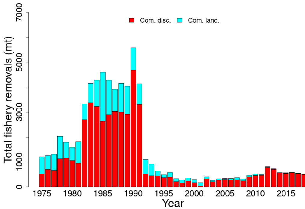
Figure 73: Total catch of southern New England - mid-Atlantic windowpane flounder between 1975 and 2018 by disposition (landings and discards).
