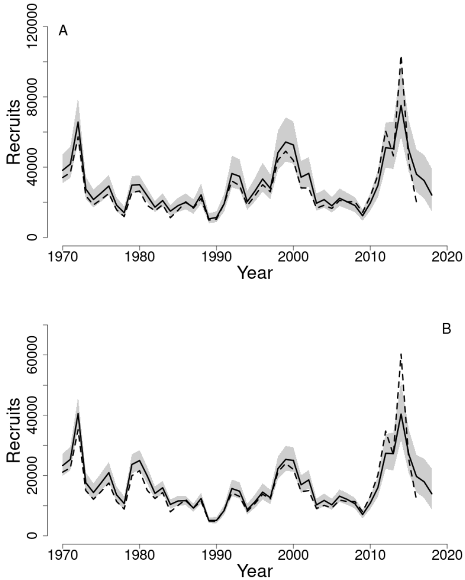
Figure 60: Estimated trends in age 1 recruitment (000s) of pollock between 1970 and 2018 from the current (solid line) and previous (dashed line) assessment for the assessment models base (A) and flat sel sensitivity (B). The approximate 90% lognormal confidence intervals are shown.
