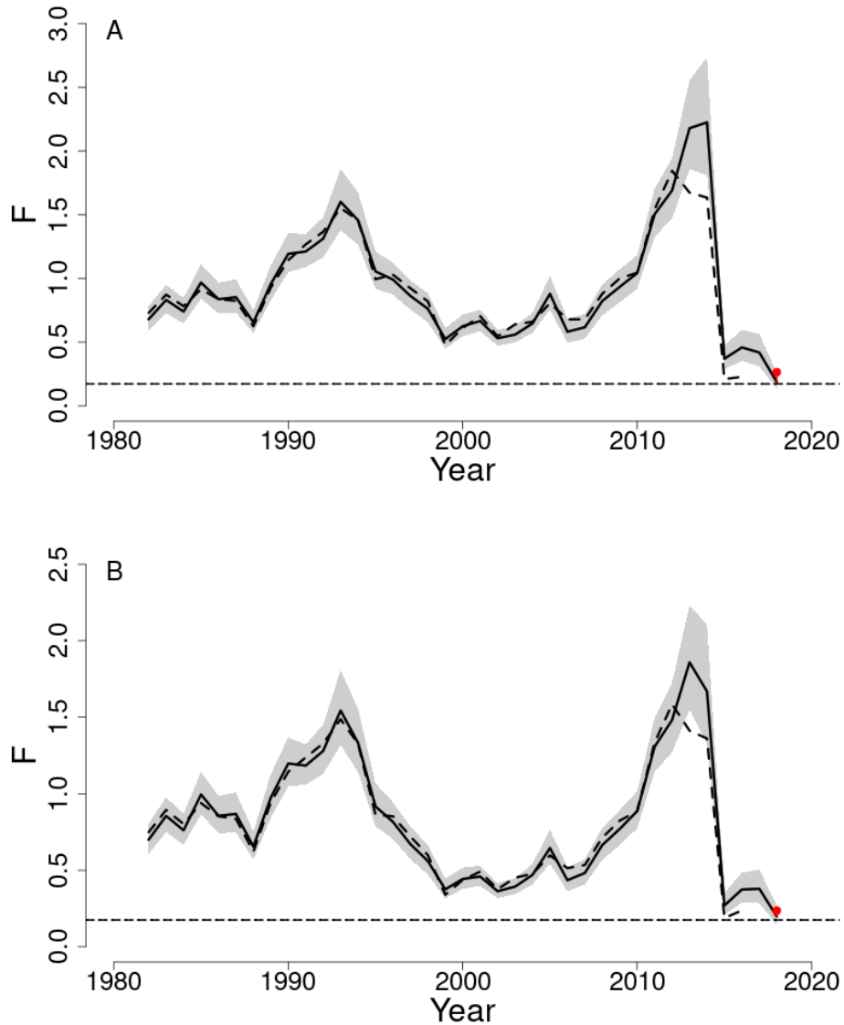
Figure 11: Estimated trends in the fully selected fishing mortality ( F ) of Gulf of Maine Atlantic cod between 1982 and 2018 from the current (solid line) and previous (dashed line) assessment and the corresponding F_{Threshold} (0.173 (M=0.2), 0.175 (M-ramp); dashed line) based on the 2019 M=0.2 (A) and M-ramp (B) assessment models. The 90% lognormal confidence intervals are shown. The red dot indicates the rho-adjusted F values that would have resulted had a retrospective adjustment been made to either model (see Special Comments section).
