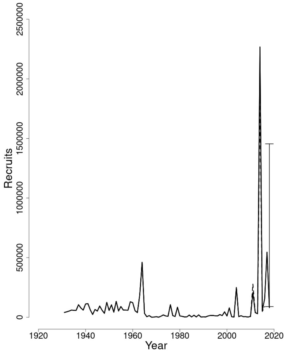
Figure 21: Trends in Recruits (age 1) (000s) of Georges Bank haddock between 1931 and 2018 from the current (solid line) and previous (dashed line) assessment. The 90% bootstrap probability intervals are shown.
