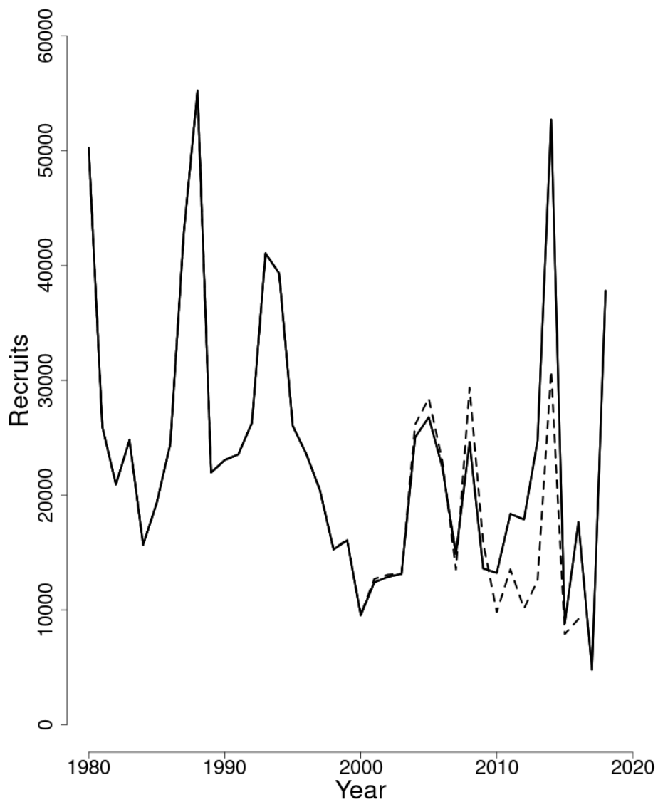
Figure 46: Trends in Recruits (age 1) (000s) of Gulf of Maine-Georges Bank American plaice between 1980 and 2018 from the current (solid line) and previous (dashed line) assessment.
