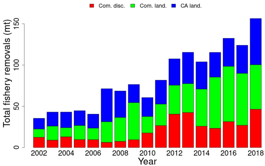
Figure 65: Total catch of Atlantic halibut between 2006 and 2018 by disposition (landings and discards).
