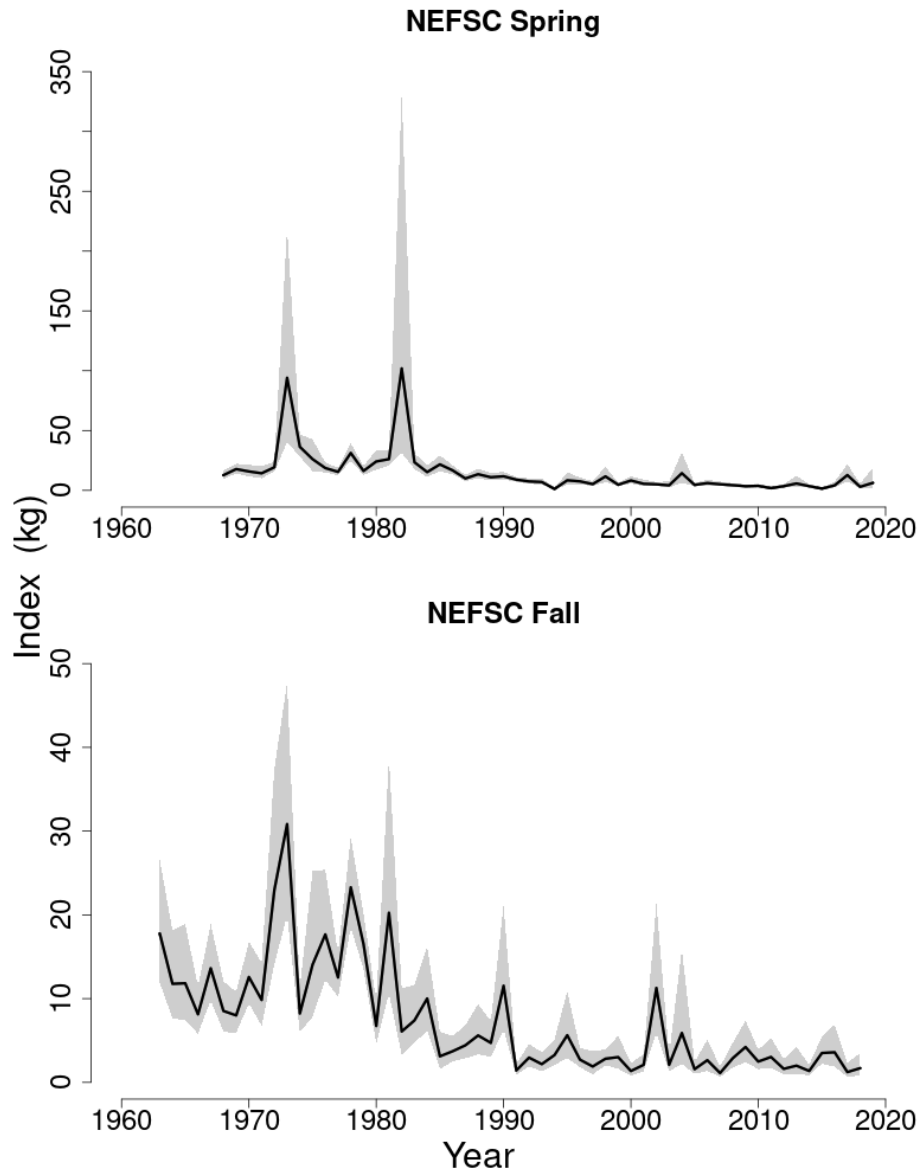
Figure 18: Indices of biomass for the Georges Bank Atlantic cod between 1963 and 2019 for the Northeast Fisheries Science Center (NEFSC) spring and fall trawl surveys. The approximate 90% lognormal confidence intervals are shown.
