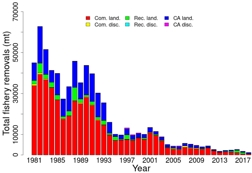
Figure 17: Total catch of Georges Bank Atlantic cod between 1981 and 2018 by fleet (US commercial, US recreational, or Canadian) and disposition (landings and discards).
