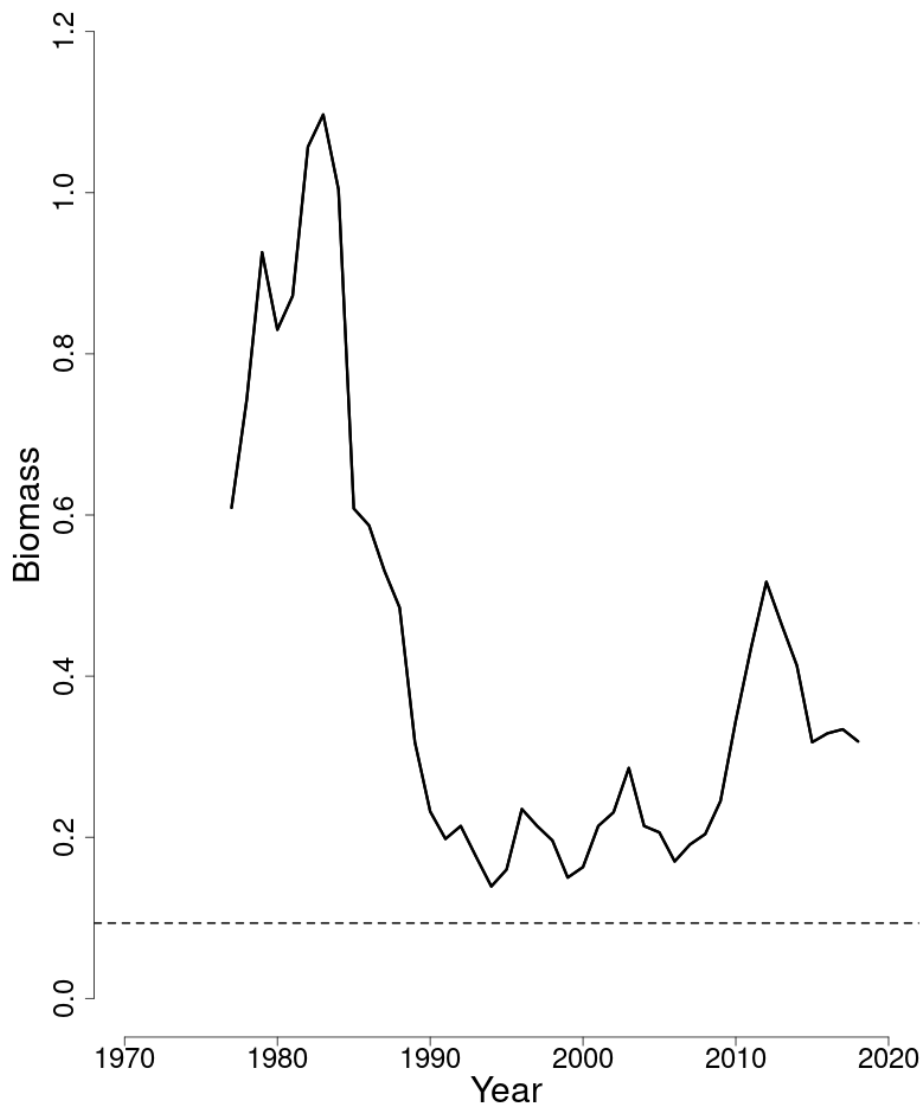
Figure 71: Trends in the biomass index (a 3-year moving average of the NEFSC fall bottom trawl survey index) of southern New England - mid-Atlantic windowpane flounder between 1975 and 2018 from the current assessment, and the corresponding B_{Threshold} = \frac{1}{2} B_{MSY} proxy = 0.094 kg/tow (horizontal dashed line).
