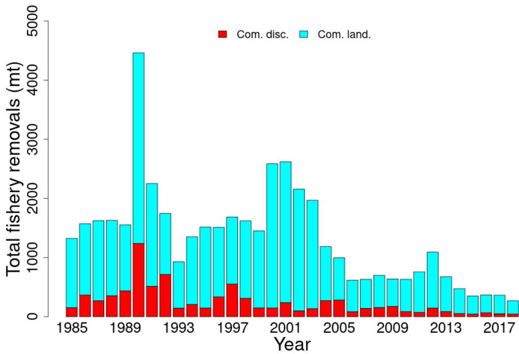
Figure 32: Total catch of Cape Cod-Gulf of Maine yellowtail flounder between 1985 and 2018 by disposition (landings and discards).
