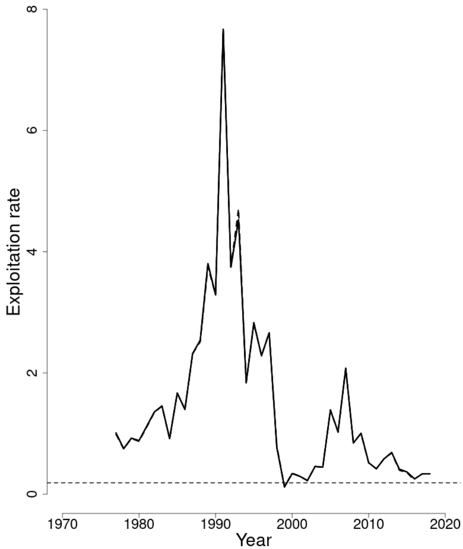
Figure 68: Trends in estimated relative fishing mortality of Gulf of Maine - Georges Bank windowpane flounder between 1975 and 2018 from the current assessment, and the corresponding F_{MSY} proxy = 0.185 (horizontal dashed line).
