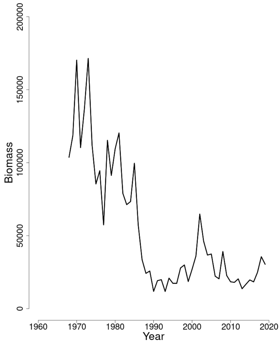
Figure 49: Trends in exploitable biomass (mt) of witch flounder between 1968 and 2019 from the current assessment.
