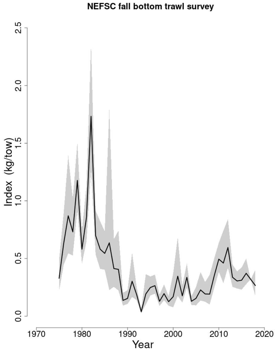
Figure 74: NEFSC fall bottom trawl survey indices in kg/tow for southern New England - mid-Atlantic windowpane flounder between 1975 and 2018. The approximate 90% lognormal confidence intervals are shown.
