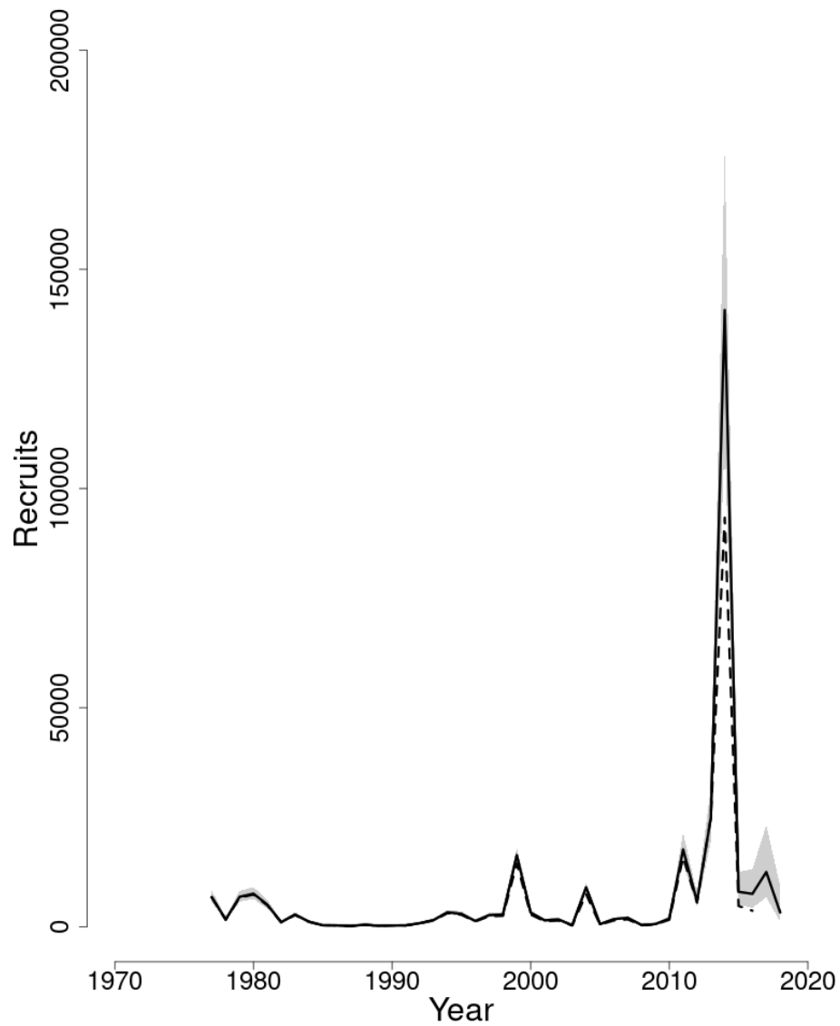
Figure 26: Trends in Recruits (age 1) (000s) of Gulf of Maine haddock between 1977 and 2018 from the current (solid line) and previous (dashed line) assessment. The approximate 90% lognormal confidence intervals are shown.
