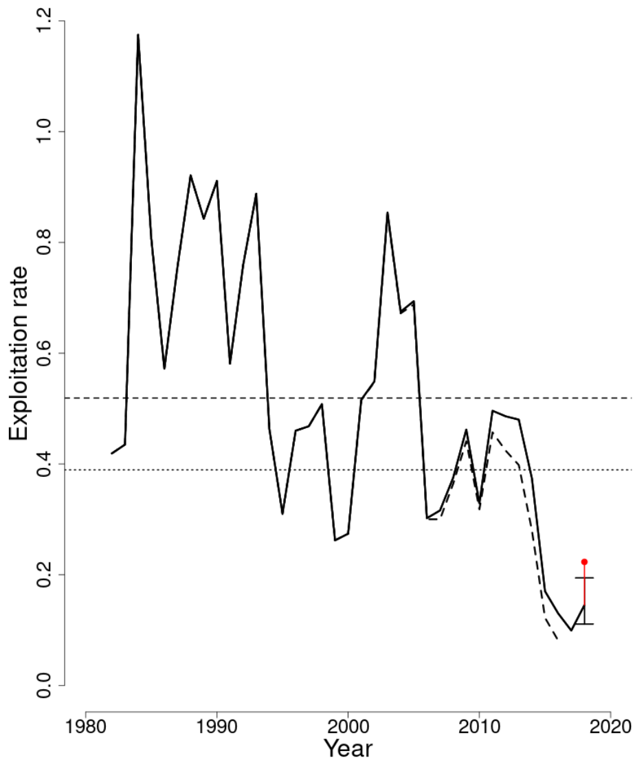
Figure 40: Trends in fully selected fishing mortality ( F_{Full} ) of Georges Bank Winter Flounder between 1982 and 2018 from the current (solid line) and previous (dashed line) assessments and the corresponding F_{Threshold} ( F_{MSY}=0.519 ; horizontal dashed line) as well as ( F_{Target}=75\% of FMSY; horizontal dotted line). F_{Full} was adjusted for a retrospective pattern and the adjustment is shown in red. The 90% normal confidence interval is shown for 2018.
