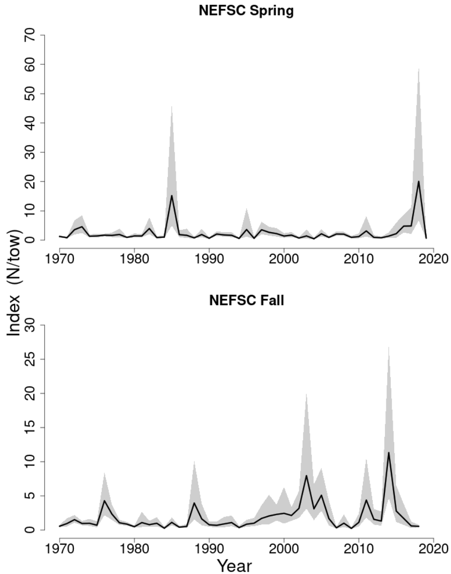
Figure 62: Indices of abundance for pollock from the Northeast Fisheries Science Center (NEFSC) spring (1970 to 2019) and fall (1970 to 2018) bottom trawl surveys. The approximate 90% lognormal confidence intervals are shown.
