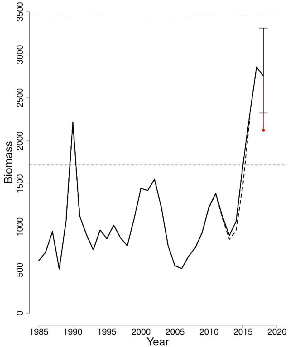
Figure 29: Trends in spawning stock biomass of Cape Cod-Gulf of Maine yellowtail flounder between 1985 and 2018 from the current (solid line) and previous (dashed line) assessment and the corresponding SSB_{Threshold} ( \frac{1}{2} SSB_{MSY} proxy; horizontal dashed line) as well as SSB_{Target} ( SSB_{MSY} proxy; horizontal dotted line) based on the 2019 assessment. Biomass was adjusted for a retrospective pattern and the adjustment is shown in red. The 90% bootstrap probability intervals are shown.
