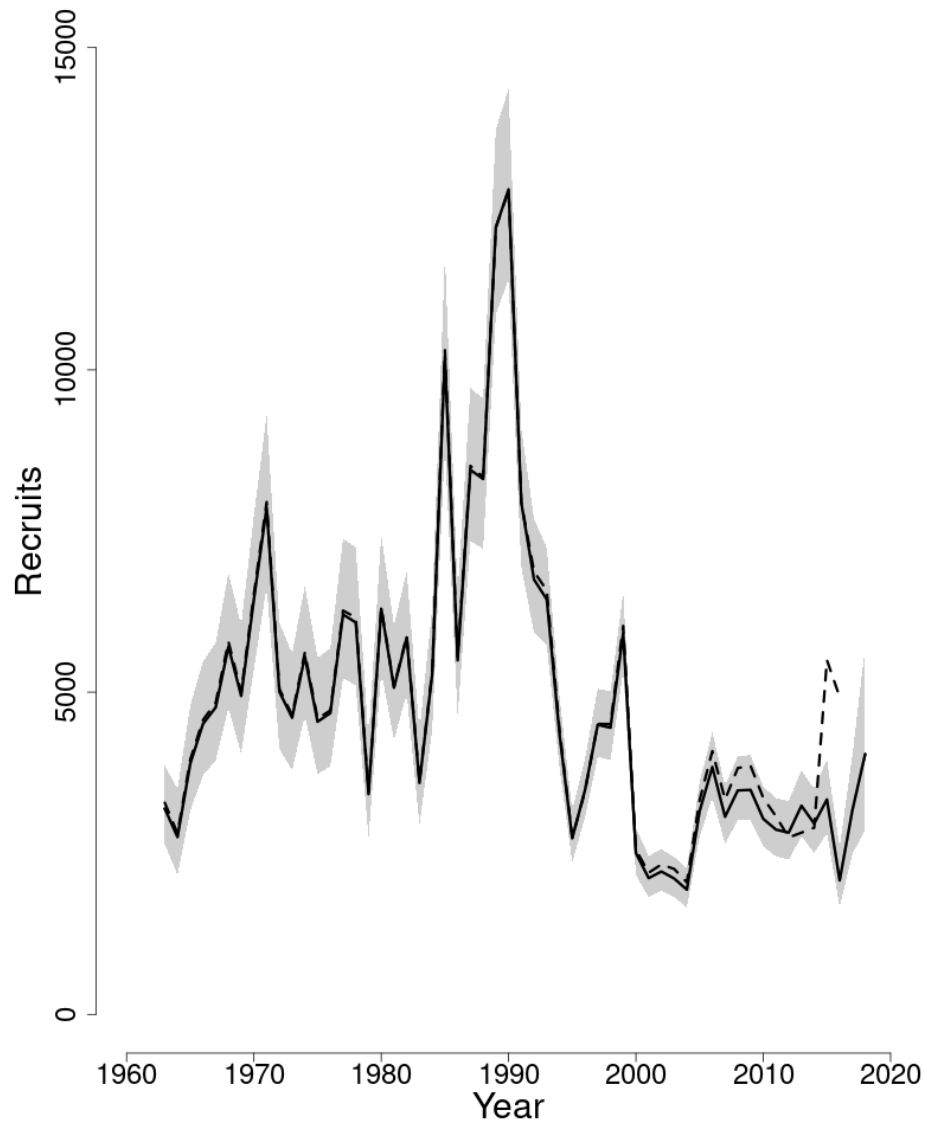
Figure 55: Trends in Recruits (age 1) (000s) of white hake between 1963 and 2018 from the current (solid line) and previous (dashed line) assessment. The approximate 90% lognormal confidence intervals are shown.
