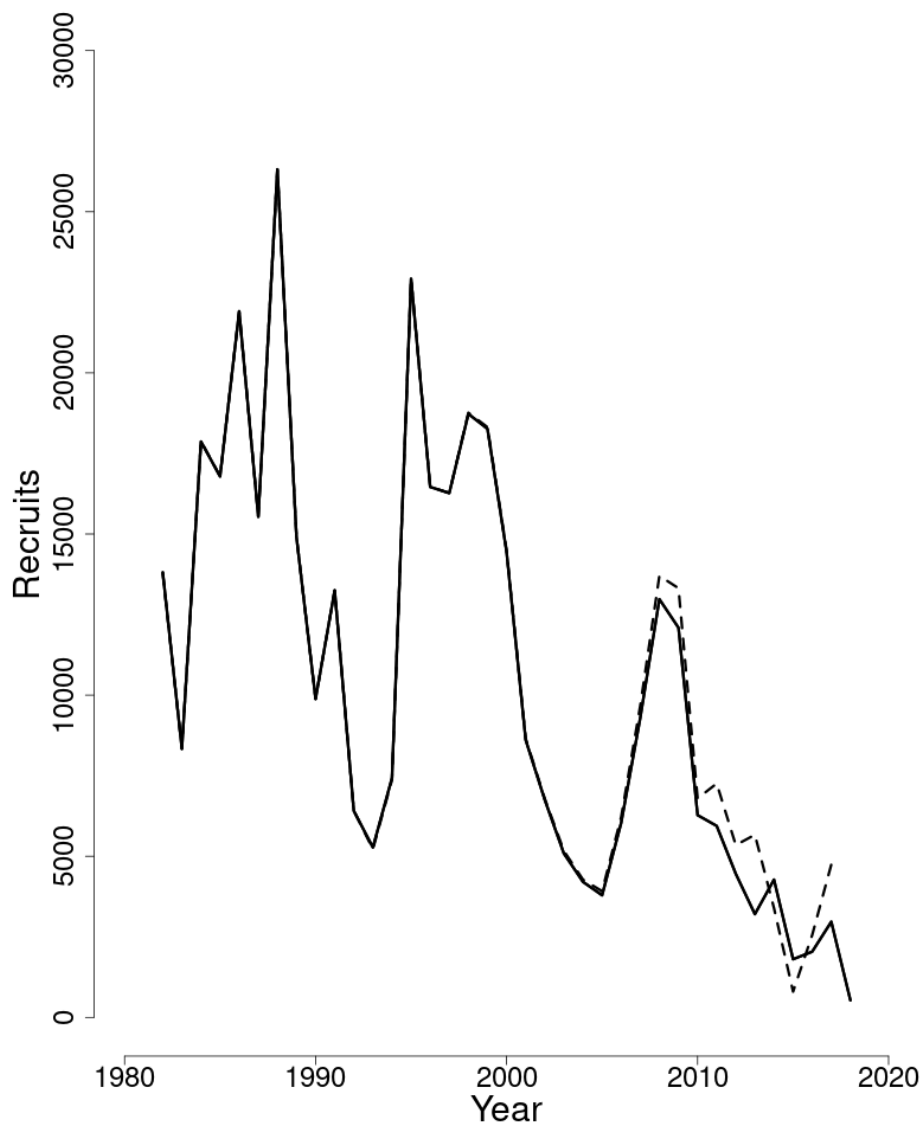
Figure 41: Trends in Recruits (age 1) (000s) of Georges Bank Winter Flounder between 1982 and 2018 from the current (solid line) and previous (dashed line) assessments.
