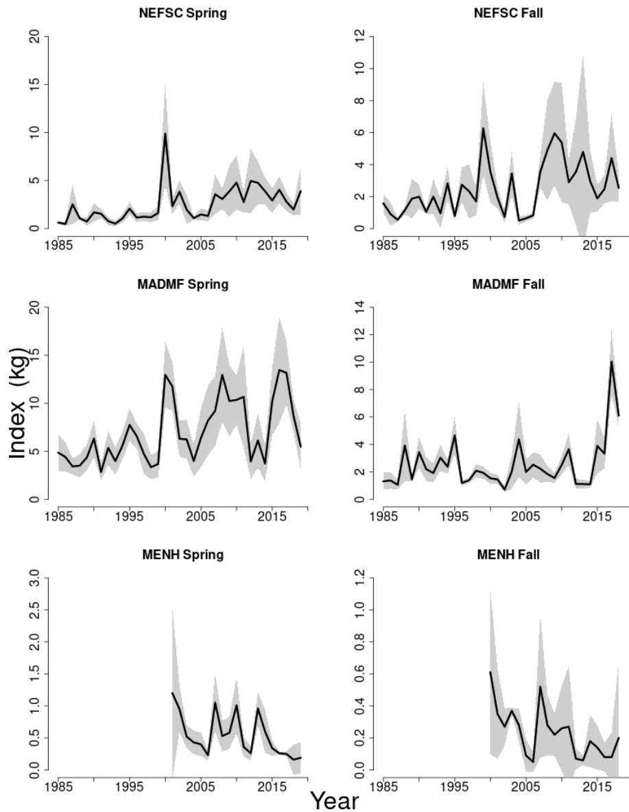
Figure 33: Indices of biomass for the Cape Cod-Gulf of Maine yellowtail flounder between 1985 and 2019 for the Northeast Fisheries Science Center (NEFSC) spring and fall bottom trawl surveys, Massachusetts Division of Marine Fisheries (MADMF) inshore state spring and fall bottom trawl surveys, and the Maine New Hampshire inshore state spring and fall state surveys. The 90% bootstrap probability intervals are shown.
