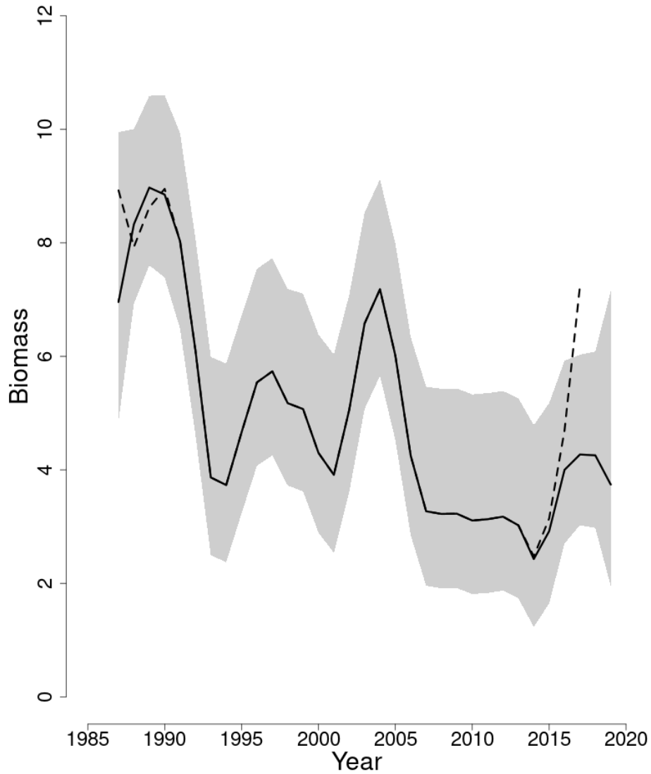
Figure 15: Trends in smoothed survey biomass (kg/tow) of Georges Bank Atlantic cod between 1987 and 2019 from the current (solid line) and previous (dashed line) assessment based on the 2019 assessment. The approximate 90% lognormal confidence intervals are shown.
