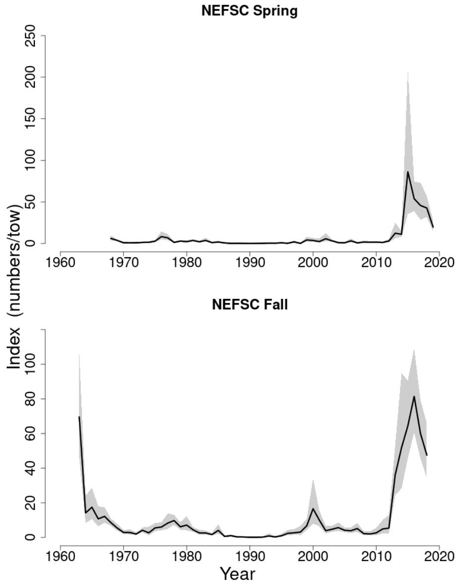
Figure 28: Indices of abundance for the Gulf of Maine haddock between 1963 and 2019 for the Northeast Fisheries Science Center (NEFSC) spring and fall bottom trawl surveys. The approximate 90% lognormal confidence intervals are shown.
