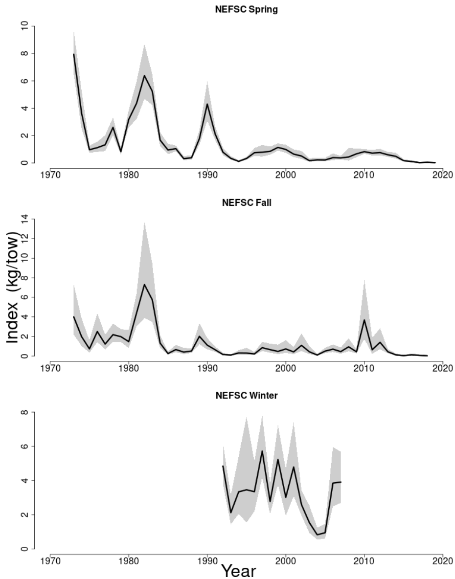
Figure 38: Indices of biomass for the Southern New England-Mid Atlantic yellowtail flounder between 1973 and 2019 for the Northeast Fisheries Science Center (NEFSC) spring, fall and winter bottom trawl surveys. The approximate 90% lognormal confidence intervals are shown. Note: Larval index based on Richardson et al (2009) was also used in this assessment and is available in the supplemental documentation.
