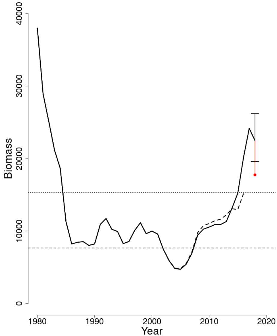
Figure 44: Trends in spawning stock biomass of Gulf of Maine-Georges Bank American plaice between 1980 and 2018 from the current (solid line) and previous (dashed line) assessment and the corresponding SSB_{Threshold} ( \frac{1}{2} SSB_{MSY} proxy; horizontal dashed line) as well as SSB_{Target} ( SSB_{MSY} proxy; horizontal dotted line) based on the 2019 assessment. Biomass was adjusted for a retrospective pattern and the adjustment is shown in red. The approximate 90% normal confidence intervals are shown.
