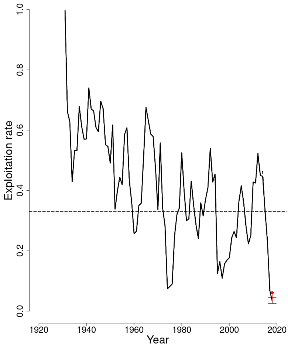
Figure 20: Trends in the average fishing mortality ( \bar{F}_{5-7} ) of Georges Bank haddock between 1931 and 2018 from the current (solid line) and previous (dashed line) assessment and the corresponding F_{Threshold} ( F_{MSY} proxy=0.33; horizontal dashed line) based on the 2019 assessment. \bar{F}_{5-7} was adjusted for a retrospective pattern and the adjustment is shown in red. The 90% bootstrap probability intervals are shown.
