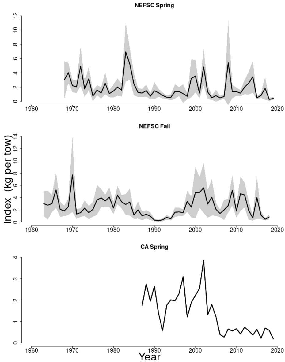
Figure 43: Indices of biomass for the Georges Bank Winter Flounder for the Northeast Fisheries Science Center (NEFSC) spring (1968-2019) and fall (1963-2018) bottom trawl surveys and the Canadian DFO spring survey (1987-2019). The 90% normal confidence interval is shown.
