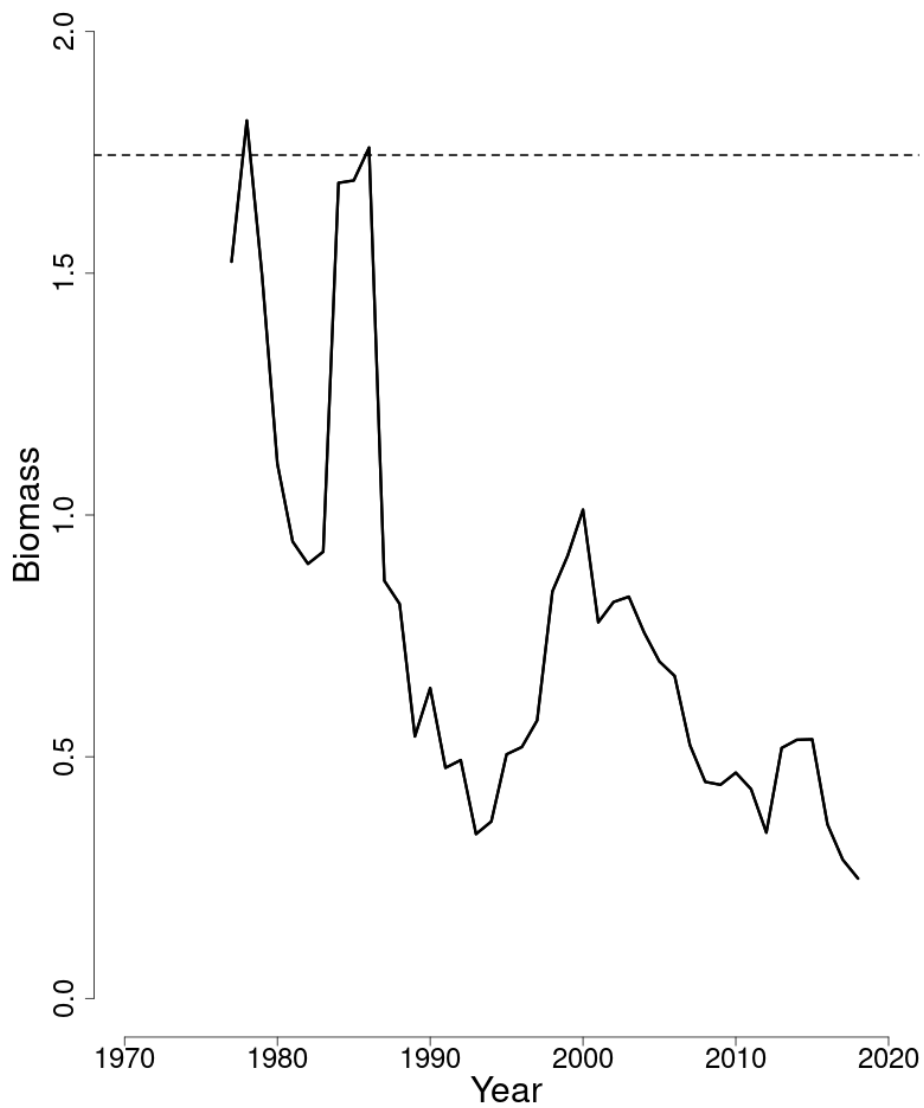
Figure 67: Trends in the biomass index (a 3-year moving average of the NEFSC fall bottom trawl survey index) of Gulf of Maine - Georges Bank windowpane flounder between 1975 and 2018 from the current assessment, and the corresponding B_{Threshold} = \frac{1}{2} B_{MSY} proxy = 1.745 kg/tow (horizontal dashed line).
