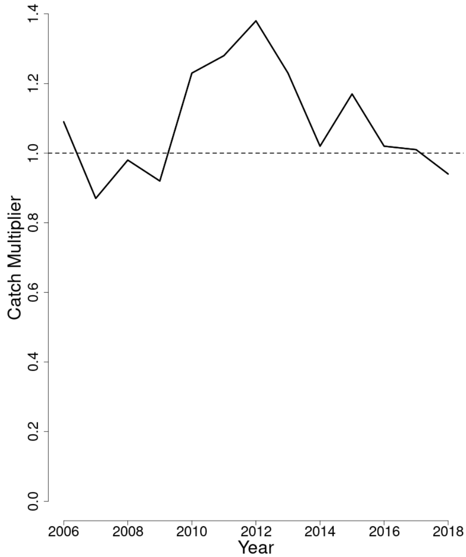
Figure 63: The catch multiplier resulting from the FSD model for Atlantic halibut between 2006 and 2018 from the current (solid line) assessment. A dashed line at 1 is added for reference.
