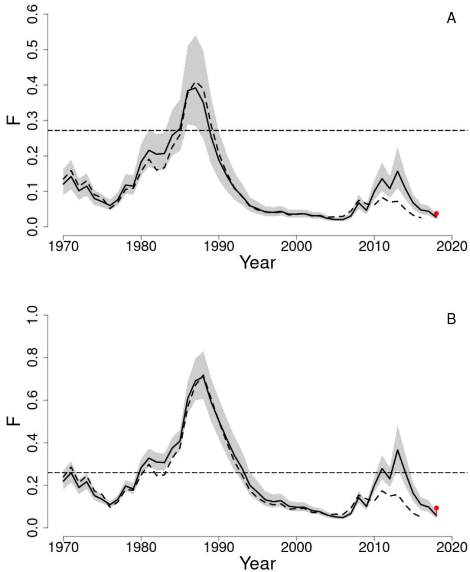
Figure 59: Estimated trends in age 5 to 7 average F ( F_{AVG} ) of pollock between 1970 and 2018 from the current (solid line) and previous (dashed line) assessment and the corresponding F_{Threshold} ( F_{MSY} proxy; dashed line) based on the 2019 assessment models base (A) and flat sel sensitivity (B). F_{AVG} was adjusted for a retrospective pattern and the adjustment is shown in red. The approximate 90% lognormal confidence intervals are shown.
