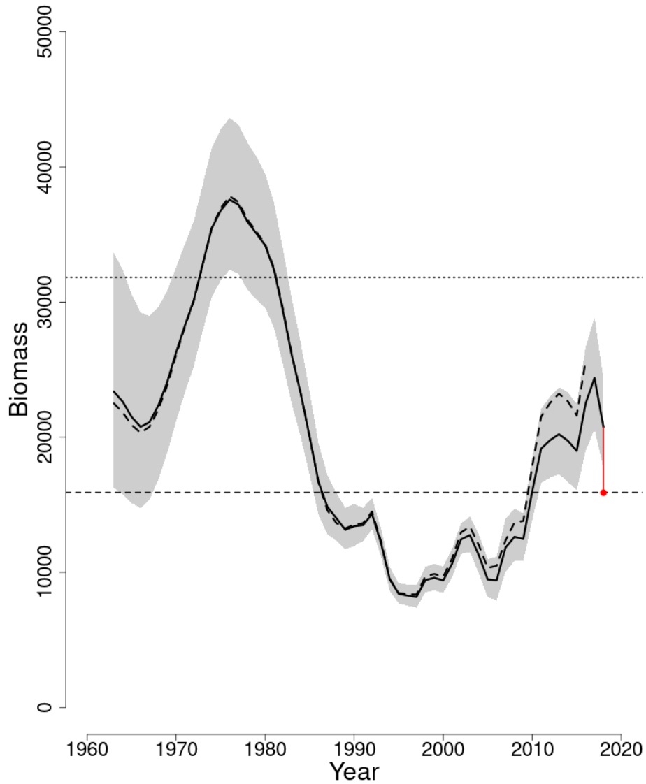
Figure 53: Trends in spawning stock biomass of white hake between 1963 and 2018 from the current (solid line) and previous (dashed line) assessment and the corresponding SSB_{Threshold} ( \frac{1}{2} SSB_{MSY} proxy; horizontal dashed line) as well as SSB_{Target} ( SSB_{MSY} proxy; horizontal dotted line) based on the 2019 assessment. Biomass was adjusted for a retrospective pattern and the adjustment is shown in red. The approximate 90% lognormal confidence intervals are shown.
