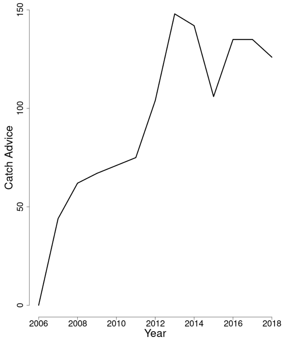
Figure 64: The catch advice resulting from multiplying catch and the catch multiplier from the FSD model for Atlantic halibut between 2006 and 2018 from the current assessment.
