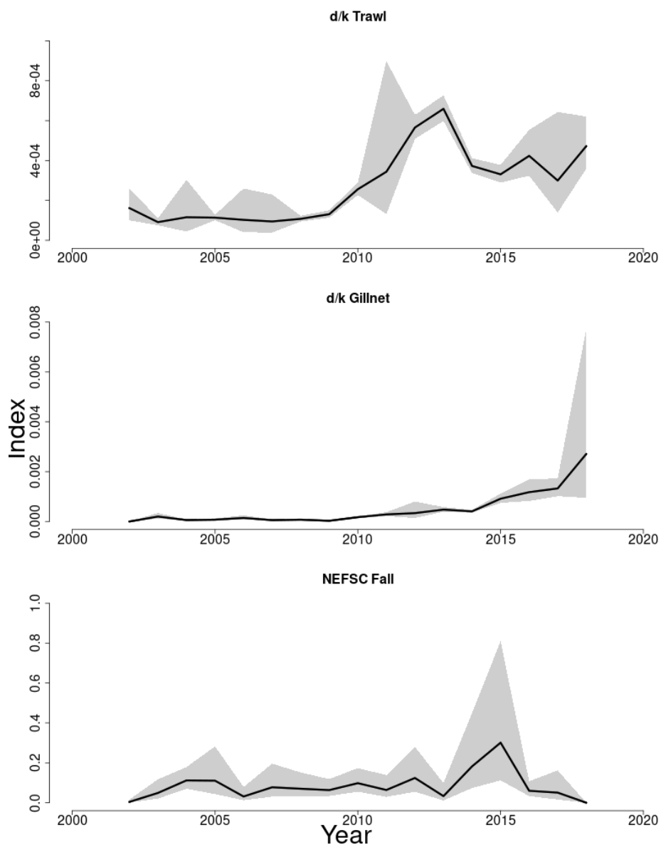
Figure 66: Indices of biomass for the Atlantic halibut between 2002 and 2018 for the Northeast Fisheries Science Center (NEFSC) fall bottom trawl survey and 2 discard ratio estimators. Discard mortality is assumed to be 0.76 for trawl gear and 0.3 for gillnet gear. The 90% lognormal confidence intervals are shown.
