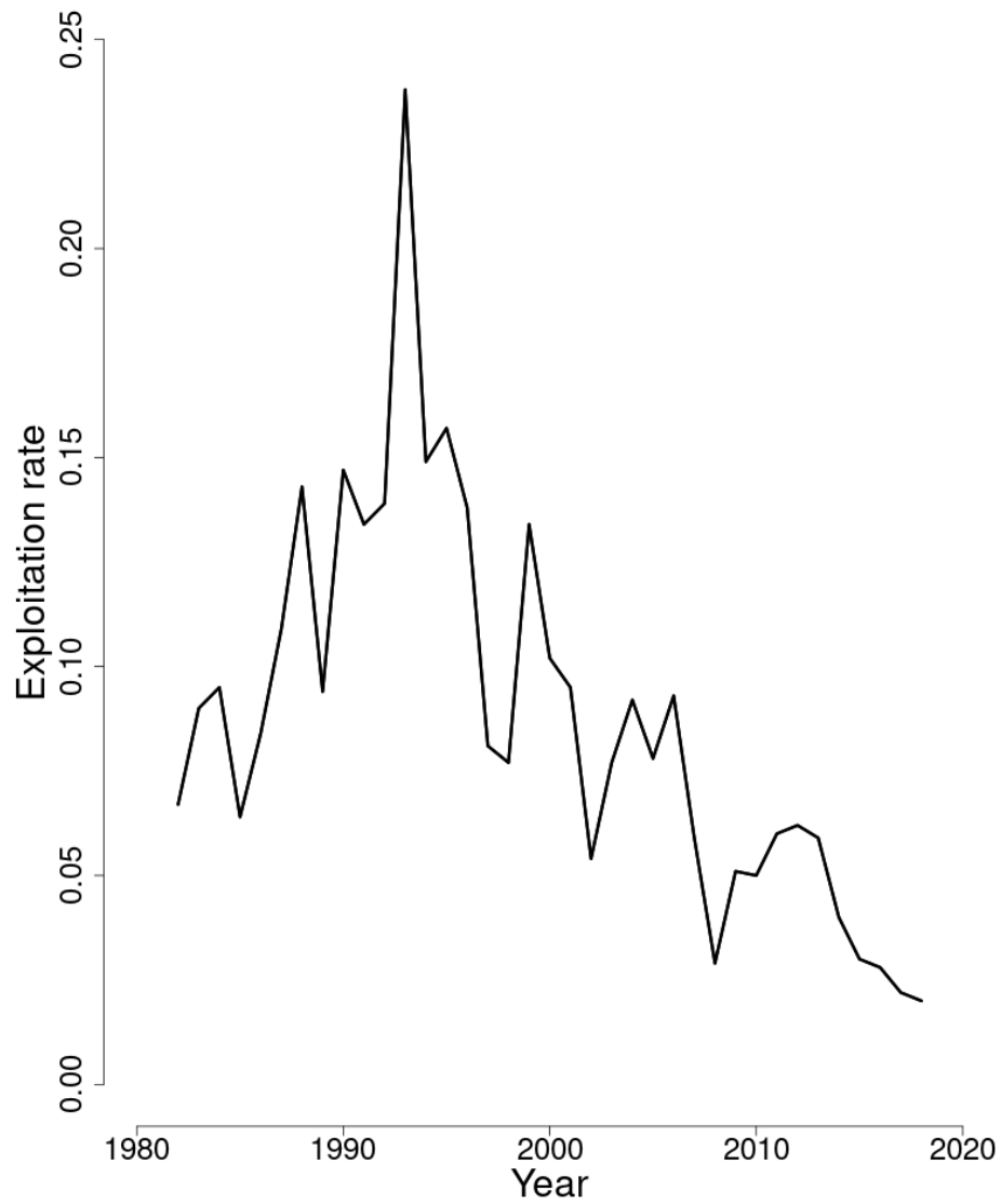
Figure 50: Trends in the exploitation rate (catch/ exploitable biomass) of witch flounder between 1982 and 2018 from the current assessment.
