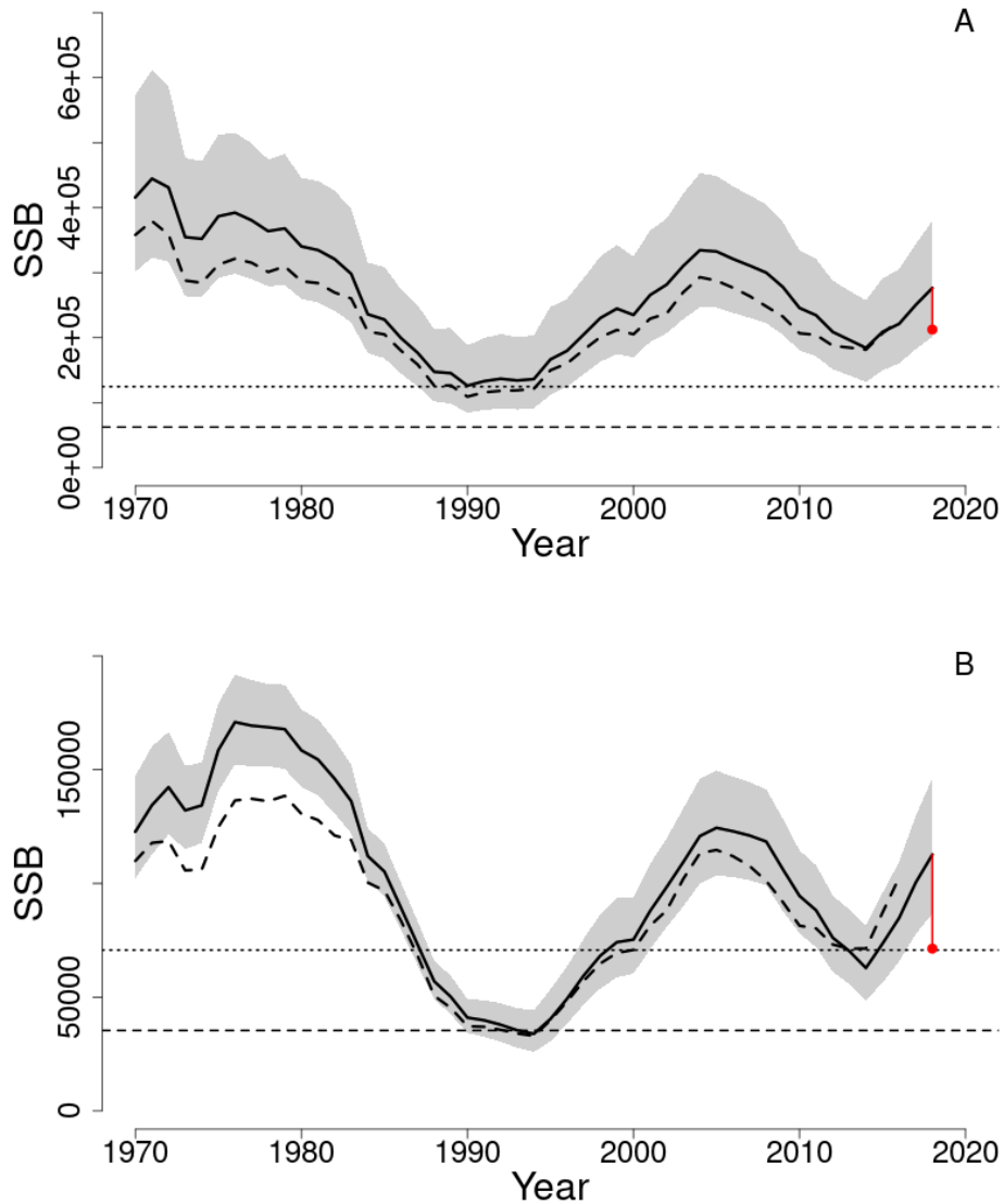
Figure 58: Estimated trends in the spawning stock biomass of pollock between 1970 and 2018 from the current (solid line) and previous (dashed line) assessment and the corresponding SSB_{Threshold} ( 0.5 * SSB_{MSY} proxy; horizontal dashed line) as well as SSB_{Target} ( SSB_{MSY} proxy; horizontal dotted line) based on the 2019 assessment models base (A) and flat sel sensitivity (B). Biomass was adjusted for a retrospective pattern and the adjustment is shown in red. The approximate 90% lognormal confidence intervals are shown.
