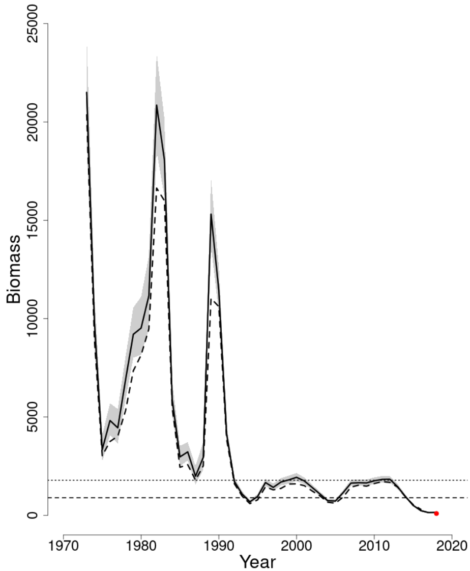
Figure 34: Trends in spawning stock biomass of Southern New England-Mid Atlantic yellowtail flounder between 1973 and 2018 from the current (solid line) and previous (dashed line) assessment and the corresponding SSB_{Threshold} ( \frac{1}{2} SSB_{MSY} proxy; horizontal dashed line) as well as SSB_{Target} ( SSB_{MSY} proxy; horizontal dotted line) based on the 2019 assessment. Biomass was adjusted for a retrospective pattern and the adjustment is shown in red. The approximate 90% lognormal confidence intervals are shown.
