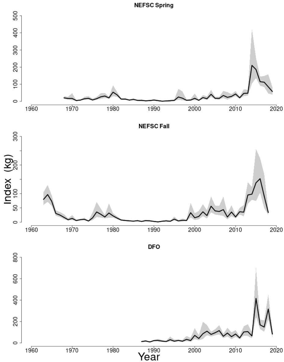
Figure 23: Indices of biomass (Mean kg/tow) for the Georges Bank haddock stock between 1963 and 2019 for the Northeast Fisheries Science Center (NEFSC) spring and fall bottom trawl surveys and the DFO winter bottom trawl survey. The approximate 90% lognormal confidence intervals are shown.
