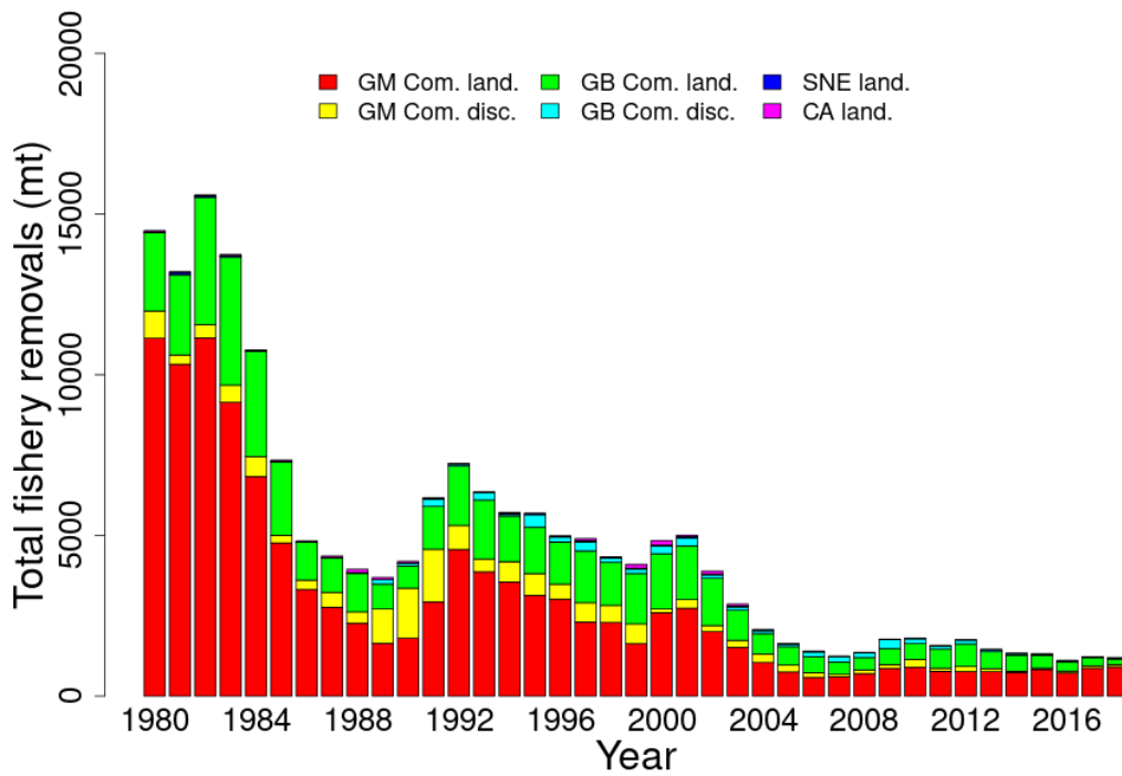
Figure 47: Total catch of Gulf of Maine-Georges Bank American plaice between 1980 and 2018 by fleet (Gulf of Maine, Georges Bank, Southern New England, and Canadian) and disposition (landings and discards).
