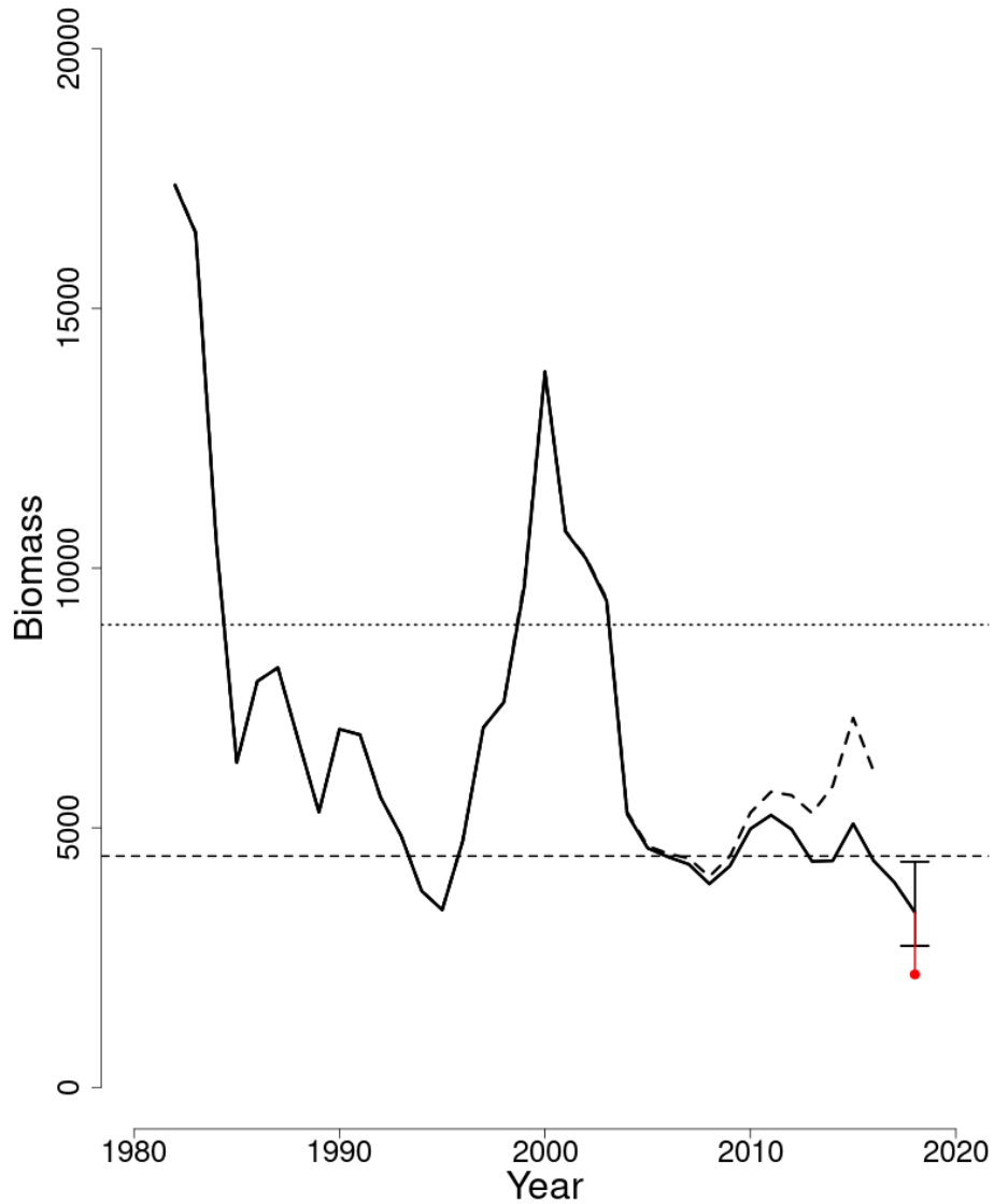
Figure 39: Trends in spawning stock biomass (mt) of Georges Bank Winter Flounder between 1982 and 2018 from the current (solid line) and previous (dashed line) assessments and the corresponding SSB_{Threshold} ( \frac{1}{2} SSB_{MSY} ; horizontal dashed line) as well as SSB_{Target} ( SSB_{MSY} ; horizontal dotted line) based on the 2019 assessment. Biomass was adjusted for a retrospective pattern and the adjustment is shown in red. The 90% normal confidence interval is shown for 2018.
