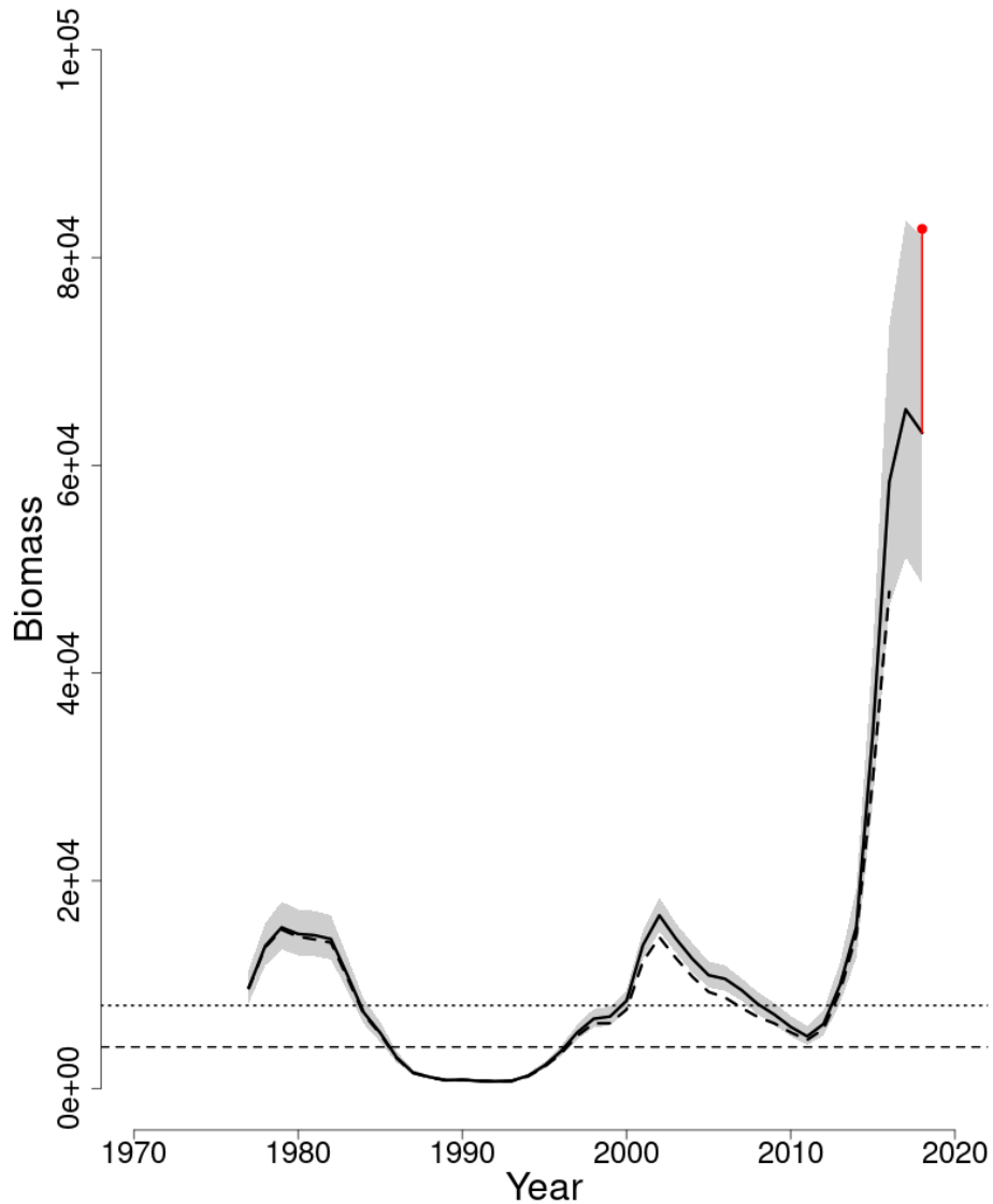
Figure 24: Trends in spawning stock biomass (SSB) of Gulf of Maine haddock between 1977 and 2018 from the current (solid line) and previous (dashed line) assessment and the corresponding SSB_{Threshold} ( \frac{1}{2} SSB_{MSY} proxy; horizontal dashed line) as well as SSB_{Target} ( SSB_{MSY} proxy; horizontal dotted line) based on the 2019 assessment. SSB was adjusted for a retrospective pattern and the adjustment is shown in red based on the 2019 assessment. The approximate 90% lognormal confidence intervals are shown.
