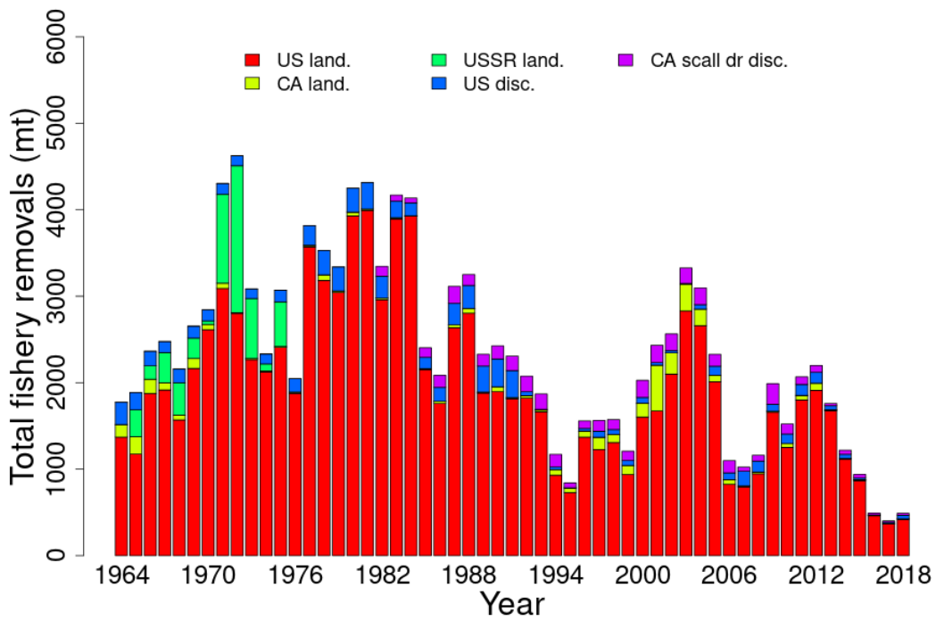
Figure 42: Total catches (mt) of Georges Bank Winter Flounder between 1982 and 2019 by country and disposition (landings and discards).
