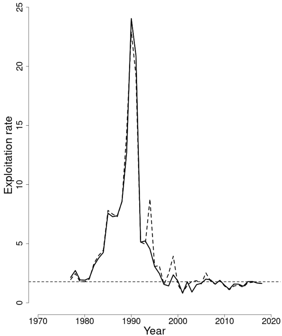
Figure 72: Trends in relative fishing mortality of southern New England - mid-Atlantic windowpane flounder between 1975 and 2018 from the current assessment using re-estimated discards (solid line), and the 2017 assessment (dashed line). The corresponding F_{MSY} proxy=1.78 is shown by the horizontal line.
