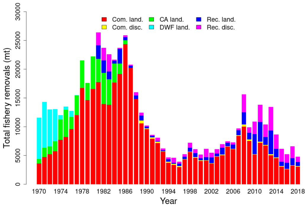
Figure 61: Total catch of pollock between 1970 and 2018 by fleet (commercial, Canadian, distant water fleet, and recreational) and disposition (landings and discards).
