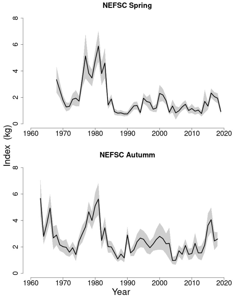
Figure 48: Indices of biomass for the Gulf of Maine-Georges Bank American plaice between 1963 and 2019 for the Northeast Fisheries Science Center (NEFSC) spring and autumn research bottom trawl surveys. The approximate 90% normal confidence intervals are shown.
