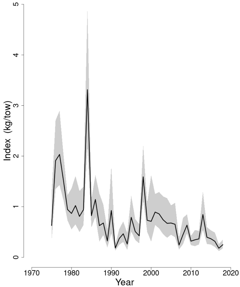
Figure 70: NEFSC fall bottom trawl survey indices in kg/tow for Gulf of Maine - Georges Bank windowpane flounder between 1975 and 2018. The approximate 90% lognormal confidence intervals are shown.
