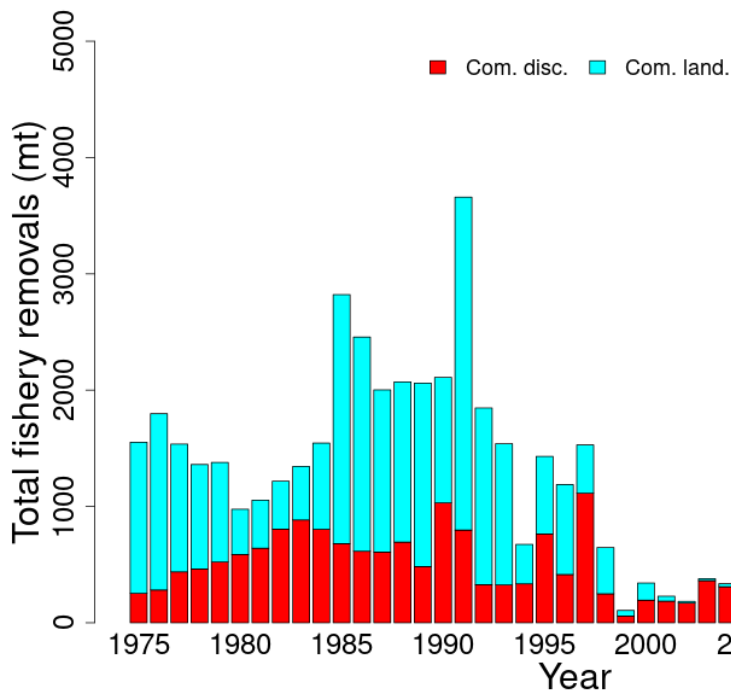
Figure 69: Total catch of Gulf of Maine - Georges Bank windowpane flounder between 1975 and 2018 by disposition (landings and discards).
