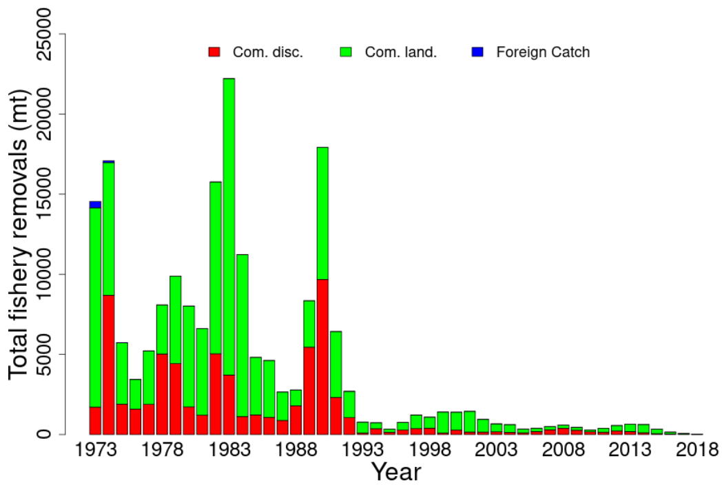
Figure 37: Total catch of Southern New England-Mid Atlantic yellowtail flounder between 1973 and 2018 by fleet (US domestic and foreign catch) and disposition (landings and discards).
