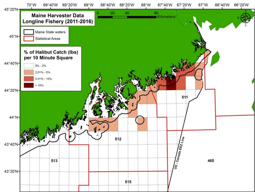
Figure 6. Proportion of longline halibut catch (catch weight in each 10 minute square/total halibut catch weight) reported in each 10 minute square between 2011 and 2016.
