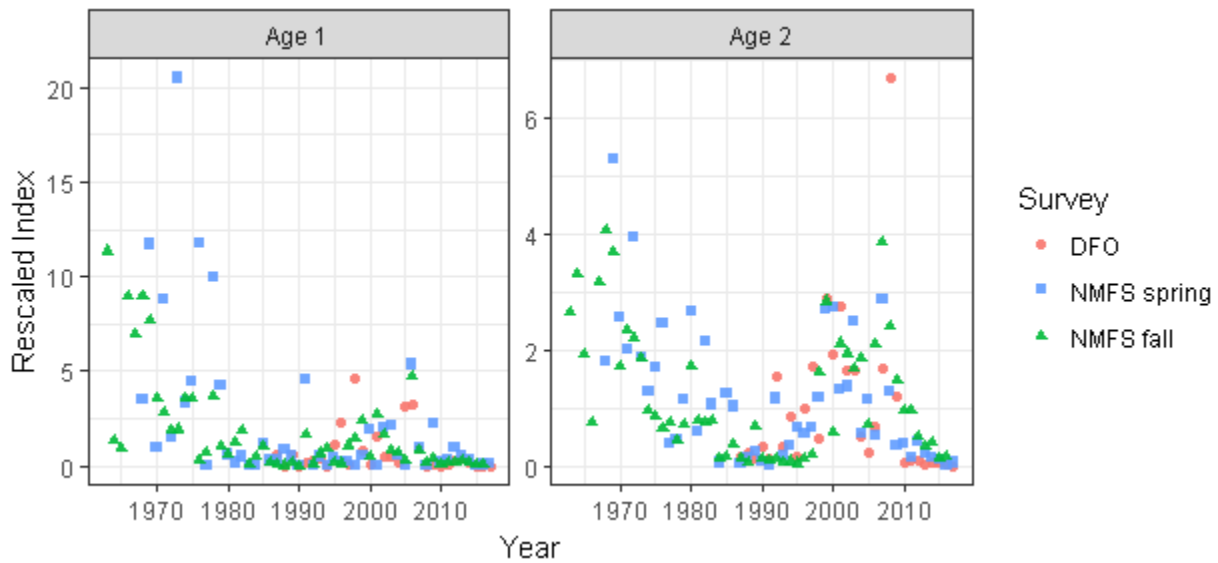
Figure 4. Estimates of recruitment (age 1 has many zeros, so age 2 also shown) from the three bottom trawl surveys standardized to their respective means during 1987 through 2007.
