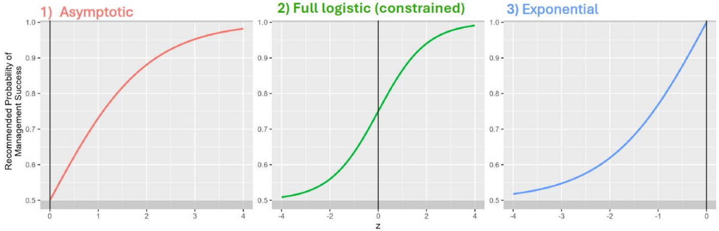
Figure 2. Three possible shapes for the Risk Policy curve including 1) an asymptotic curve, 2) a full logistic curve constrained between 0.5 and 1, and 3) an exponential curve.
