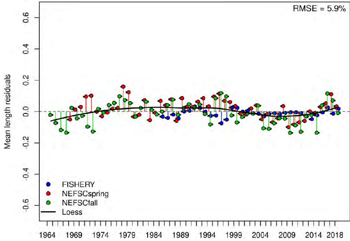
Figure 4.29. SS joint residual plot from fit to annual mean length from length composition data.
