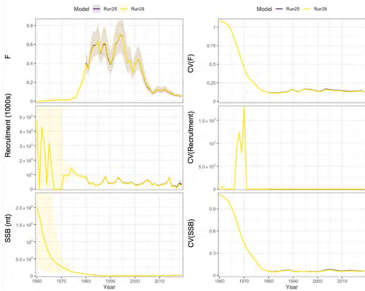
Figure 4.4: Model estimates of spawning stock biomass (SSB), fishing mortality (F) and recruitment (left), corresponding CVs around these estimates (right). Both run 25 and 28 implemented recruitment and selectivity random effects, with run 28 fit to catch data beginning in 1960 rather than in 1980 as in run 25.
