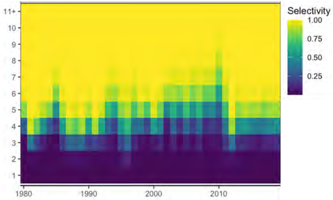
Figure 5.3. Estimates of fishery selectivity at age for American plaice from WHAM run 29F4.
