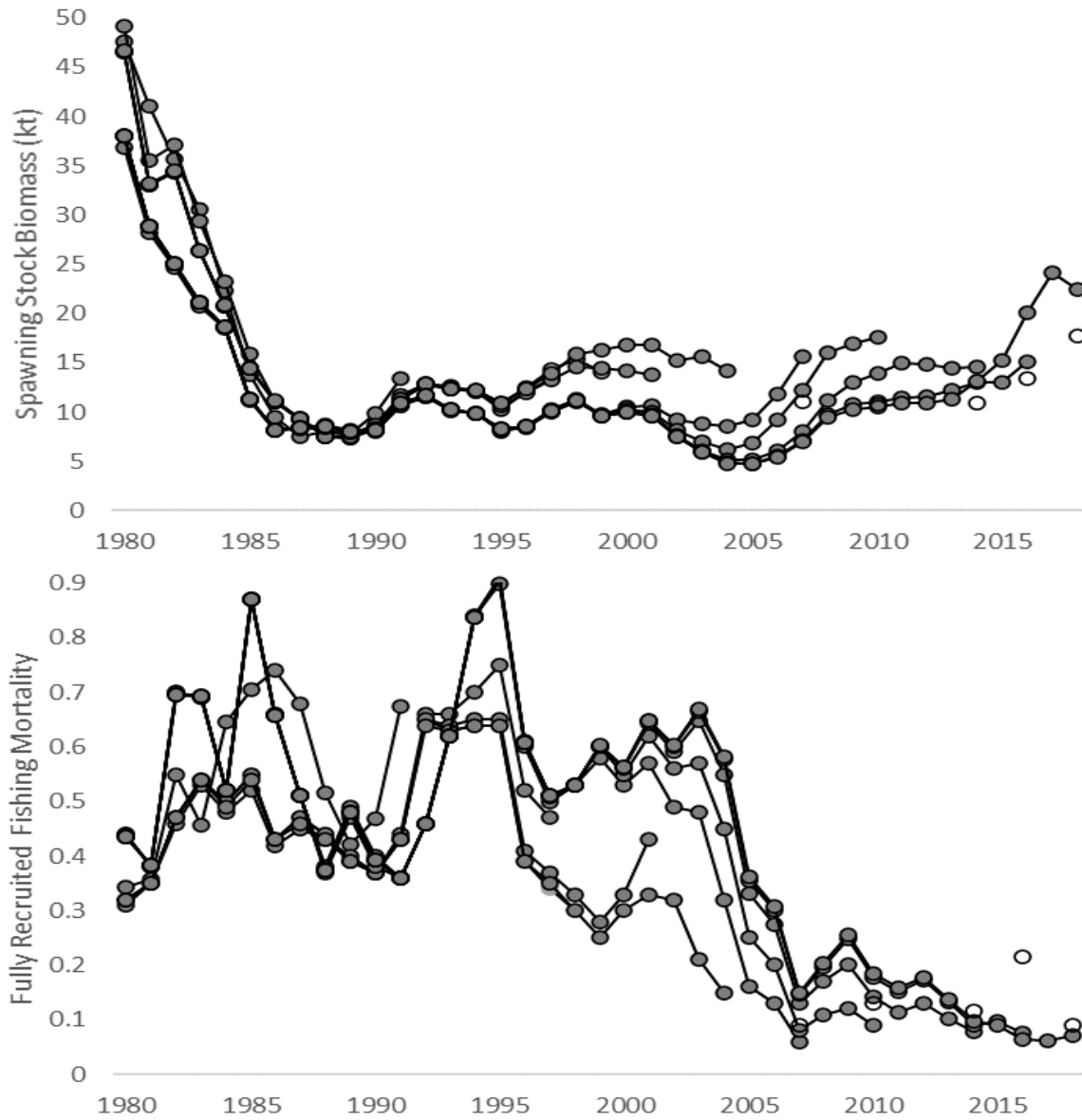
Figure 4. Estimates of spawning stock biomass (top) and fully-recruited fishing mortality (bottom) from the series of American plaice stock assessments. Open circles indicate retrospective-adjusted estimates.
