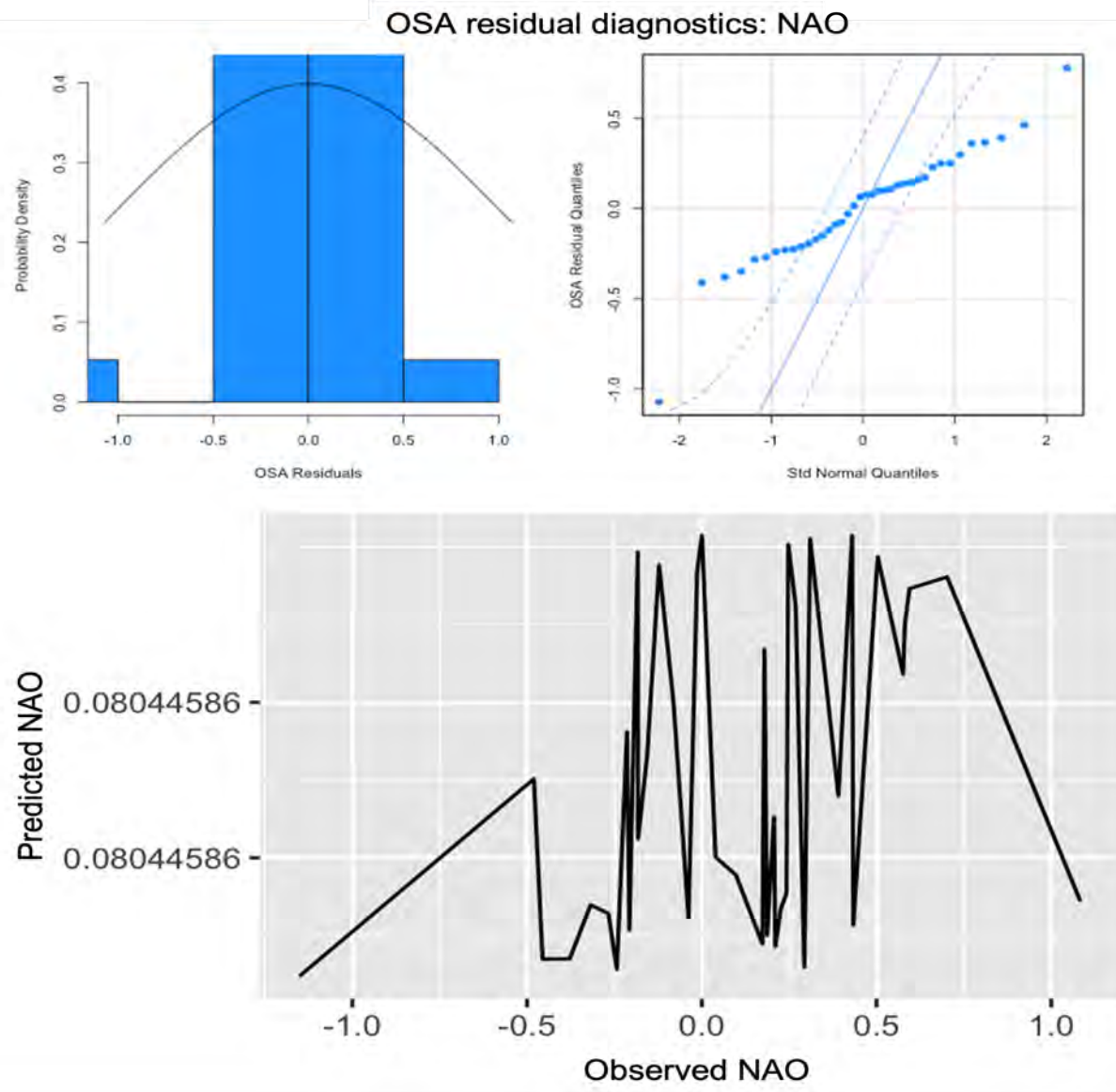
Figure 4.7: Example of over-dispersed one-step ahead (OSA) residuals for fit to a North Atlantic Oscillation (NAO) covariate (top) and comparison of model predicted values for this covariate vs. observed values for this covariate (bottom). Both results indicate a modeling error in WHAM when an model is fit to an environmental covariate without an effect on stock dynamics specified (i.e. to establish a base model that is comparable via AIC to runs with an effect specified) that was not resolved in this research track due to time constraints.
