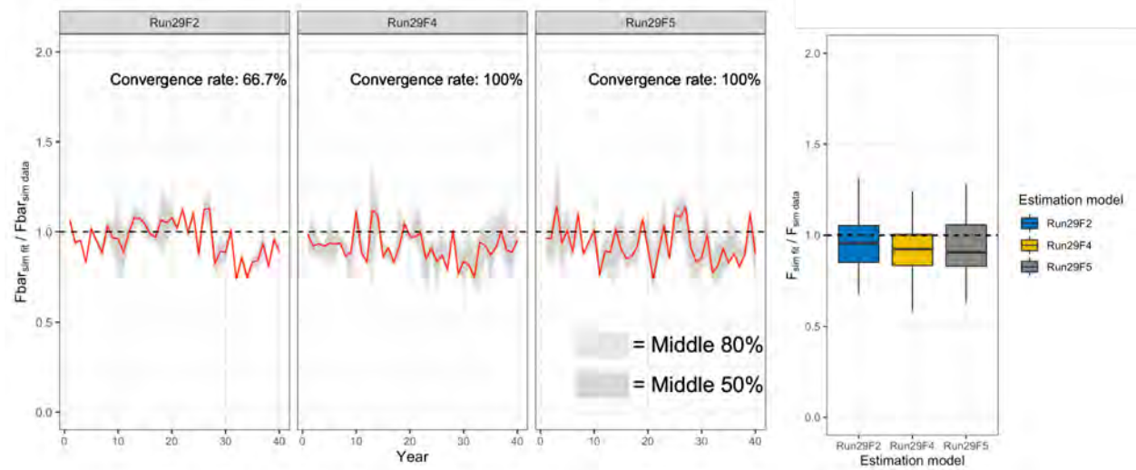
Figure 4.17: Fishing mortality ( F_{bar} ) relative error for candidate model self-tests over time (3 leftmost panels, median in red, middle 50% and 80% of simulations in dark gray and gray respectively). Boxplot of relative error aggregated across all simulations and years for each of the candidate models for each of the candidate models (rightmost panel).
