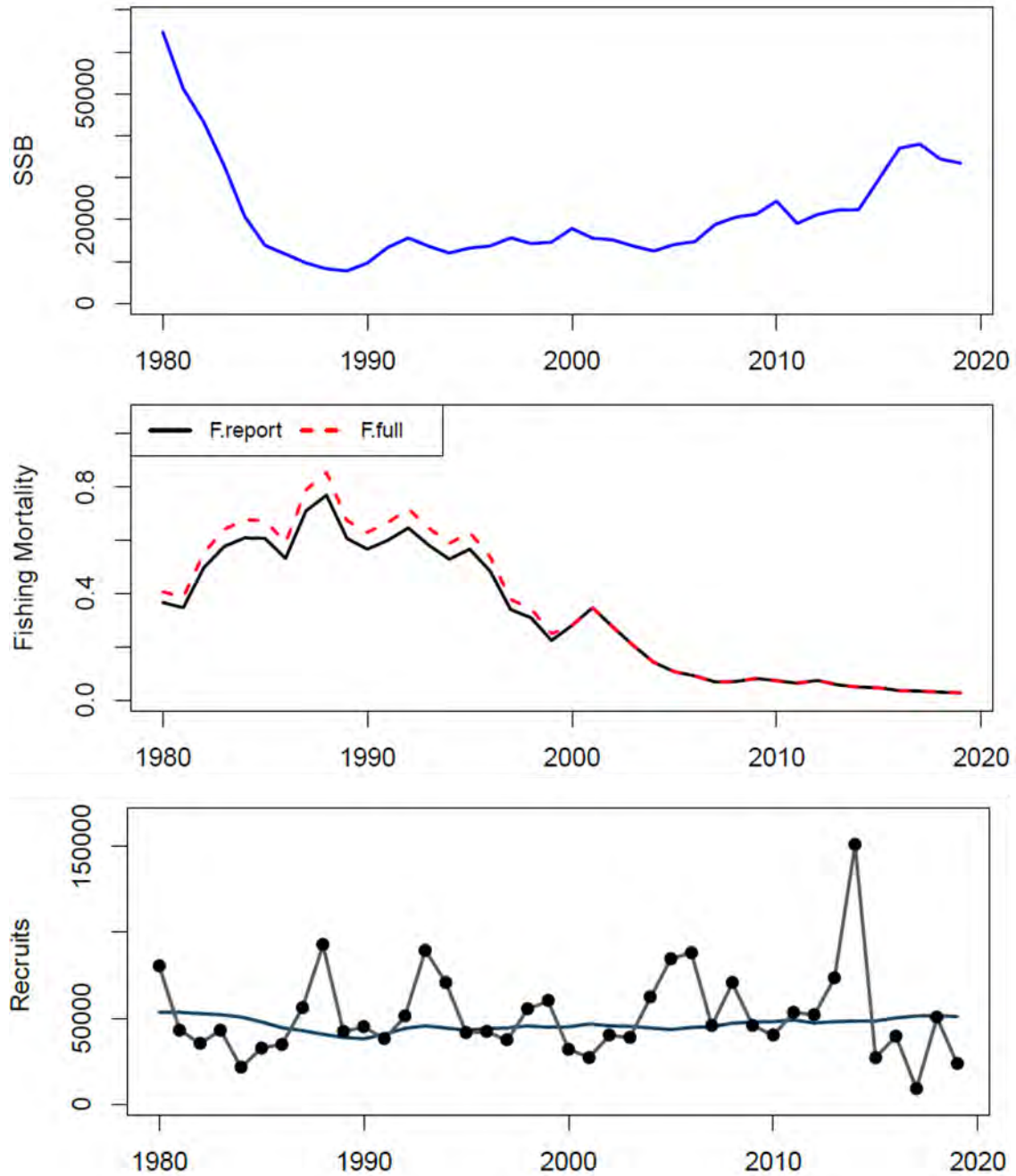
Figure 4.24: Estimates of American plaice spawning stock biomass (SSB, mt) and fishing mortality (F report : average of ages 6-9, and fully selected F) and age-1 recruitment (thousands) from ASAP run 43.
