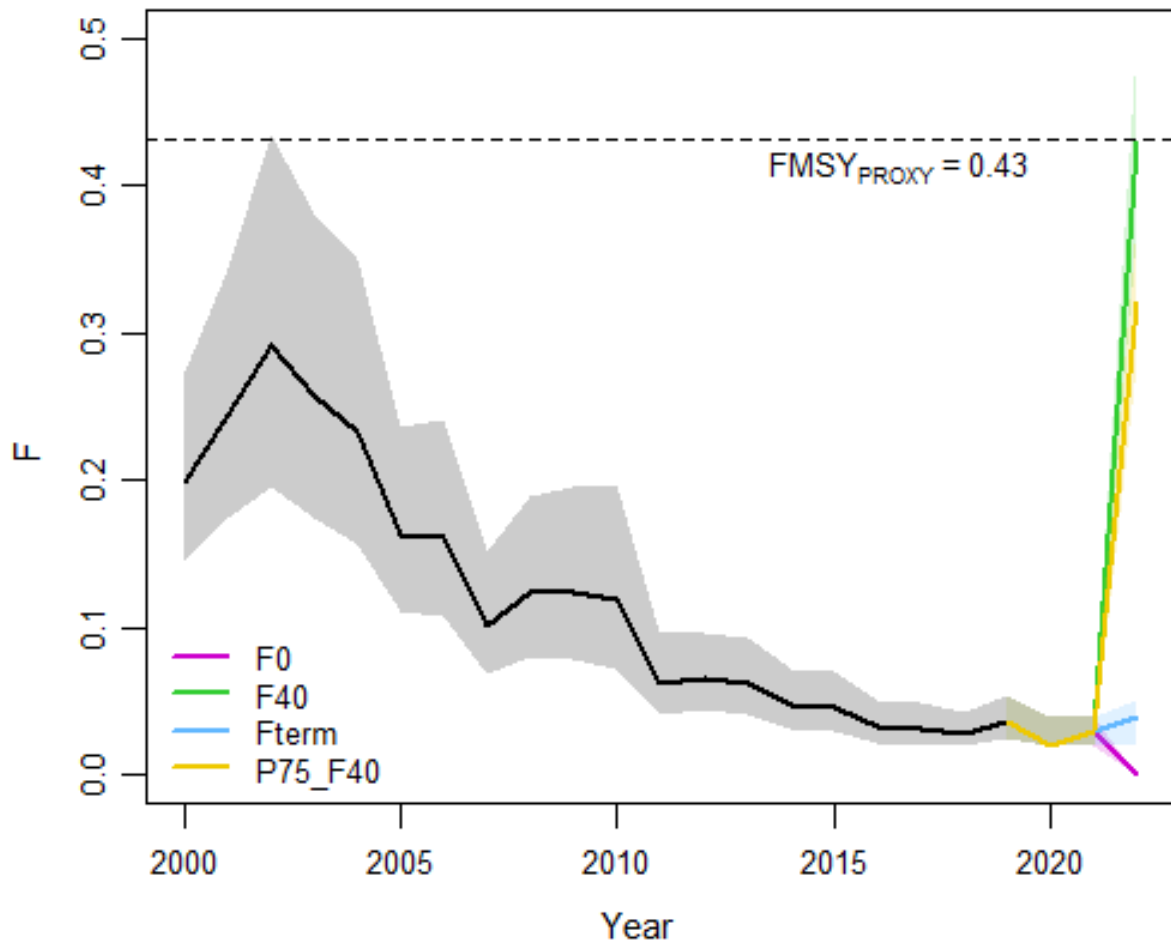
Figure 6.3. Projections of American fishing mortality expected from four scenarios of fishing in 2022 (F0: no fishing; F40: fishing at the F 40% ; Fterm: fishing at 2019 F; and P75_F40: fishing at 75% of F 40% ).
