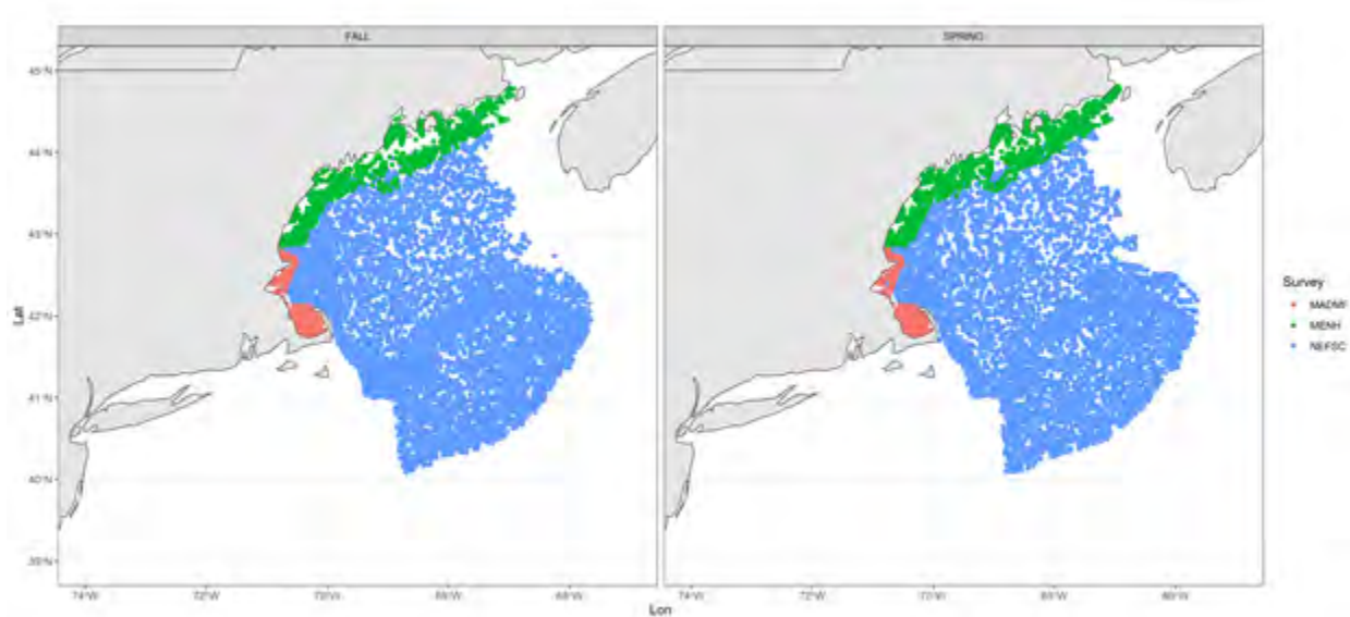
Figure 3.12. Tow locations for the three surveys used in VAST model for American plaice
