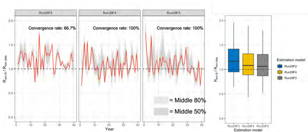
Figure 4.15: Recruitment (R) relative error for candidate model self-tests over time (3 leftmost panels, median in red, middle 50% and 80% of simulations in dark gray and gray respectively). Boxplot of relative error aggregated across all simulations and years for each of the candidate models (rightmost panel).
