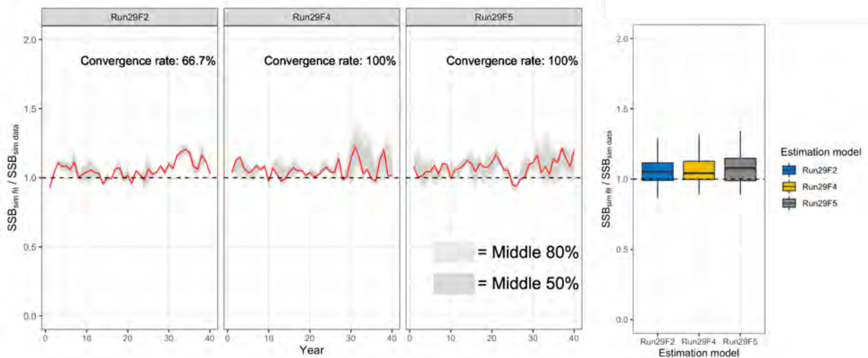
Figure 4.14: Spawning stock biomass (SSB) relative error for candidate model self-tests over time (3 leftmost panels, median in red, middle 50% and 80% of simulations in dark gray and gray)
