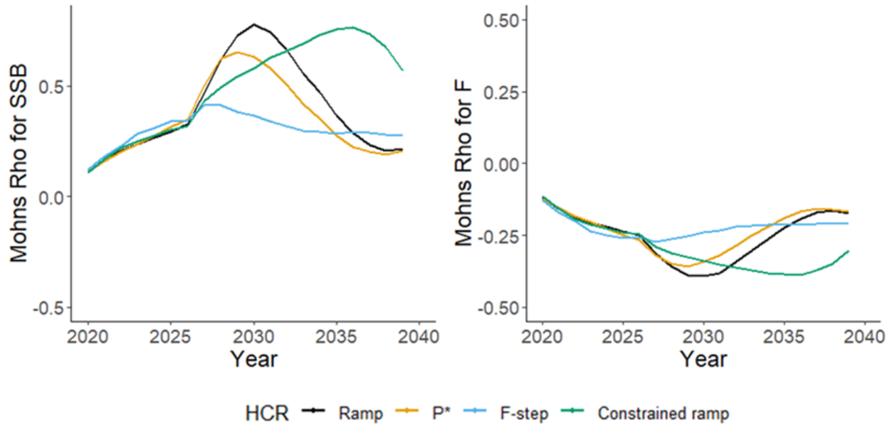
Figure 17. Mohn's Rho values for spawning stock biomass (SSB) and fishing mortality (F) for Gulf of Maine cod with a natural mortality stock assessment model misspecification (Overfished Mortality Misspecified Scenario).
