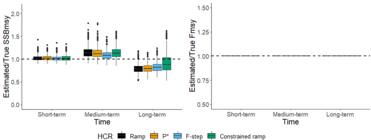
Figure 45. Median ratios of estimated to true stock biomass reference point ( SSB_{MSY} ) and fishing mortality biomass reference point ( F_{MSY} ) for Gulf of Maine cod with a stock assessment misspecification (Overfished Mortality and Recruitment Misspecification Scenario) and year one projection held constant (Projection sub-alternative b) in the short- (1-5 years), medium- (6-10 years), and long-term (11-21 years).
