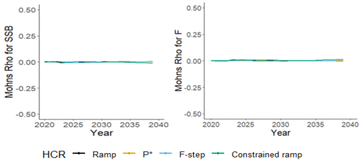
Figure 71. Mohn's Rho values for spawning stock biomass (SSB) and fishing mortality (F) for Georges Bank haddock with no stock assessment model misspecification (Base Case Not Overfished Scenario).
