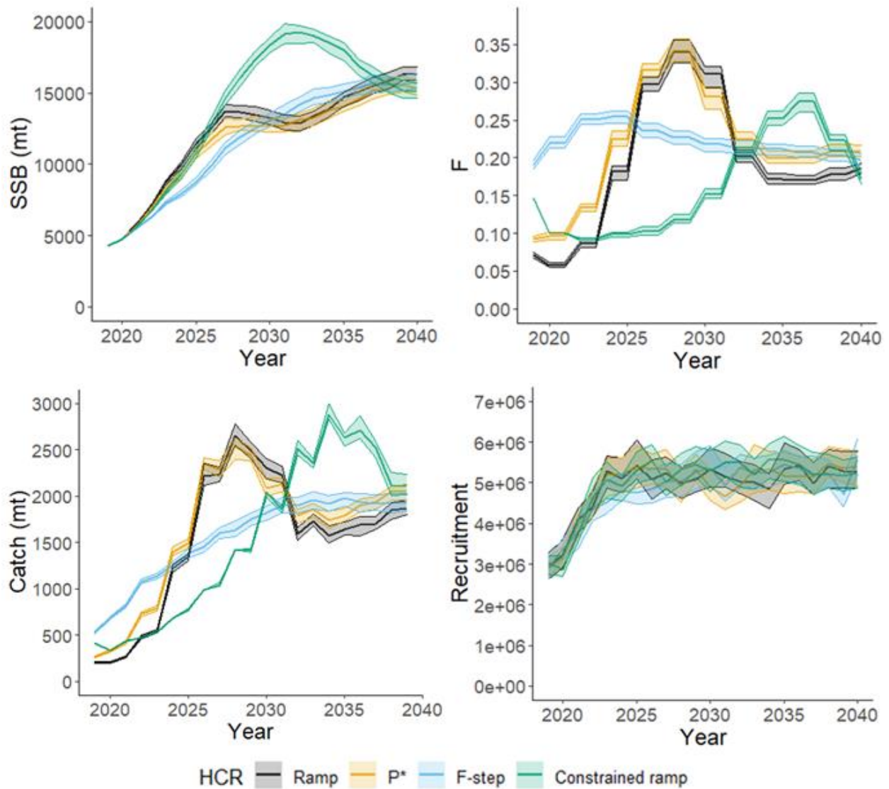
Figure 14. True operating model median spawning stock biomass (SSB), fishing mortality (F), catch (mt), and recruits with 95% confidence intervals for Gulf of Maine cod with a natural mortality stock assessment model misspecification (Overfished Mortality Misspecified Scenario) from 2019 to 2040.
