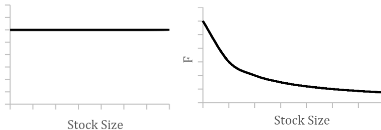
Figure B1. Constant catch harvest control rule.
