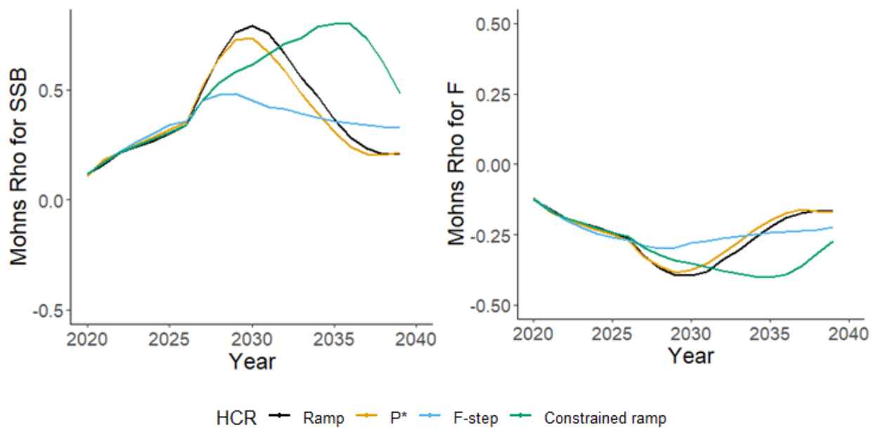
Figure 44. Mohn's Rho values for spawning stock biomass (SSB) and fishing mortality (F) for Gulf of Maine cod with a stock assessment misspecification (Overfished Mortality and Recruitment Misspecification Scenario) and year one projection held constant (Projection sub-alternative b).
