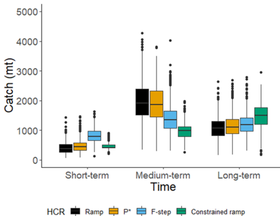
Figure 33. True median catch for Gulf of Maine cod with a natural mortality and recruitment stock assessment model misspecification (Overfished Mortality and Recruitment Misspecified Scenario) in the short- (1-5 years), medium- (6-10 years), and long-term (11-21 years).
