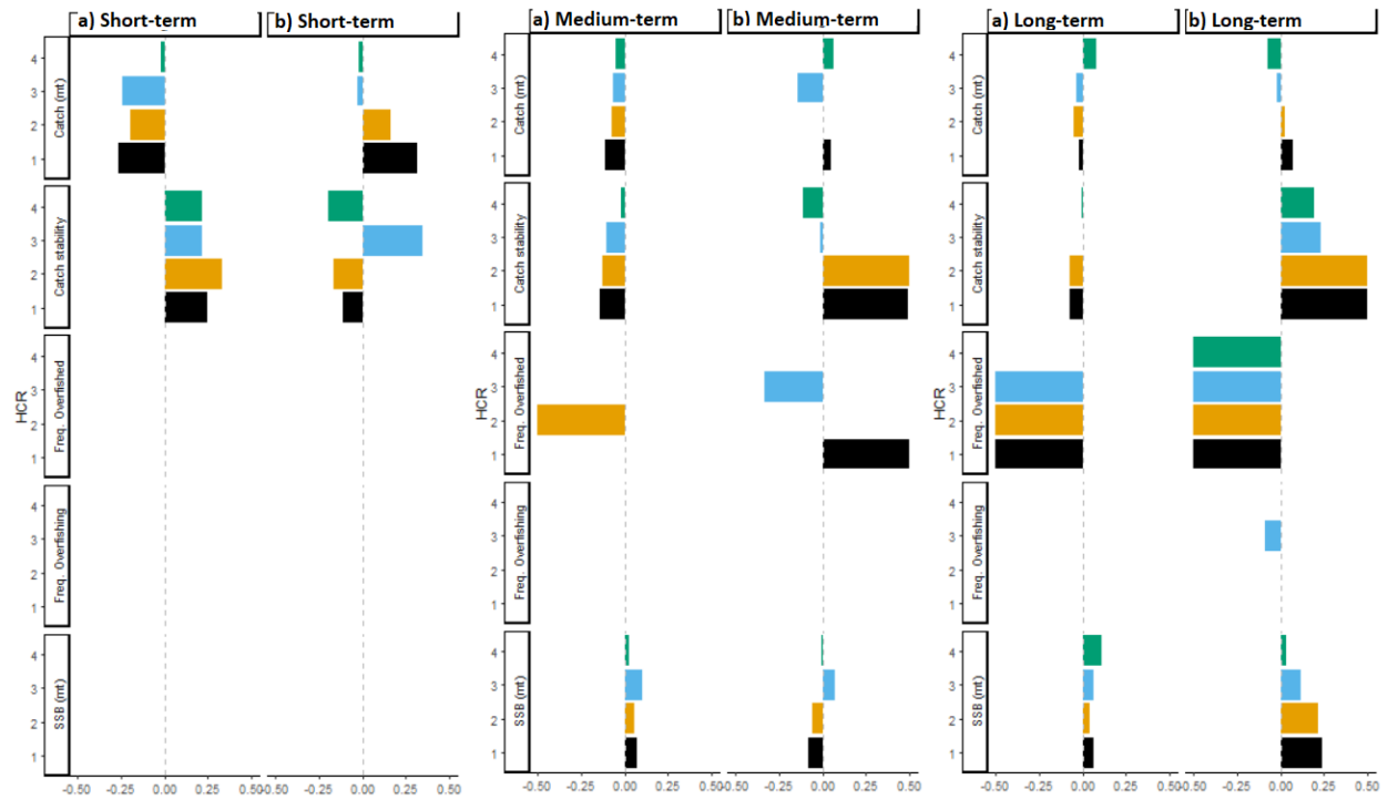
Figure 88. Short- (1-5 years), medium- (6-10 years), and long-term (11-21 years) relative difference in harvest control rule performance with the Overfished Mortality and Recruitment Misspecified Scenario with catch advice based on two-year projections and a) catch advice based on year one projection held constant and b) annual stock assessment updates.
