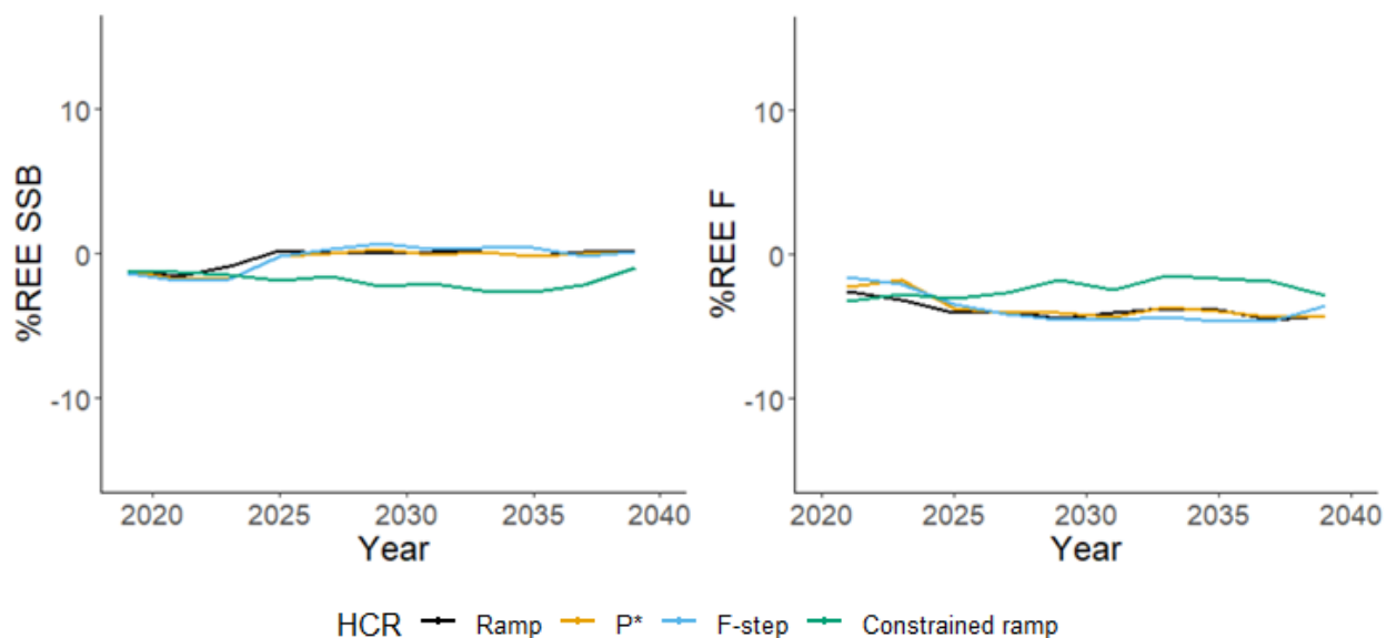
Figure 70. Percent relative error (REE) in terminal estimated spawning stock biomass (SSB) and fishing mortality (F) for Georges Bank haddock with no stock assessment model misspecification (Base Case Not Overfished Scenario).
