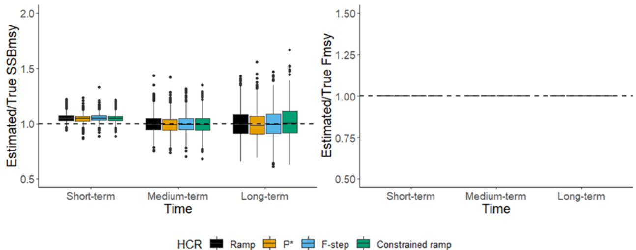
Figure 9. Median ratios of estimated to true stock biomass reference point ( SSB_{MSY} ) and fishing mortality biomass reference point ( F_{MSY} ) for Gulf of Maine cod with no stock assessment model misspecification (Base Case Overfished Scenario) in the short- (1-5 years), medium- (6-10 years), and long-term (11-21 years).
