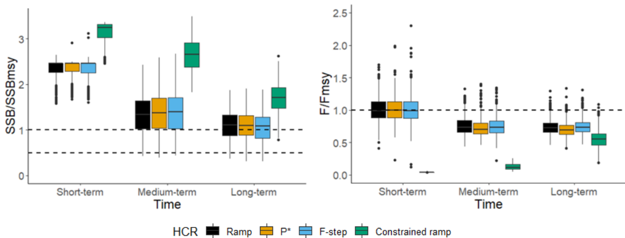
Figure 74. True median ratios of spawning stock biomass to the spawning stock biomass reference point ( SSB/SSB_{MSY} ) and fishing mortality to the fishing mortality biomass reference point ( F/F_{MSY} ) for Georges Bank haddock with no stock assessment model misspecification (Base Case Not Overfished Scenario) in the short- (1-5 years), medium- (6-10 years), and long-term (11-21 years).
