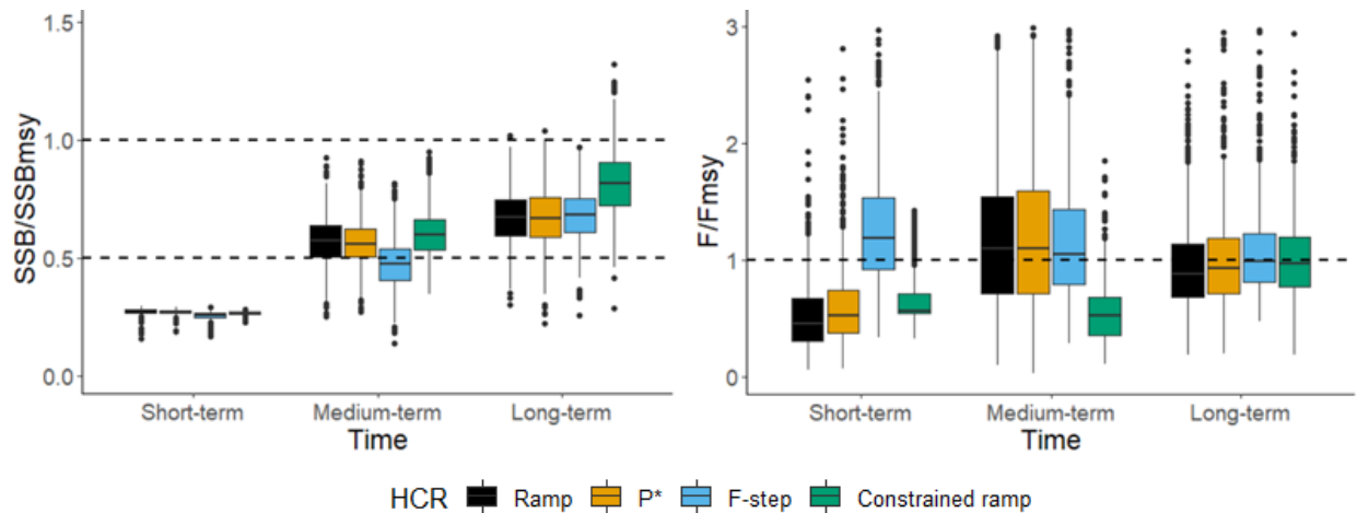
Figure 56. True median ratios of spawning stock biomass to the spawning stock biomass reference point ( SSB/SSB_{MSY} ) and fishing mortality to the fishing mortality biomass reference point ( F/F_{MSY} ) for Gulf of Maine cod with a natural mortality stock assessment model misspecification (Overfished Mortality and Recruitment Misspecified Scenario) and a rho-adjustment (Rho Scenario 1) in the short- (1-5 years), medium- (6-10 years), and long-term (11-21 years).
