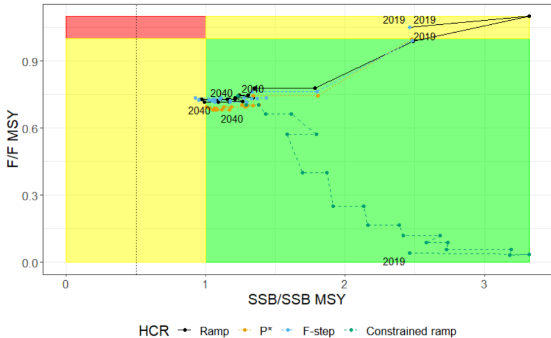
Figure 73. True stock status trajectories (ratio of fishing mortality over fishing mortality reference point ( F/F_{MSY} ) versus ratio of spawning stock biomass over spawning stock biomass reference point ( SSB/SSB_{MSY} ) for Georges Bank haddock with a no stock assessment model misspecification (Base Case Not Overfished Scenario). The dashed line represents the overfished threshold.
