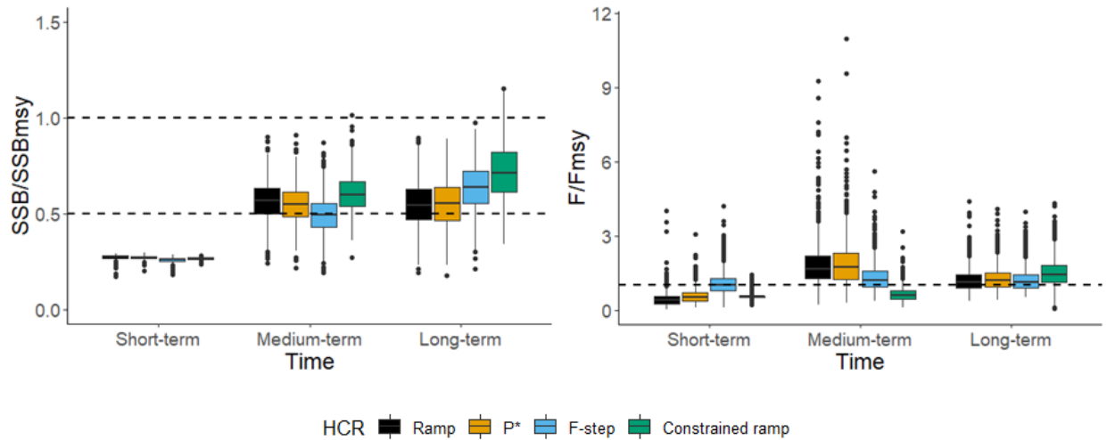
Figure 47. True median ratios of spawning stock biomass to the spawning stock biomass reference point ( SSB/SSB_{MSY} ) and fishing mortality to the fishing mortality biomass reference point ( F/F_{MSY} ) for Gulf of Maine cod with a stock assessment misspecification (Overfished Mortality and Recruitment Misspecification Scenario) and year one projection held constant (Projection sub-alternative b) in the short- (1-5 years), medium- (6-10 years), and long-term (11-21 years).
