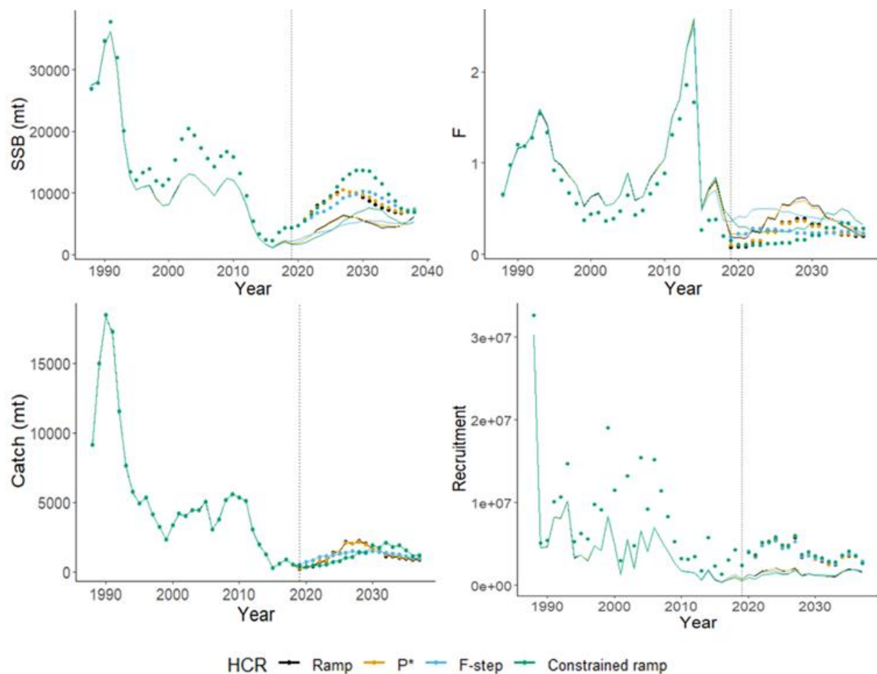
Figure 31. True operating model (closed circles) and estimated stock assessment values from the terminal assessment (stock assessment completed in 2039 with a terminal year of 2038; lines) of spawning stock biomass (SSB), fishing mortality (F), catch (mt), and recruits for Gulf of Maine cod with a natural mortality and recruitment stock assessment model misspecification (Overfished Mortality and Recruitment Misspecified Scenario) from 1982 to 2038 for SSB and 2037 for other metrics. The dashed line represents the beginning of the management procedure period (2019).
