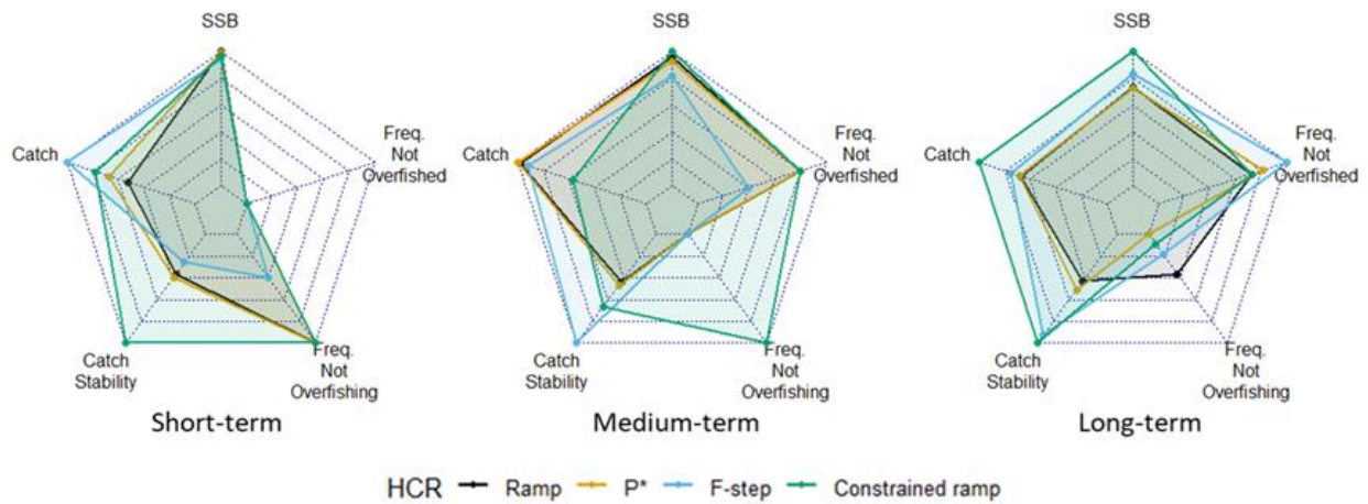
Figure 48. Harvest control rule (HCR) performance for Gulf of Maine cod with a stock assessment misspecification (Overfished Mortality and Recruitment Misspecification Scenario) and year one projection held constant (Projection sub-alternative b) in the short- (1-5 years), medium- (6-10 years), and long-term (11-21 years). Metrics are standardized to the maximum value for each metric attained by the different HCRs and equally weighted. Spawning stock biomass (SSB) and catch are median SSB and catch for the time period.
