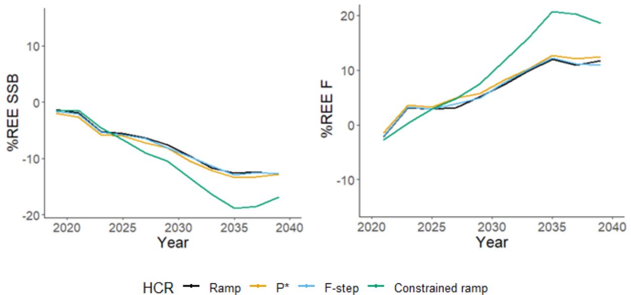
Figure 79. Percent relative error (REE) in terminal estimated spawning stock biomass (SSB) and fishing mortality (F) for Georges Bank haddock with a survey catchability stock assessment model misspecification (Not Overfished Catchability Misspecified Scenario).
