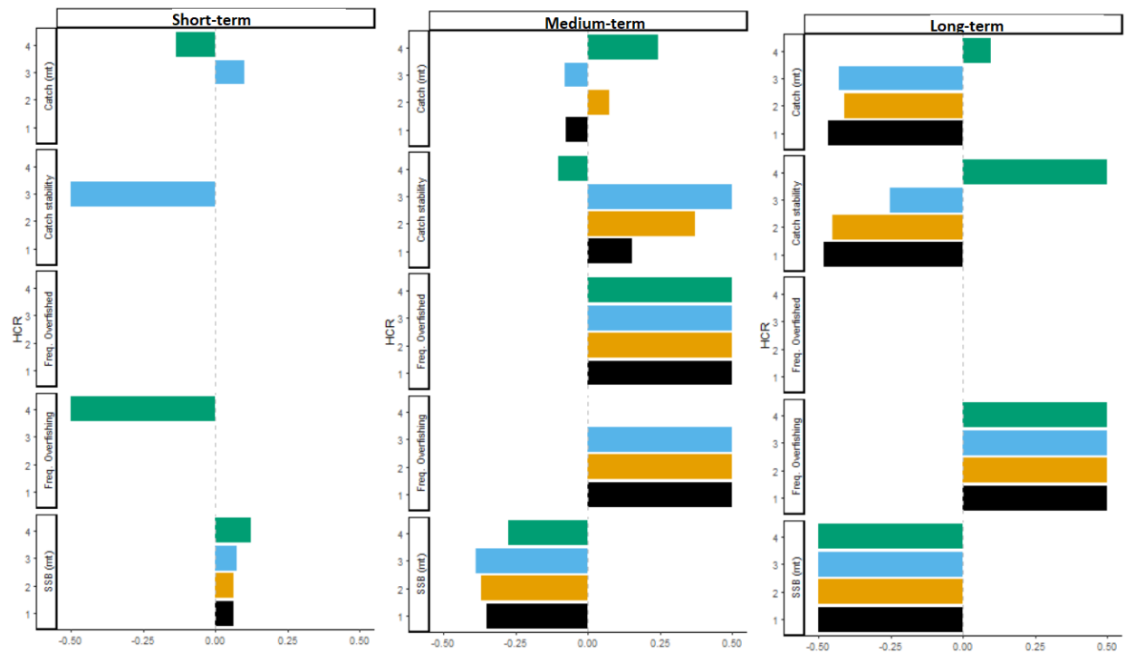
Figure 85. Short- (1-5 years), medium- (6-10 years), and long-term (11-21 years) relative difference in harvest control rule performance between the Base Case Overfished Scenario and the Overfished Mortality Misspecified Scenario.
