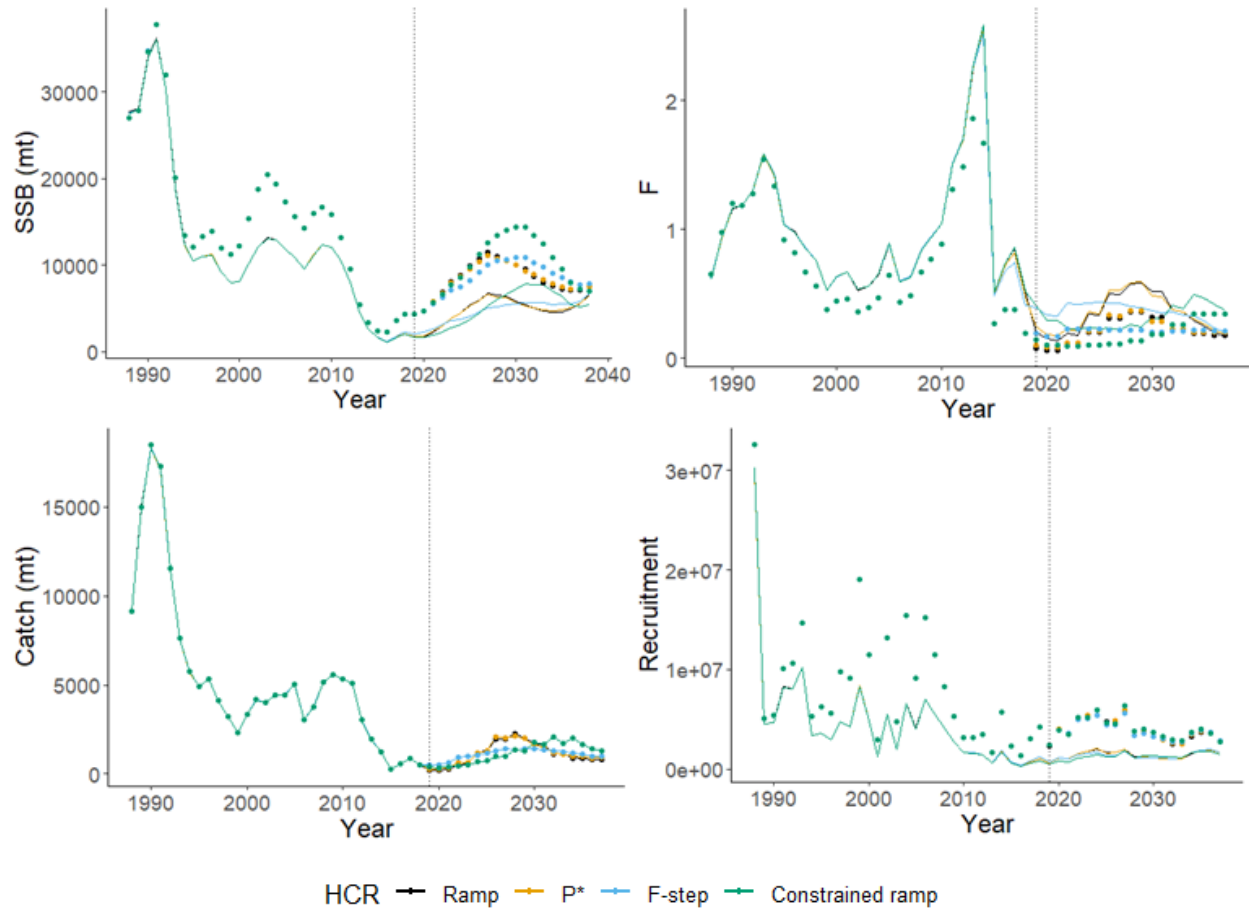
Figure 40. True operating model (closed circles) and estimated stock assessment values from the terminal assessment (stock assessment completed in 2039 with a terminal year of 2038; lines) of spawning stock biomass (SSB), fishing mortality (F), catch (mt), and recruits for Gulf of Maine cod with a stock assessment misspecification (Overfished Mortality and Recruitment Misspecification Scenario) and year one projection held constant (Projection Sub-alternative b) from 1982 to 2038 for SSB and 2037 for other metrics. The dashed line represents the beginning of the management procedure period (2019).
