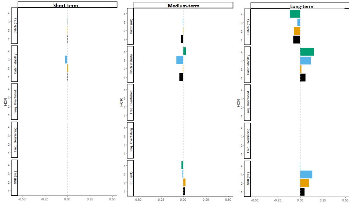
Figure 89. Short- (1-5 years), medium- (6-10 years), and long-term (11-21 years) relative difference in harvest control rule performance between the Base Case Not Overfished Scenario and the Not Overfished Catchability Misspecified Scenario.
