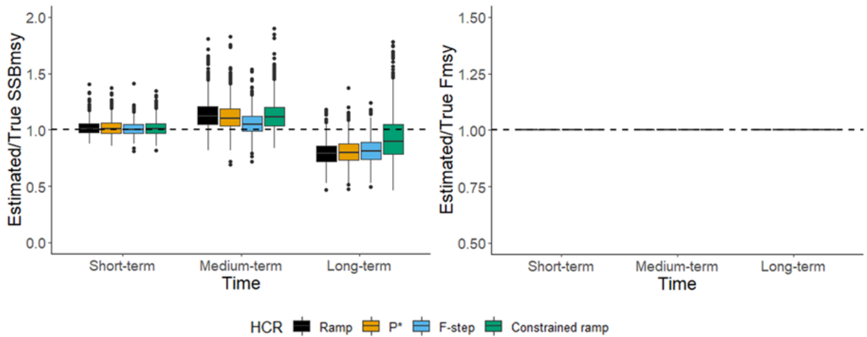
Figure 18. Median ratios of estimated to true stock biomass reference point ( SSB_{MSY} ) and fishing mortality biomass reference point ( F_{MSY} ) for Gulf of Maine cod with a natural mortality stock assessment model misspecification (Overfished Mortality Misspecified Scenario) in the short- (1-5 years), medium- (6-10 years), and long-term (11-21 years).
