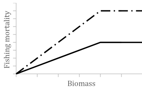
Figure 7. Harvest control rule with target (solid line) and limit (dashed line) fishing mortality reference points
