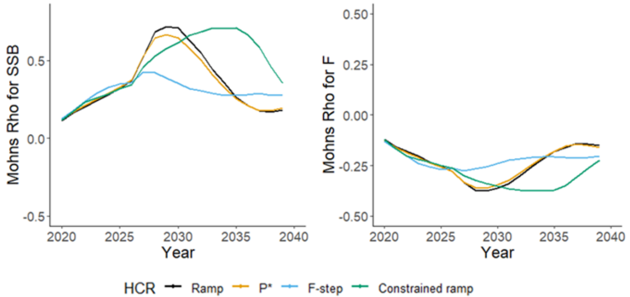
Figure 35. Mohn's Rho values for spawning stock biomass (SSB) and fishing mortality (F) for Gulf of Maine cod with a natural mortality and recruitment stock assessment model misspecification (Overfished Mortality and Recruitment Misspecified Scenario).
