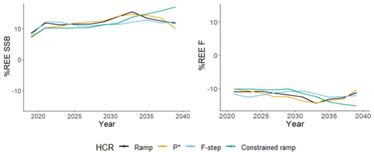
Figure 25. Percent relative error (REE) in terminal estimated spawning stock biomass (SSB) and fishing mortality (F) for Gulf of Maine cod with a recruitment stock assessment model misspecification (Overfished Recruitment Misspecified Scenario).
