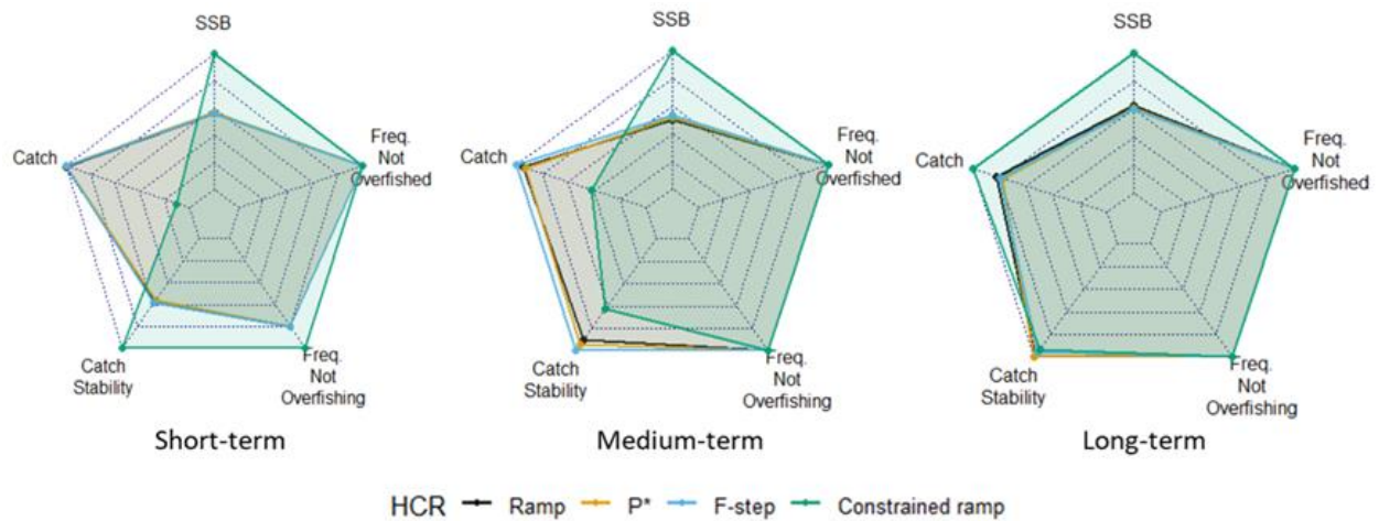
Figure 75. Harvest control rule (HCR) performance for Georges Bank haddock with no stock assessment model misspecification (Base Case Not Overfished Scenario) in the short- (1-5 years), medium- (6-10 years), and long-term (10-20 years). Metrics are standardized to the maximum value for each metric attained by the different HCRs and equally weighted. Spawning stock biomass (SSB) and catch are median SSB and catch for the time period.
