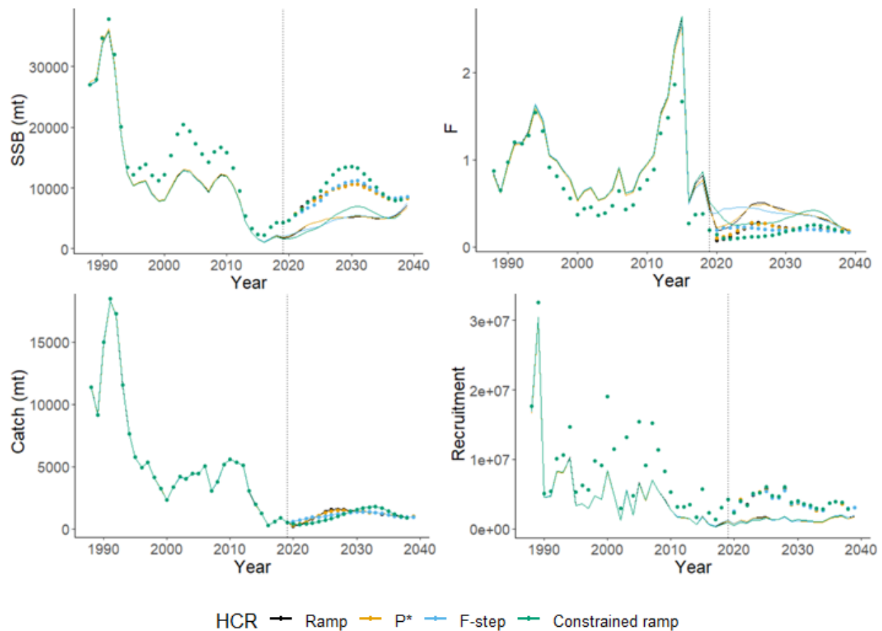
Figure 58. True operating model (closed circles) and estimated stock assessment values from the terminal assessment (stock assessment completed in 2039 with a terminal year of 2038; lines) of spawning stock biomass (SSB), fishing mortality (F), catch (mt), and recruits for Gulf of Maine cod with a natural mortality stock assessment model misspecification (Overfished Mortality and Recruitment Misspecified Scenario) and annual stock assessment updates (Frequency Scenario 2) from 1982 to 2038 for SSB and 2037 for other metrics. The dashed line represents the beginning of the management procedure period (2019).
