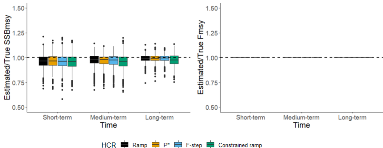
Figure 72. Median ratios of estimated to true ratios of the stock biomass reference point ( SSB_{MSY} ) and fishing mortality biomass reference point ( F_{MSY} ) for a stock originally not undergoing overfishing and not overfished (Georges Bank haddock) with no stock assessment model misspecification (Base Case Not Overfished Scenario) in the short- (1-5 years), medium- (5-10 years), and long-term (10-20 years).
