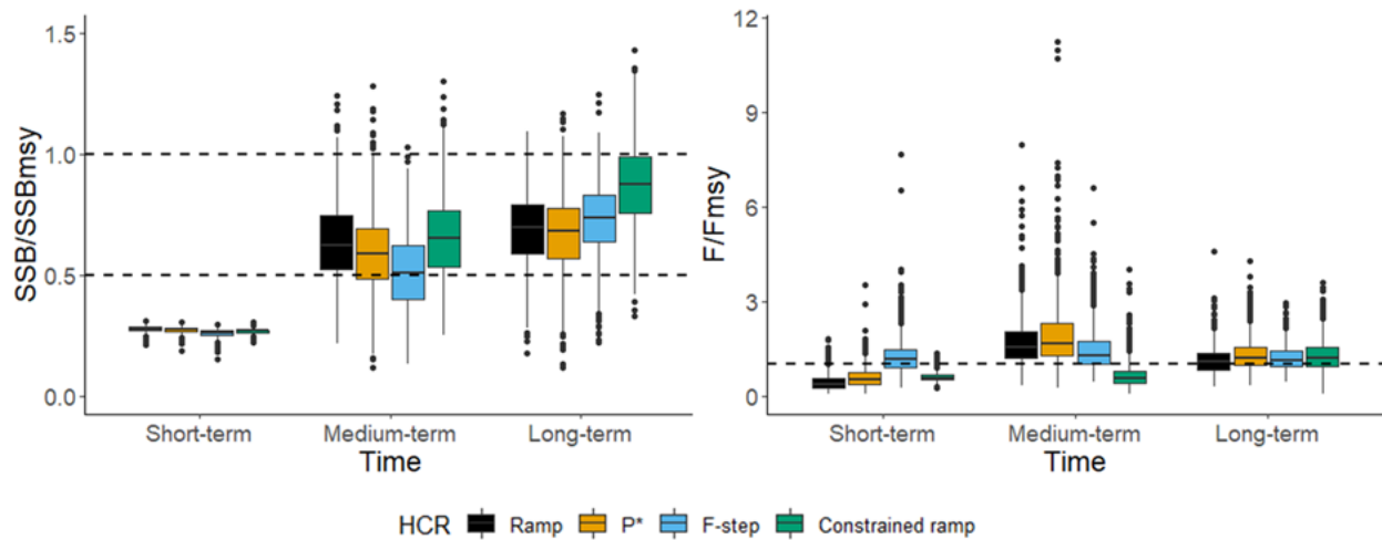
Figure 20. True median ratios of spawning stock biomass to the spawning stock biomass reference point ( SSB/SSB_{MSY} ) and fishing mortality to the fishing mortality biomass reference point ( F/F_{MSY} ) for Gulf of Maine cod with a natural mortality stock assessment model misspecification (Overfished Mortality Misspecified Scenario) in the short- (1-5 years), medium- (5-10 years), and long-term (10-20 years).
