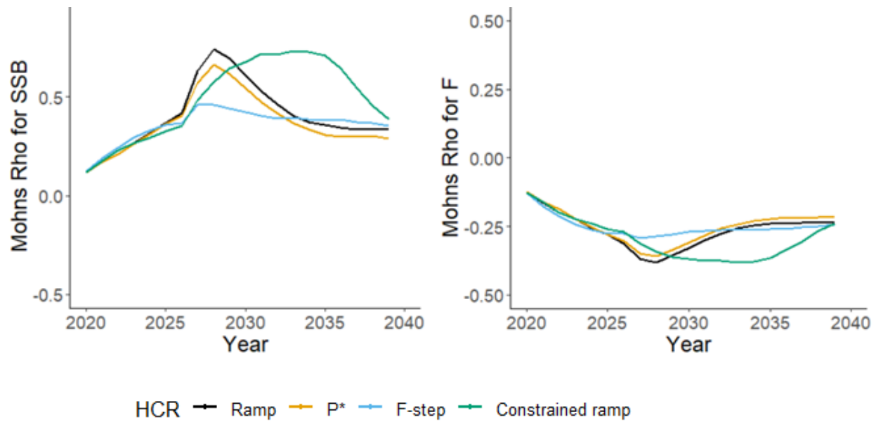
Figure 62. Mohn's Rho values for spawning stock biomass (SSB) and fishing mortality (F) for Gulf of Maine cod with a natural mortality stock assessment model misspecification (Overfished Mortality and Recruitment Misspecified Scenario) and annual stock assessment updates (Frequency Scenario 2).
