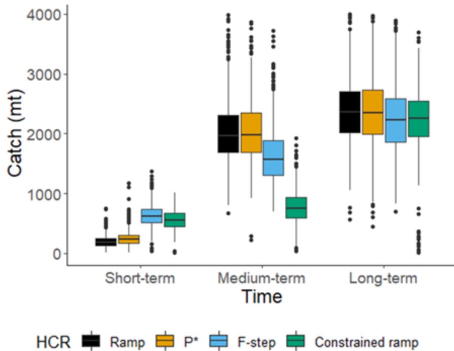
Figure 24. True median catch for Gulf of Maine cod with a recruitment stock assessment model misspecification (Overfished Recruitment Misspecified Scenario) in the short- (1-5 years), medium- (5-10 years), and long-term (10-20 years).
