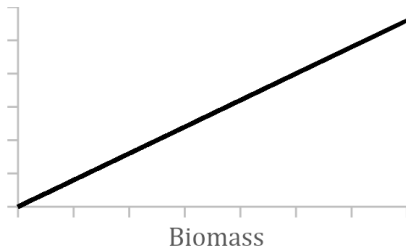
Figure B3. Constant fishing mortality harvest control rule.
