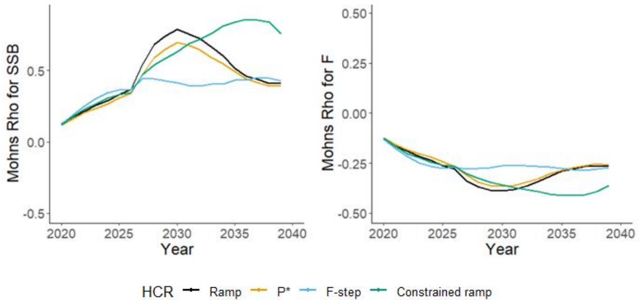
Figure 53. Mohn's Rho values for spawning stock biomass (SSB) and fishing mortality (F) for Gulf of Maine cod with a stock assessment model misspecification (Overfished Mortality and Recruitment Misspecified Scenario) and a rho-adjustment (Rho Scenario 1).
