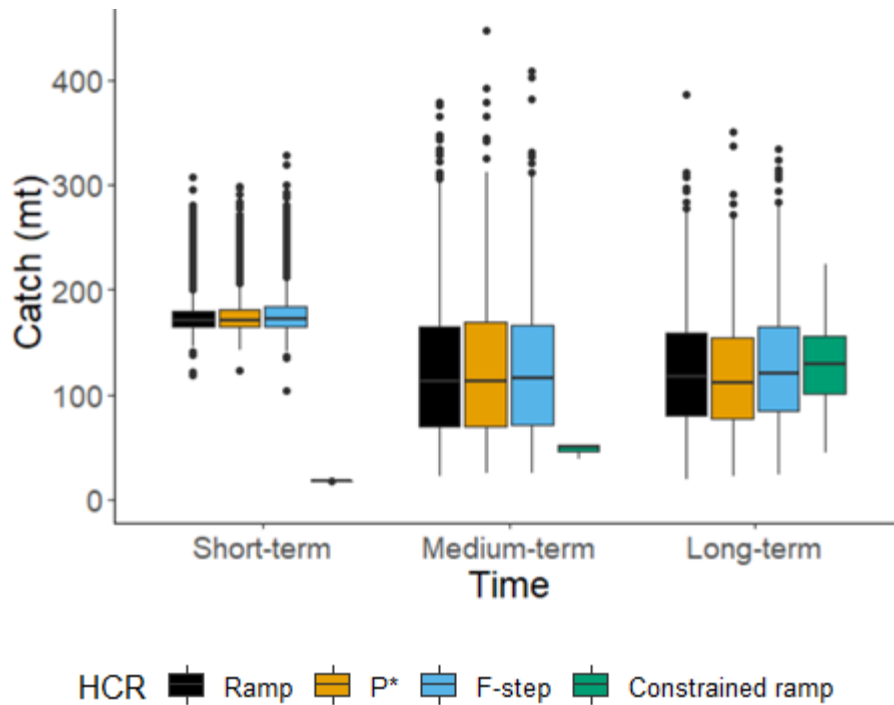
Figure 78. True median catch for Georges Bank haddock with a survey catchability stock assessment model misspecification (Not Overfished Misspecified Scenario) in the short- (1-5 years), medium- (6-10 years), and long-term (11-21 years).
