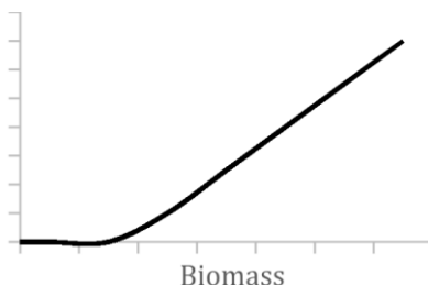
Figure B2. Constant escapement harvest control rule.
