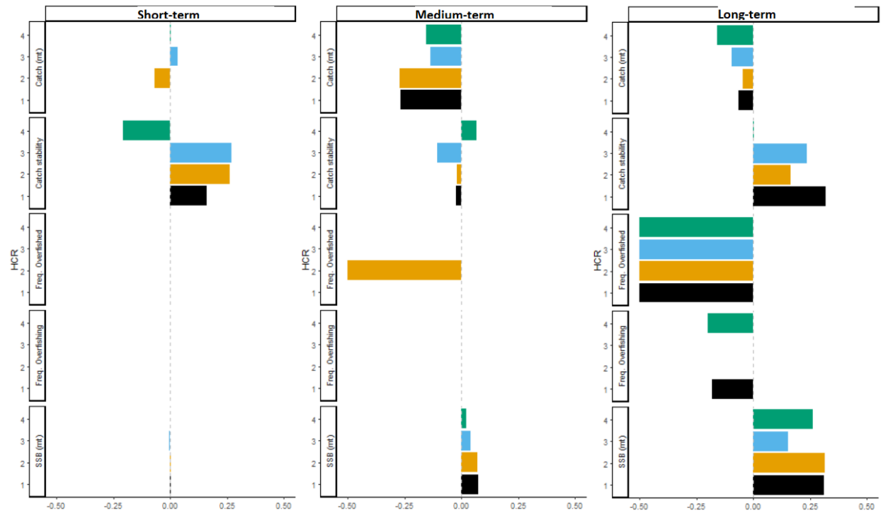
Figure 90. Short- (1-5 years), medium- (6-10 years), and long-term (11-21 years) relative difference in harvest control rule performance with the Overfished Mortality and Recruitment Misspecified Scenario without and with rho-adjustments.
