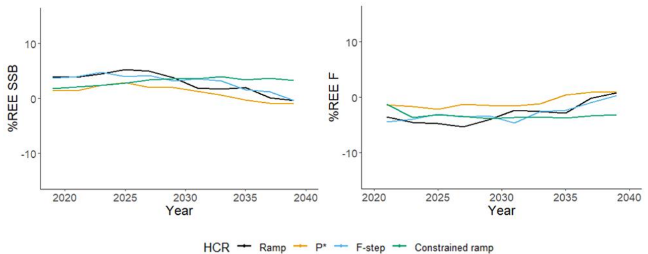
Figure 7. Percent relative error (REE) in terminal estimated spawning stock biomass (SSB) and fishing mortality (F) for Gulf of Maine cod with no stock assessment model misspecification (Base Case Overfished Scenario).
