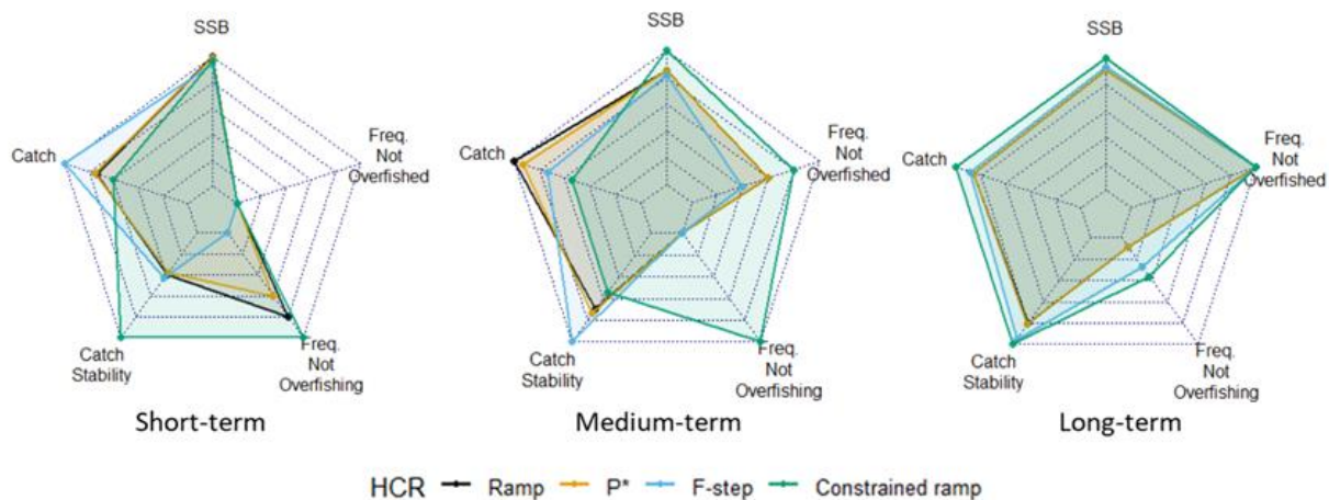
Figure 66. Harvest control rule (HCR) performance for Gulf of Maine cod with a natural mortality stock assessment model misspecification (Overfished Mortality and Recruitment Misspecified Scenario) and annual stock assessment updates (Frequency Scenario 2) in the short- (1-5 years), medium- (6-10 years), and long-term (11-20 years). Metrics are standardized to the maximum value for each metric attained by the different HCRs and equally weighted. Spawning stock biomass (SSB) and catch are median SSB and catch for the time period.
