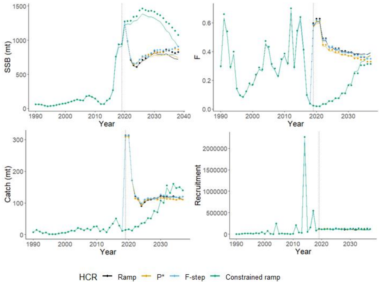
Figure 76. True operating model (closed circles) and estimated stock assessment values from the terminal assessment (stock assessment completed in 2039 with a terminal year of 2038; lines) of spawning stock biomass (SSB), fishing mortality (F), catch (mt), and recruits for Georges Bank haddock with a survey catchability stock assessment model misspecification (Not Overfished Catchability Misspecified Scenario) from 1982 to 2038 for SSB and 2037 for other metrics. The dashed line represents the beginning of the management procedure period (2019).
