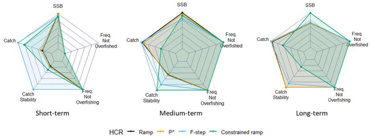
Figure 12. Harvest control rule (HCR) performance for Gulf of Maine cod with no stock assessment model misspecification (Base Case Overfished Scenario) in the short- (1-5 years), medium- (6-10 years), and long-term (11-21 years). Metrics are standardized to the maximum value for each metric attained by the different HCRs and equally weighted. Spawning stock biomass (SSB) and catch are median SSB and catch for the time period.
