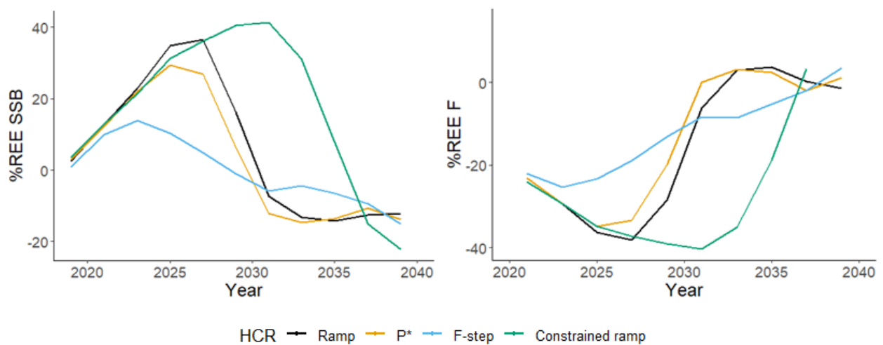
Figure 43. Percent relative error (REE) in terminal estimated spawning stock biomass (SSB) and fishing mortality (F) for Gulf of Maine cod with a stock assessment misspecification (Overfished Mortality and Recruitment Misspecification Scenario) and year one projection held constant (Projection sub-alternative b).
