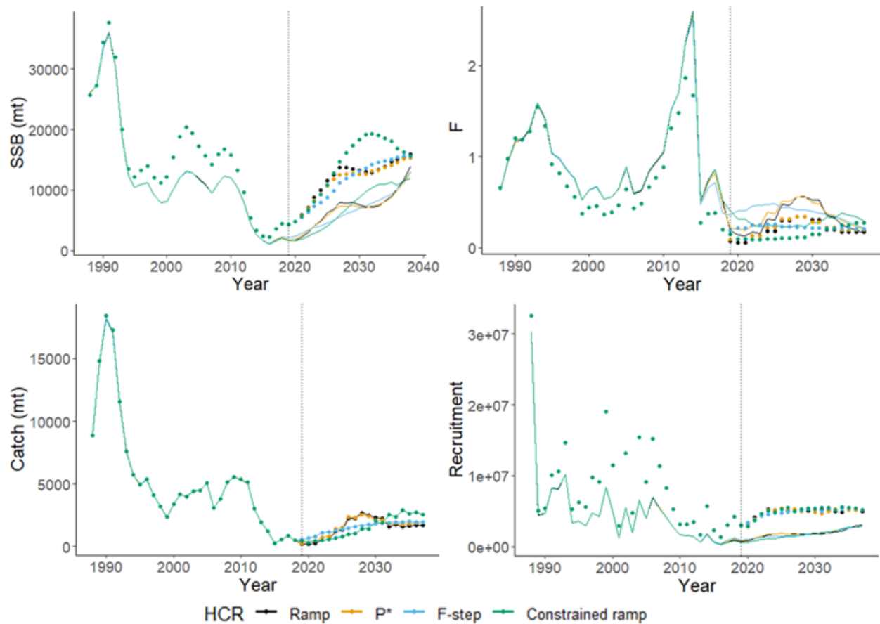
Figure 13. True operating model (closed circles) and estimated stock assessment values from the terminal assessment (stock assessment completed in 2039 with a terminal year of 2038; lines) of spawning stock biomass (SSB), fishing mortality (F), catch (mt), and recruits for Gulf of Maine cod with a natural mortality stock assessment model misspecification (Overfished Mortality Misspecified Scenario) from 1982 to 2038 for SSB and 2037 for other metrics. The dashed line represents the beginning of the management procedure period (2019).
