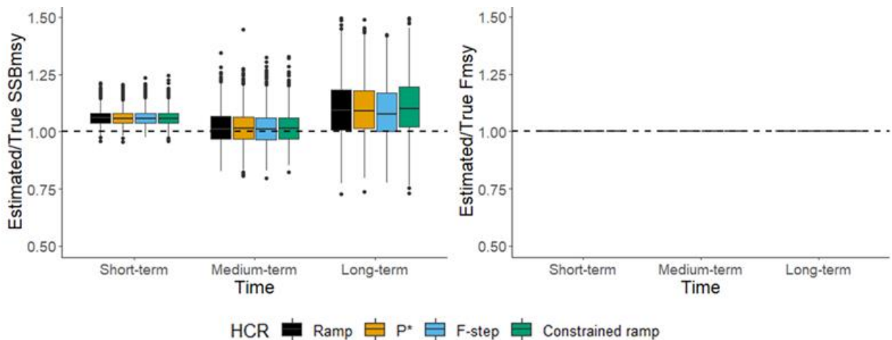
Figure 27. Median ratios of estimated to true ratios of the stock biomass reference point (SSB MSY ) and fishing mortality biomass reference point (F MSY ) for a stock originally undergoing overfishing and overfished (Gulf of Maine cod) with a recruitment stock assessment model misspecification (Overfished Recruitment Misspecified Scenario) in the short- (1-5 years), medium- (5-10 years), and long-term (10-20 years).
