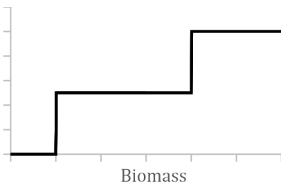
Figure 6. Harvest control rule with target and limit reference points.
