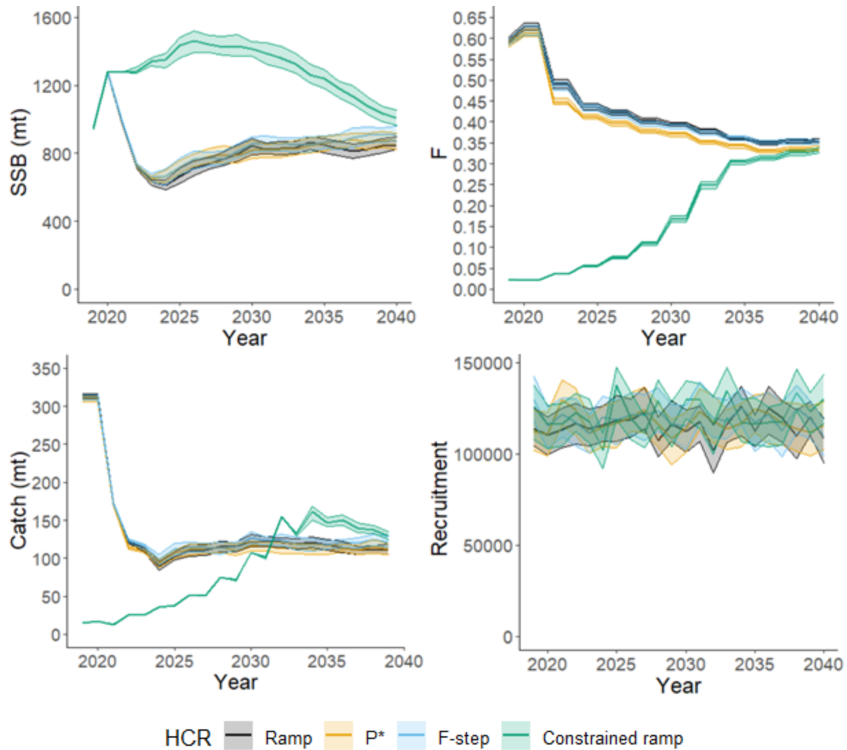
Figure 77. True operating model median spawning stock biomass (SSB), fishing mortality (F), catch (mt), and recruits with 95% confidence intervals for Georges Bank haddock with a survey catchability stock assessment model misspecification (Not Overfished Catchability Misspecified Scenario) from 2019 to 2040.
