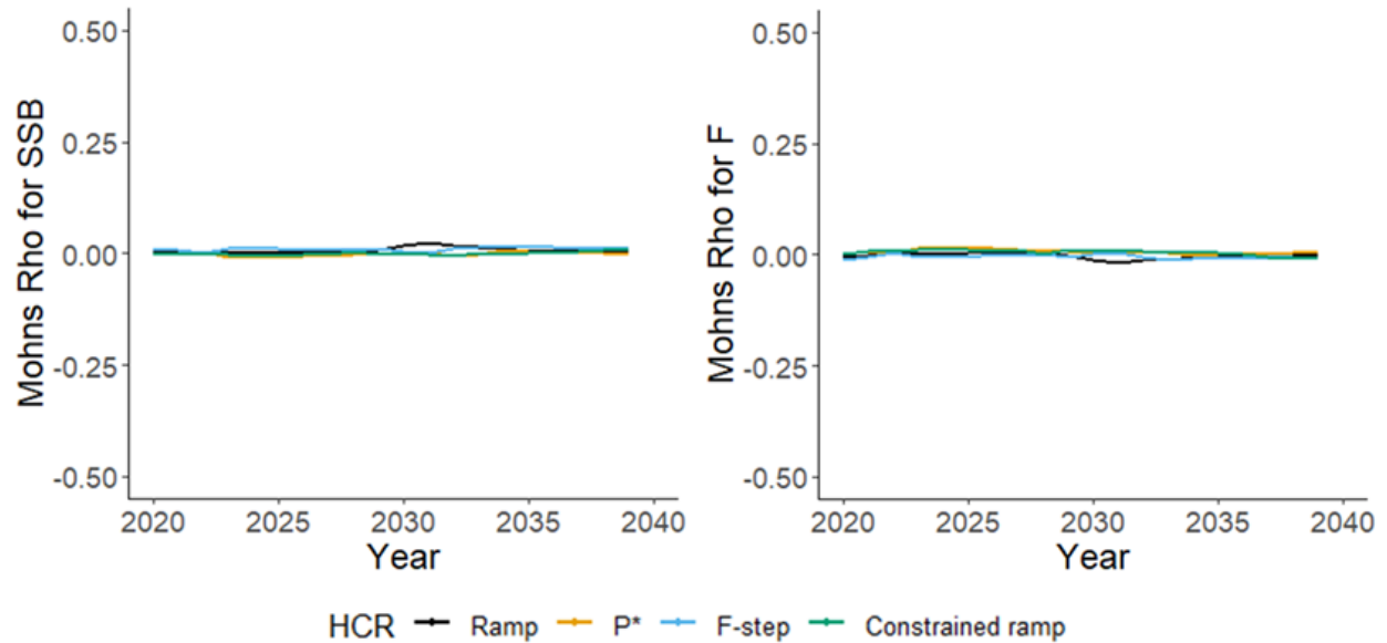
Figure 8. Mohn's Rho values for spawning stock biomass (SSB) and fishing mortality (F) for Gulf of Maine cod with no stock assessment model misspecification (Base Case Overfished Scenario).
