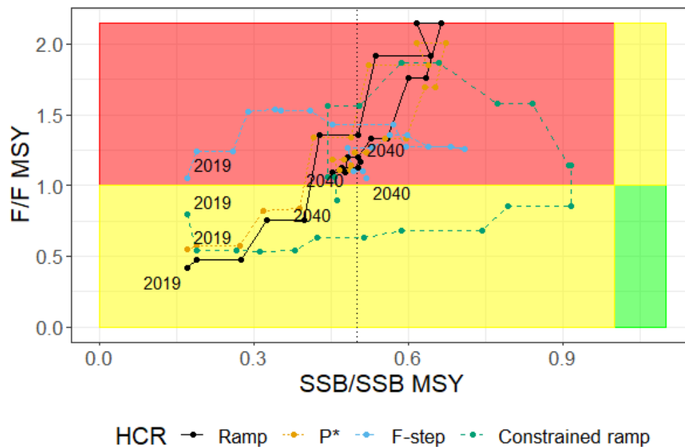
Figure 37. a) Estimated terminal stock status of each year's stock assessment relative to M=0.2 reference points ( F/F_{MSY} and SSB/SSB_{MSY} ), b) True stock status relative to M=0.2 reference points for Gulf of Maine cod with a natural mortality and recruitment stock assessment model misspecification (Overfished Mortality and Recruitment Misspecified Scenario). The dashed line represents the overfished threshold.
