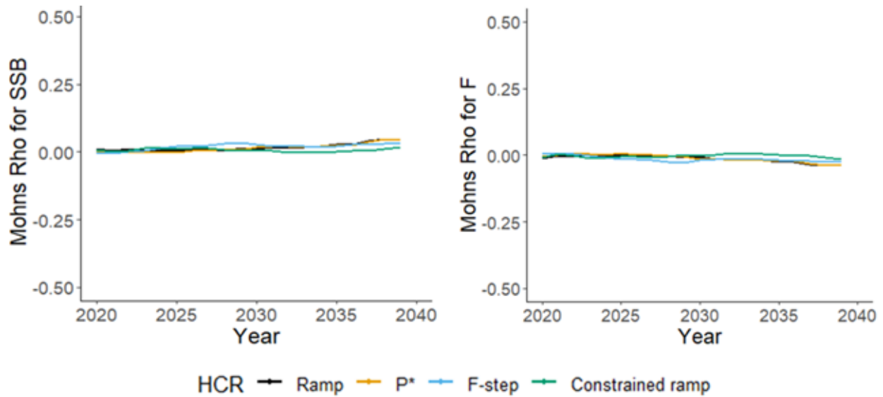
Figure 26. Mohn's Rho values for spawning stock biomass (SSB) and fishing mortality (F) for Gulf of Maine cod with a recruitment stock assessment model misspecification (Overfished Recruitment Misspecified Scenario).
