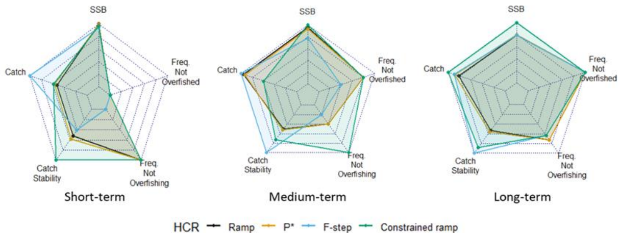
Figure 57. Harvest control rule (HCR) performance for Gulf of Maine cod with a natural mortality stock assessment model misspecification (Overfished Mortality and Recruitment Misspecified Scenario) and a rho-adjustment (Rho Scenario 1) in the short- (1-5 years), medium- (6-10 years), and long-term (11-21 years). stock biomass (SSB) and catch are median SSB and catch for the time period.
