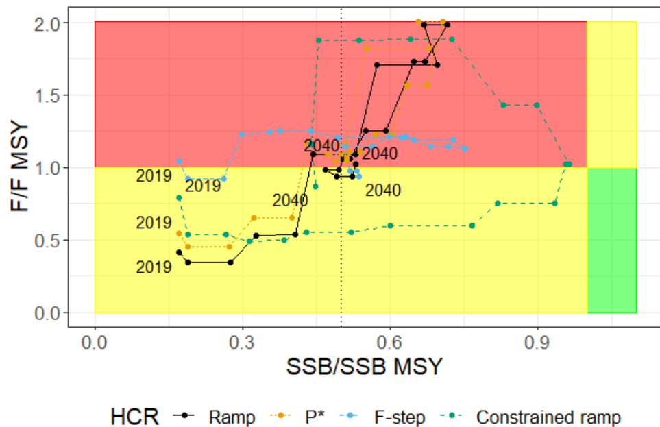
Figure 46. a) Estimated terminal stock status of each year's stock assessment relative to M=0.2 reference points ( F/F_{MSY} and SSB/SSB_{MSY} ), b) True stock status relative to M=0.2 reference points for Gulf of Maine cod with a stock assessment misspecification (Overfished Mortality and Recruitment Misspecification Scenario) with year one projection held constant (Projection sub-alternative b). The dashed line represents the overfished threshold.
