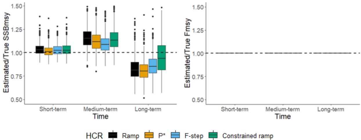
Figure 54. Median ratios of estimated to true stock biomass reference point ( SSB_{MSY} ) and fishing mortality biomass reference point ( F_{MSY} ) for Gulf of Maine cod with a natural mortality stock assessment model misspecification (Overfished Mortality and Recruitment Misspecified Scenario) and a rho-adjustment (Rho Scenario 1) in the short- (1-5 years), medium- (6-10 years), and long-term (11-21 years).
