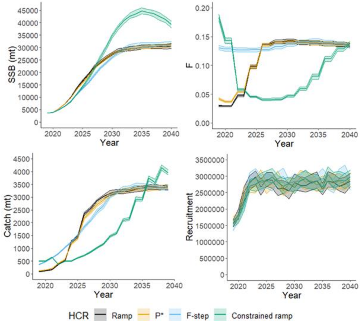
Figure 5. True operating model median spawning stock biomass (SSB), fishing mortality (F), catch (mt), and recruits with 95% confidence intervals for Gulf of Maine cod with no stock assessment model misspecification (Base Case Overfished Scenario) from 2019 to 2040.
