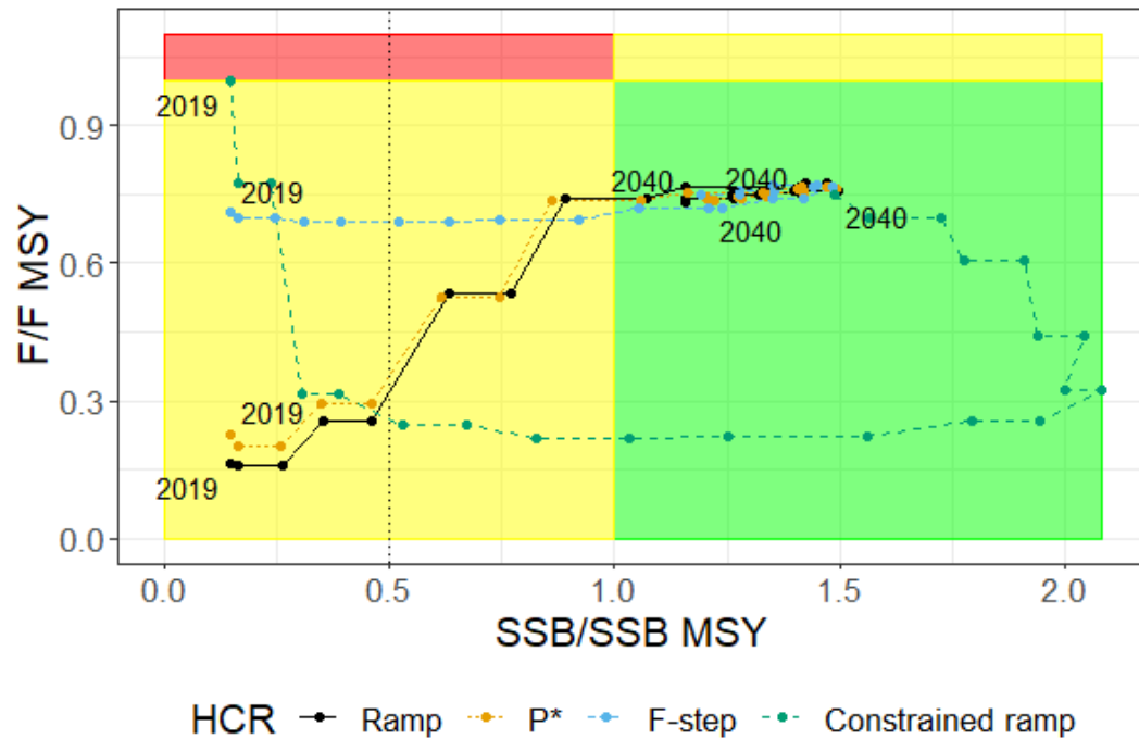
Figure 10. True stock status trajectories (ratio of fishing mortality to the fishing mortality reference point ( F/F_{MSY} ) versus ratio of spawning stock biomass to the spawning stock biomass reference point ( SSB/SSB_{MSY} )) for Gulf of Maine cod with no stock assessment model misspecification (Base Case Overfished Scenario). The dashed line represents the overfished threshold.
