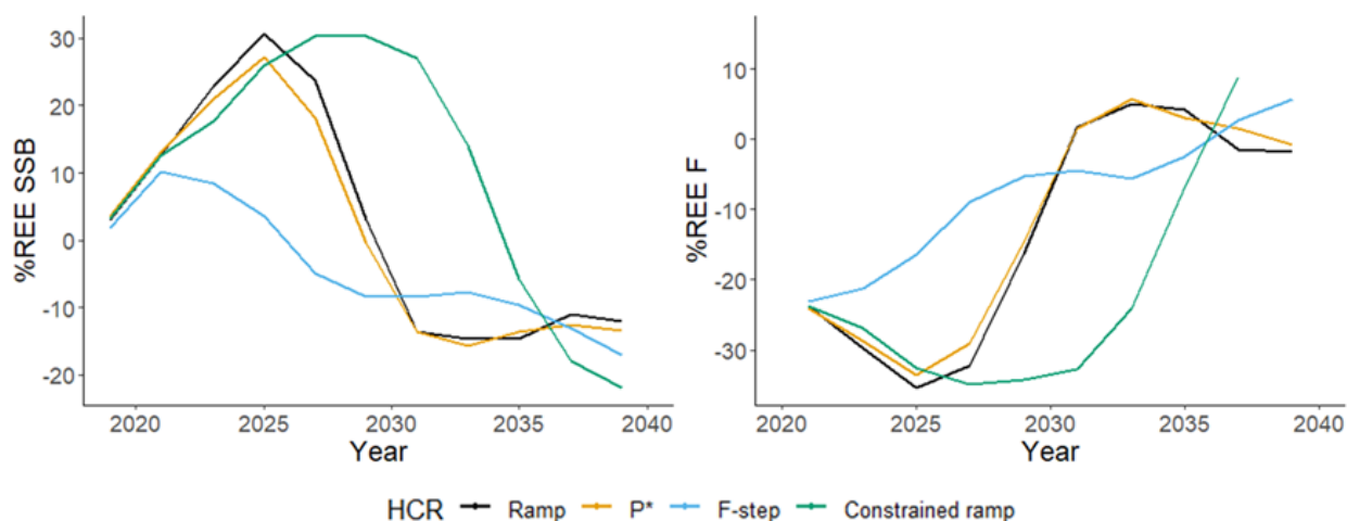
Figure 34. Percent relative error (REE) in terminal estimated spawning stock biomass (SSB) and fishing mortality (F) for Gulf of Maine cod with a natural mortality and recruitment stock assessment model misspecification (Overfished Mortality and Recruitment Misspecified Scenario).
