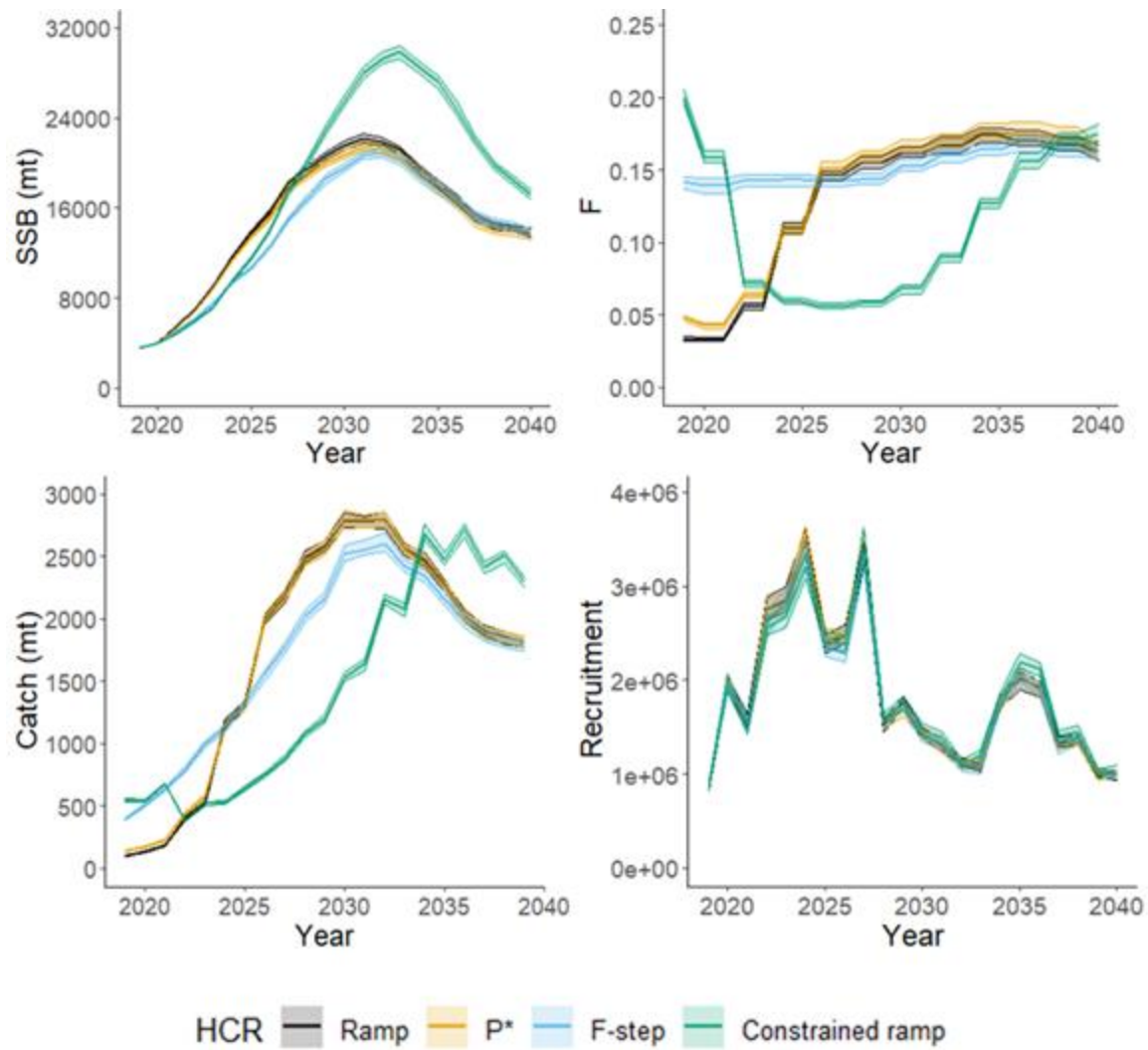
Figure 23. True operating model median spawning stock biomass (SSB), fishing mortality (F), catch (mt), and recruits with 95% confidence intervals for Gulf of Maine cod with a recruitment stock assessment model misspecification (Overfished Recruitment Misspecified Scenario) from 2019 to 2040.
