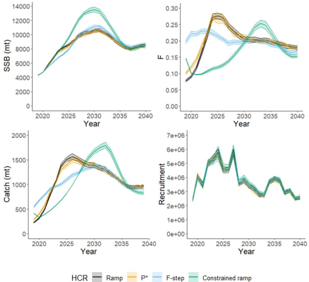
Figure 59. True operating model median spawning stock biomass (SSB), fishing mortality (F), catch (mt), and recruits with 95% confidence intervals for Gulf of Maine cod with a natural mortality stock assessment model misspecification (Overfished Mortality and Recruitment Misspecified Scenario) and annual stock assessment updates (Frequency Scenario 2) from 2019 to 2040.
