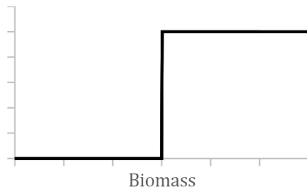
Figure A4. Threshold harvest control rule.
