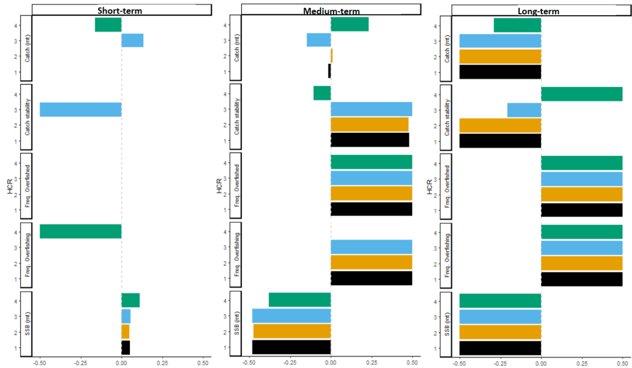
Figure 87. Short- (1-5 years), medium- (6-10 years), and long-term (11-21 years) relative difference in harvest control rule performance between the Base Case Overfished Scenario and the Overfished Mortality and Recruitment Misspecified Scenario.
