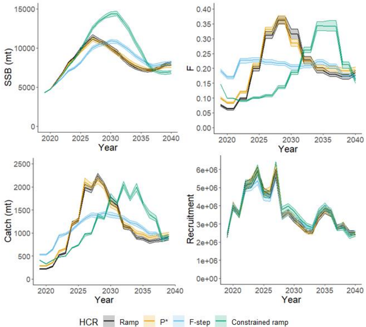
Figure 41. True operating model median spawning stock biomass (SSB), fishing mortality (F), catch (mt), and recruits with 95% confidence intervals for Gulf of Maine cod with a stock assessment misspecification (Overfished Mortality and Recruitment Misspecification Scenario) and year one projection held constant (Projection sub-alternative b) from 2019 to 2040.
