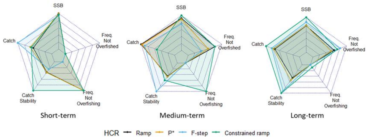
Figure 39. Harvest control rule (HCR) performance for Gulf of Maine cod with a natural mortality and recruitment stock assessment model misspecification (Overfished Mortality and Recruitment Misspecified Scenario) in the short- (1-5 years), medium- (6-10 years), and long-term (11-21 years). Metrics are standardized to the maximum value for each metric attained by the different HCRs and equally weighted. Spawning stock biomass (SSB) and catch are median SSB and catch for the time period.
