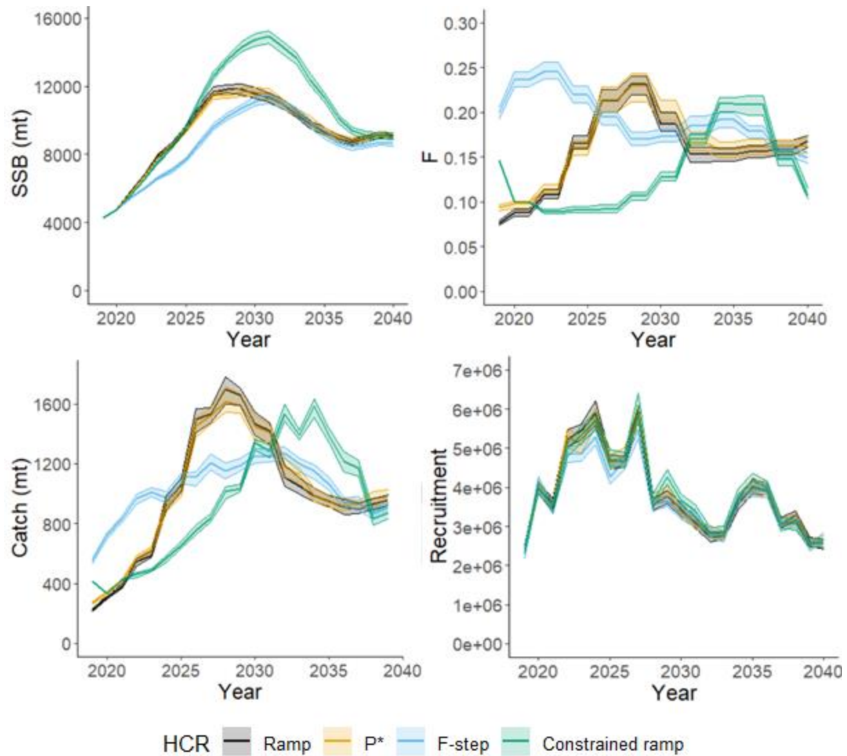
Figure 50. True operating model median spawning stock biomass (SSB), fishing mortality (F), catch (mt), and recruits with 95% confidence intervals for Gulf of Maine cod with natural mortality and recruitment stock assessment model misspecification (Overfished Mortality and Recruitment Misspecified Scenario) and a rho-adjustment (Rho Scenario 1) from 2019 to 2040.
