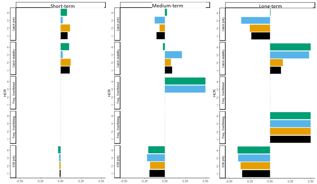
Figure 86. Short- (1-5 years), medium- (6-10 years), and long-term (11-21 years) relative difference in harvest control rule performance between the Base Case Overfished Scenario and the Overfished Recruitment Misspecified Scenario.
