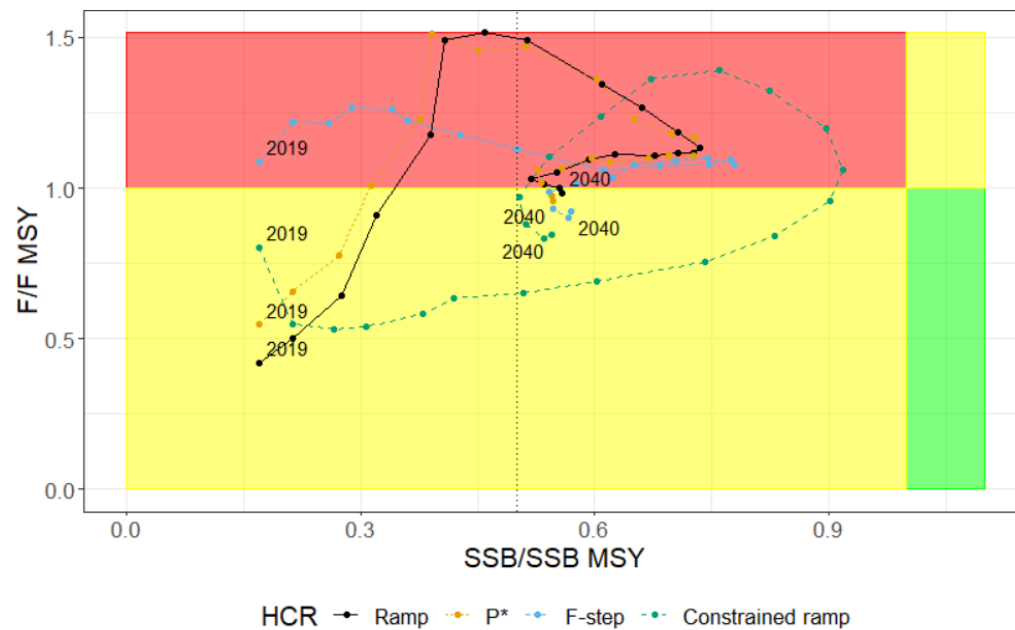
Figure 64. a) Estimated terminal stock status of each year's stock assessment relative to M=0.2 reference points ( F/F_{MSY} and SSB/SSB_{MSY} ), b) True stock status relative to M=0.2 reference points for Gulf of Maine cod with a stock assessment model misspecification (Overfished Mortality and Recruitment Misspecified Scenario) and annual stock assessment updates (Frequency Scenario 2). The dashed line represents the overfished threshold.
