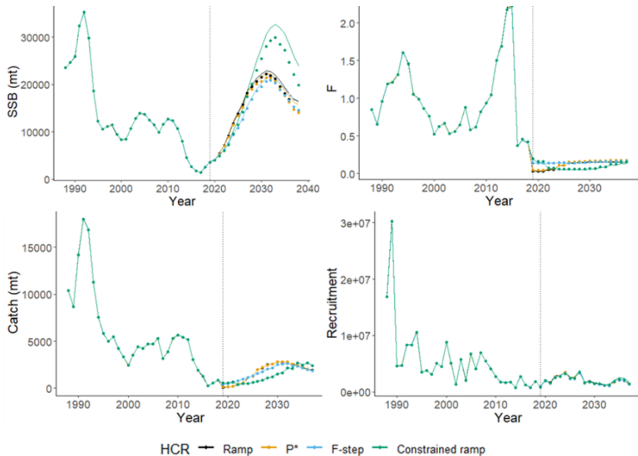
Figure 22. True operating model (closed circles) and estimated stock assessment values from the terminal assessment (stock assessment completed in 2039 with a terminal year of 2038; lines) of spawning stock biomass (SSB), fishing mortality (F), catch (mt), and recruits for Gulf of Maine cod with a recruitment stock assessment model misspecification (Overfished Recruitment Misspecified Scenario) from 1982 to 2038 for SSB and 2037 for other metrics. The dashed line represents the beginning of the management procedure period (2019).
