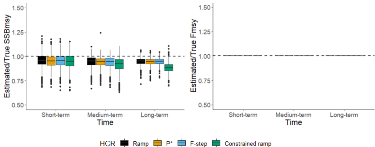
Figure 81. Median ratios of estimated to true ratios of the stock biomass reference point ( SSB_{MSY} ) and fishing mortality biomass reference point ( F_{MSY} ) for a stock originally not undergoing overfishing and not overfished (Georges Bank haddock) with a survey catchability stock assessment model misspecification (Not Overfished Catchability Misspecified Scenario) in the short- (1-5 years), medium- (5-10 years), and long-term (10-20 years).
