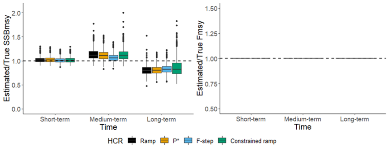
Figure 36. Median ratios of estimated to true stock biomass reference point ( SSB_{MSY} ) and fishing mortality biomass reference point ( F_{MSY} ) for Gulf of Maine cod with a natural mortality and recruitment stock assessment model misspecification (Overfished Mortality and Recruitment Misspecified Scenario) in the short- (1-5 years), medium- (6-10 years), and long-term (11-21 years).
