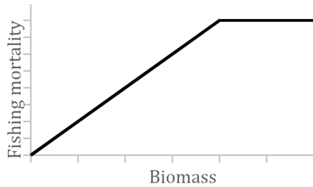
Figure B5. Ramped harvest control rule.
