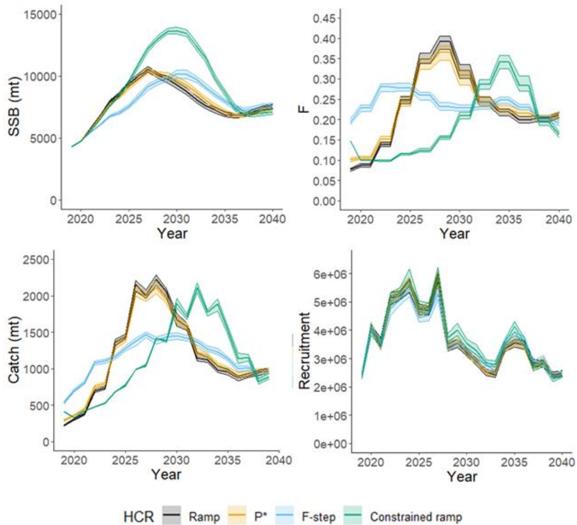
Figure 32. True operating model median spawning stock biomass (SSB), fishing mortality (F), catch (mt), and recruits with 95% confidence intervals for Gulf of Maine cod with a natural mortality and recruitment stock assessment model misspecification (Overfished Mortality and Recruitment Misspecified Scenario) from 2019 to 2040.
