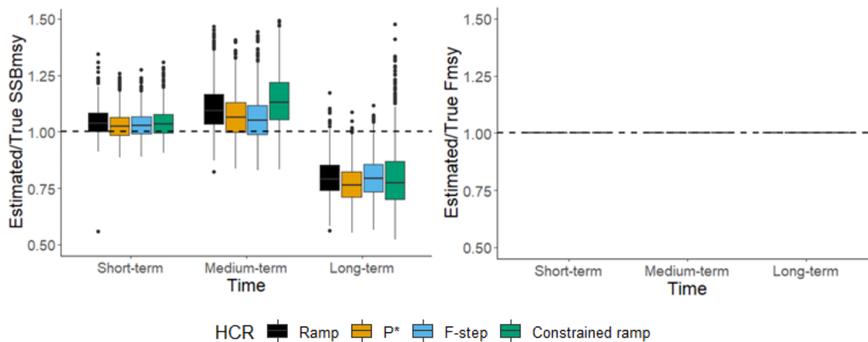
Figure 63. Median ratios of estimated to true stock biomass reference point (SSB MSY ) and fishing mortality biomass reference point (F MSY ) for Gulf of Maine cod with a natural mortality stock assessment model misspecification (Overfished Mortality and Recruitment Misspecified Scenario) and annual stock assessment updates (Frequency Scenario 2) in the short- (1-5 years), medium- (6-10 years), and long-term (11-21 years).
