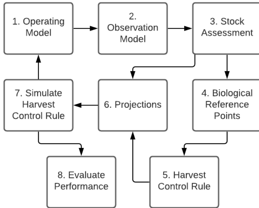
Figure 1. The management strategy evaluation framework used in this project.
