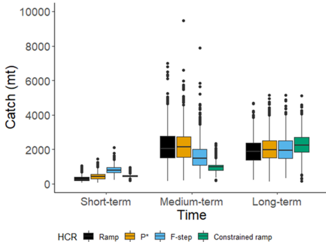
Figure 15. True median catch for Gulf of Maine cod with a natural mortality stock assessment model misspecification (Overfished Mortality Misspecified Scenario) in the short- (1-5 years), medium- (6-10 years), and long-term (11-21 years).
