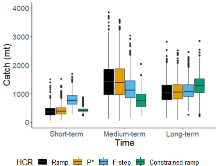
Figure 51. True median catch for Gulf of Maine cod with natural mortality and recruitment stock assessment model misspecifications (Overfished Mortality and Recruitment Misspecified Scenario) and a rho-adjustment (Rho Scenario 1) in the short- (1-5 years), medium- (6-10 years), and long-term (11-21 years).
