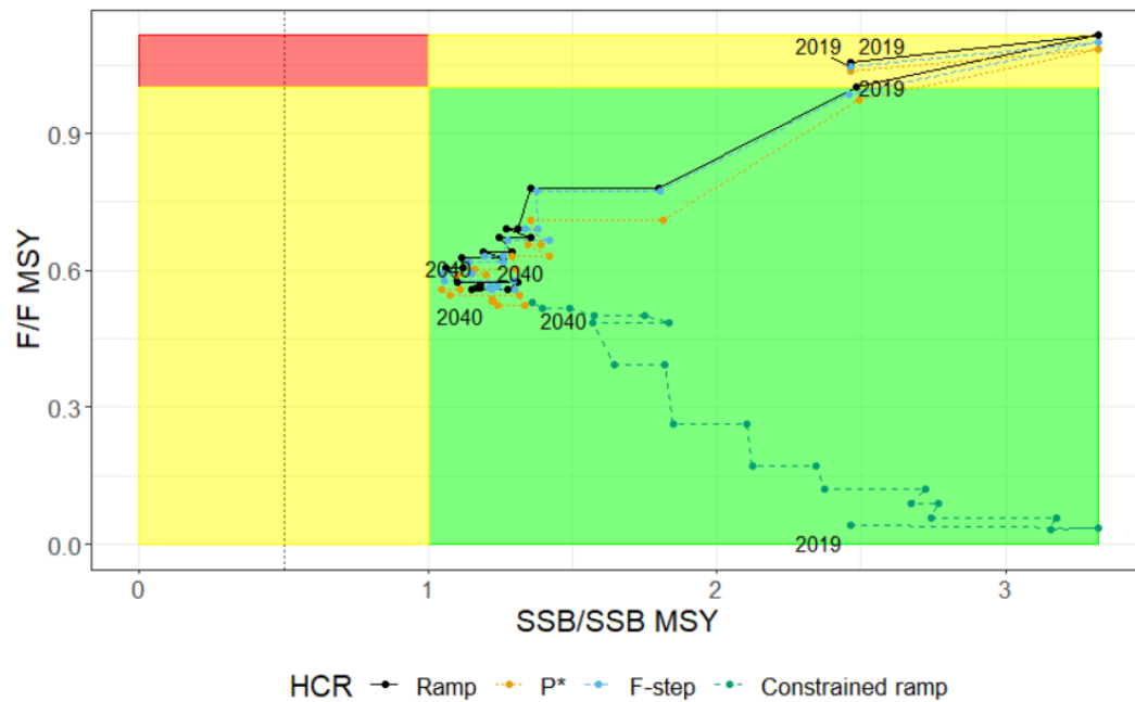
Figure 82. a) Estimated terminal stock status of each year's stock assessment relative to M=0.2 reference points ( F/F_{MSY} and SSB/SSB_{MSY} ), b) True stock status relative to M=0.2 reference points for Georges Bank haddock with a survey catchability stock assessment model misspecification (Not Overfished Catchability Misspecified Scenario). The dashed line represents the overfished threshold.
