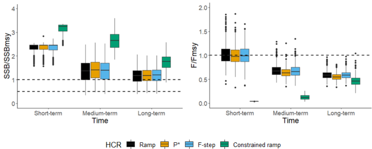
Figure 83. True median ratios of spawning stock biomass to the spawning stock biomass reference point ( SSB/SSB_{MSY} ) and fishing mortality to the fishing mortality biomass reference point ( F/F_{MSY} ) for Georges Bank haddock with a survey catchability stock assessment model misspecification (Not Overfished Catchability Misspecified Scenario) in the short- (1-5 years), medium- (6-10 years), and long-term (11-21 years).
