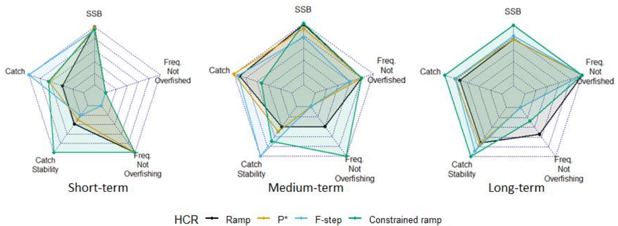
Figure 21. Harvest control rule (HCR) performance for Gulf of Maine cod with a natural mortality stock assessment model misspecification (Overfished Mortality Misspecified Scenario) in the short- (1-5 years), medium- (6-10 years), and long-term (11-20 years). Metrics are standardized to the maximum value for each metric attained by the different HCRs and equally weighted. Spawning stock biomass (SSB) and catch are median SSB and catch for the time period.
