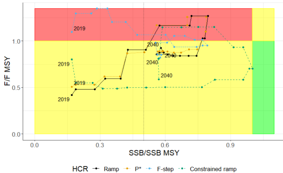
Figure 55. a) Estimated terminal stock status of each year's stock assessment relative to M=0.2 reference points ( F/F_{MSY} and SSB/SSB_{MSY} ), b) True stock status relative to M=0.2 reference points for Gulf of Maine cod with a stock assessment model misspecification (Overfished Mortality and Recruitment Misspecified Scenario) and a rho-adjustment (Rho Scenario 1). The dashed line represents the overfished threshold.
