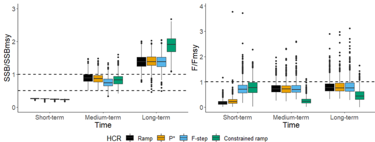
Figure 11. True median ratios of spawning stock biomass to the spawning stock biomass reference point ( SSB/SSB_{MSY} ) and fishing mortality to the fishing mortality biomass reference point ( F/F_{MSY} ) for Gulf of Maine cod with no stock assessment model misspecification (Base Case Overfished Scenario) in the short- (1-5 years), medium- (6-10 years), and long-term (11-21 years).
