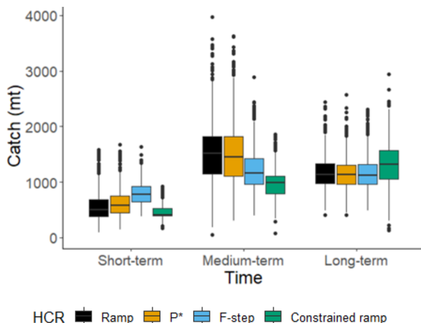
Figure 60. True median catch for Gulf of Maine cod with a natural mortality stock assessment model misspecification (Overfished Mortality and Recruitment Misspecified Scenario) and annual stock assessment updates (Frequency Scenario 2) in the short- (1-5 years), medium- (6-10 years), and long-term (11-21 years).
