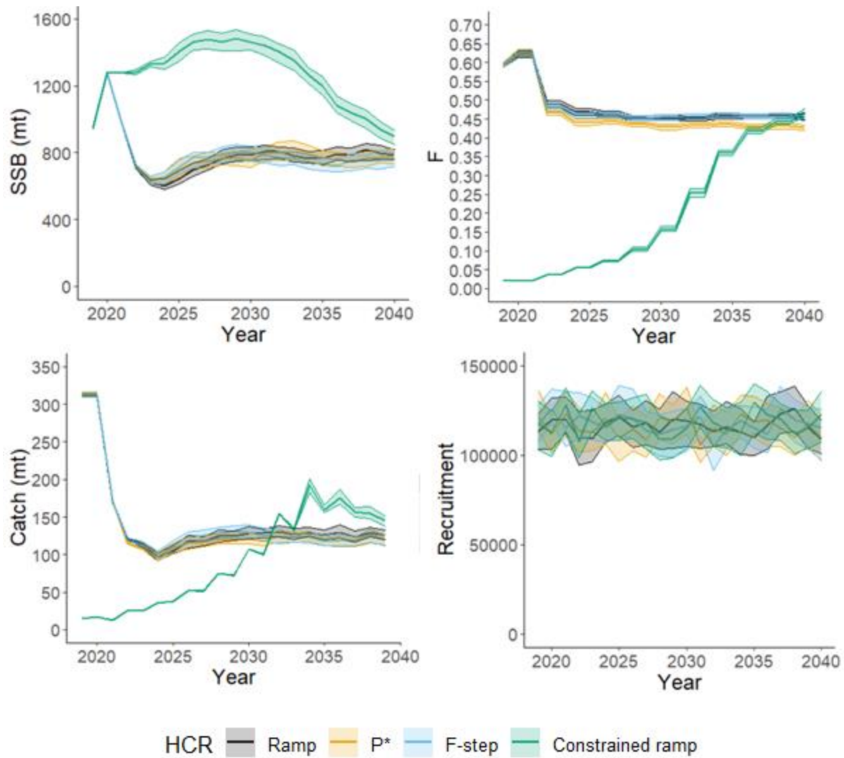
Figure 68. True operating model median spawning stock biomass (SSB), fishing mortality (F), catch (mt), and recruits with 95% confidence intervals for Georges Bank haddock with no stock assessment model misspecification (Base Case Not Overfished Scenario) from 2019 to 2040.
