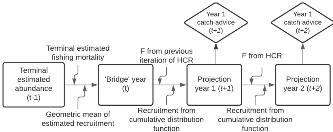
Figure 2. Projection process with a two-year stock assessment update frequency. t-1 = terminal year of assessment, t = current year, t+1 = next year, t+2 = year after next year.
