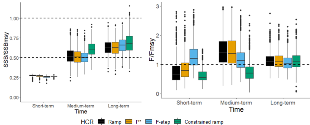
Figure 65. True median ratios of spawning stock biomass to the spawning stock biomass reference point ( SSB/SSB_{MSY} ) and fishing mortality to the fishing mortality biomass reference point ( F/F_{MSY} ) for Gulf of Maine cod with a natural mortality stock assessment model misspecification (Overfished Mortality and Recruitment Misspecified Scenario) and annual stock assessment updates (Frequency Scenario 2) in the short- (1-5 years), medium- (6-10 years), and long-term (11-21 years).
