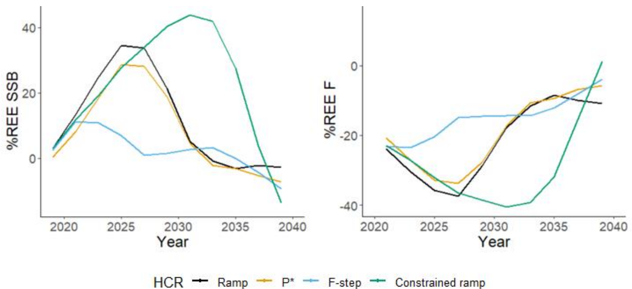
Figure 52. Percent relative error (REE) in terminal estimated spawning stock biomass (SSB) and fishing mortality (F) for Gulf of Maine cod with a stock assessment model misspecification (Overfished Mortality and Recruitment Misspecified Scenario) and a rho-adjustment (Rho Scenario 1).
