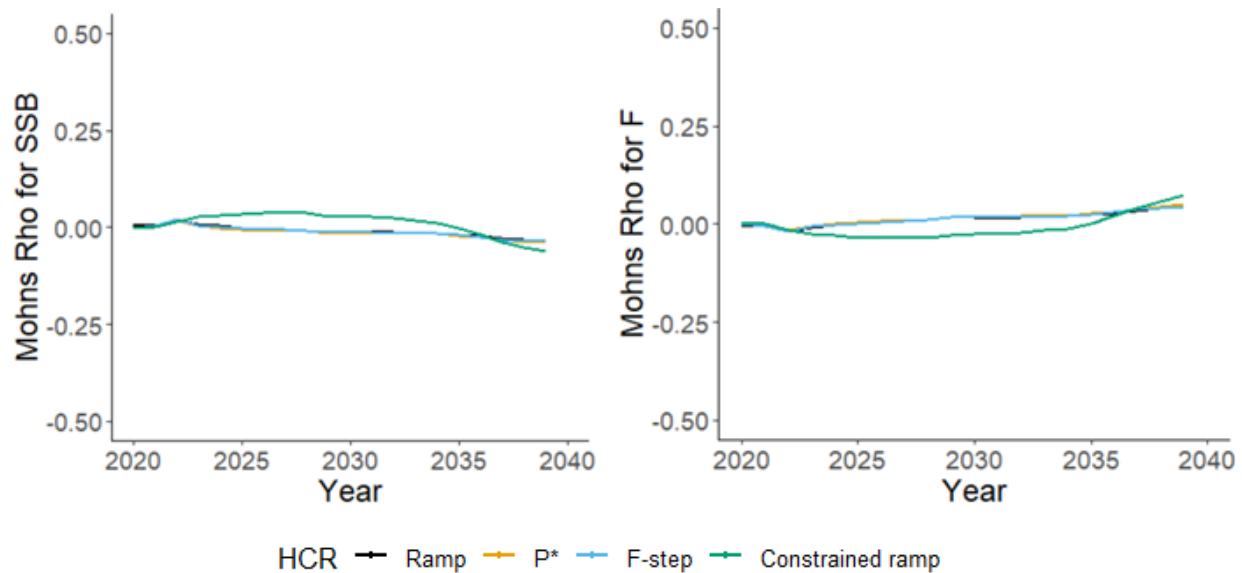
Figure 80. Mohn's Rho values for spawning stock biomass (SSB) and fishing mortality (F) for Georges Bank haddock with a survey catchability stock assessment model misspecification (Not Overfished Catchability Misspecified Scenario).
