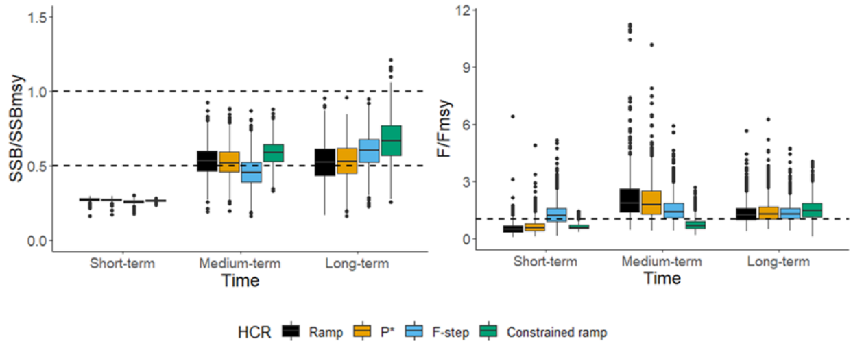
Figure 38. True median ratios of spawning stock biomass to the spawning stock biomass reference point ( SSB/SSB_{MSY} ) and fishing mortality to the fishing mortality biomass reference point ( F/F_{MSY} ) for Gulf of Maine cod with a natural mortality and recruitment stock assessment model misspecification (Overfished Mortality and Recruitment Misspecified Scenario) in the short- (1-5 years), medium- (6-10 years), and long-term (11-21 years).
