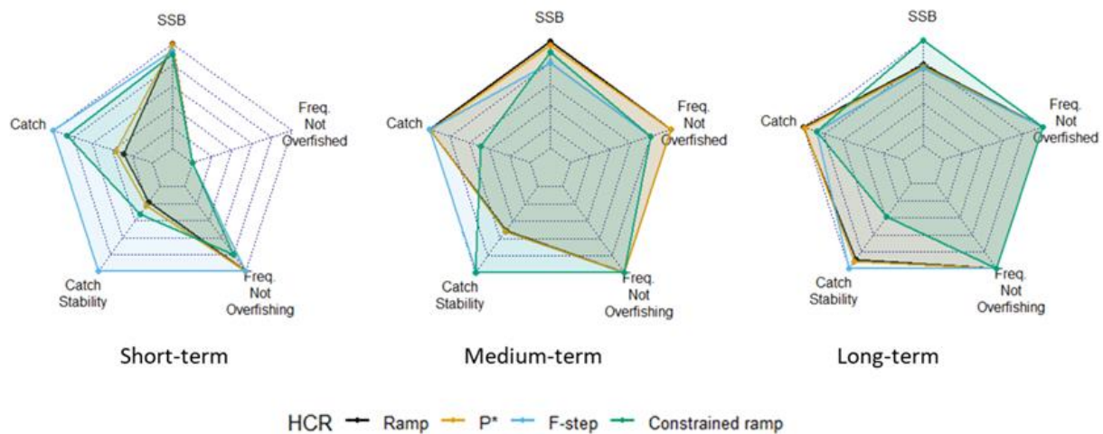
Figure 30. Harvest control rule (HCR) performance for Gulf of Maine cod with a recruitment stock assessment model misspecification (Overfished Recruitment Misspecified Scenario) in the short- (1-5 years), medium- (6-10 years), and long-term (10-20 years). Metrics are standardized to the maximum value for each metric attained by the different HCRs and equally weighted. Spawning stock biomass (SSB) and catch are median SSB and catch for the time period.
