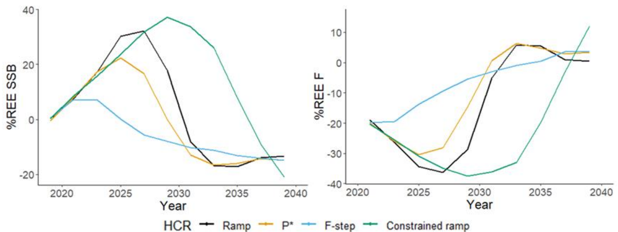
Figure 16. Percent relative error (REE) in terminal estimated spawning stock biomass (SSB) and fishing mortality (F) for Gulf of Maine cod with a natural mortality stock assessment model misspecification (Overfished Mortality Misspecified Scenario).
