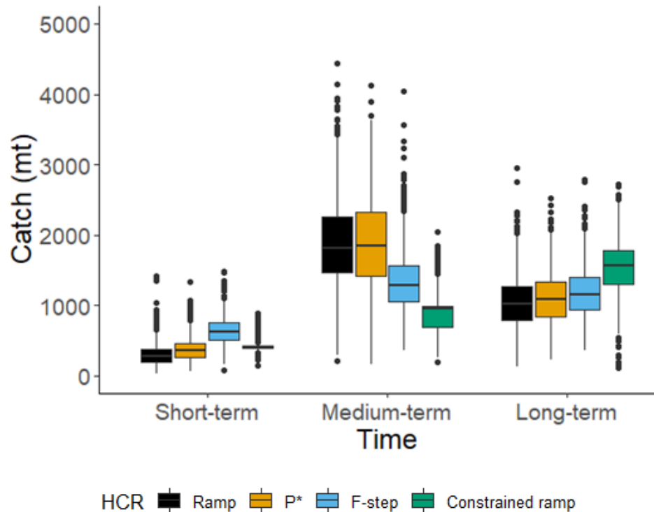
Figure 42. True median catch for Gulf of Maine cod with a stock assessment misspecification (Overfished Mortality and Recruitment Misspecification Scenario) with year one projection held constant (Projection sub-alternative b) in the short- (1-5 years), medium- (6-10 years), and long-term (11-21 years).
