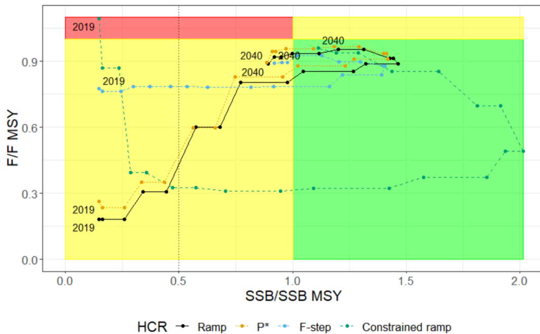
Figure 28. a) Estimated terminal stock status of each year's stock assessment relative to M=0.2 reference points ( F/F_{MSY} and SSB/SSB_{MSY} ), b) True stock status relative to M=0.2 reference points for Gulf of Maine cod with a stock assessment model misspecification (Overfished Recruitment Misspecified Scenario). The dashed line represents the overfished threshold.
