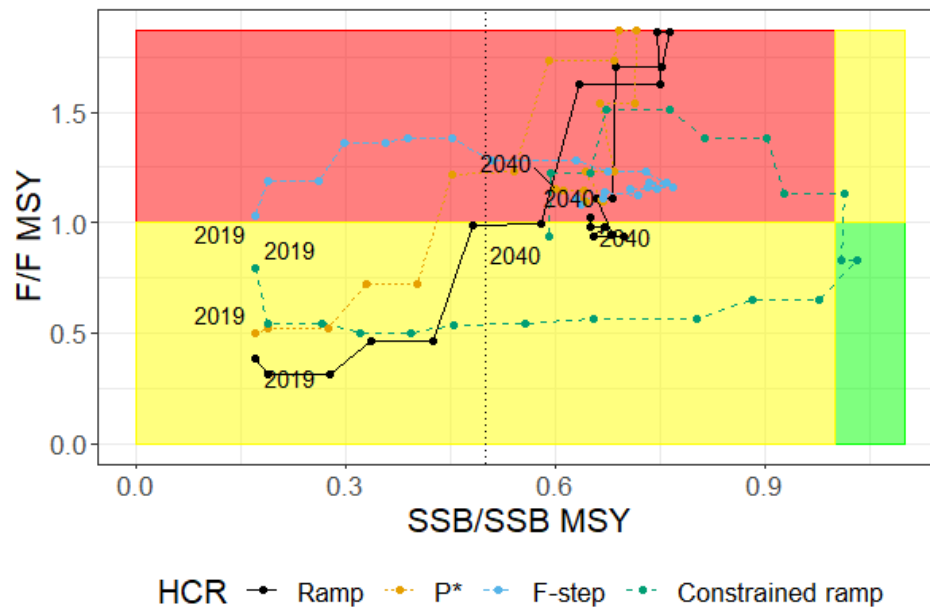
Figure 19. a) Estimated terminal stock status of each year's stock assessment relative to M=0.2 reference points ( F/F_{MSY} and SSB/SSB_{MSY} ), b) True stock status relative to M=0.2 reference points for Gulf of Maine cod with a stock assessment model misspecification (Overfished Mortality Misspecified Scenario). The dashed line represents the overfished threshold.
