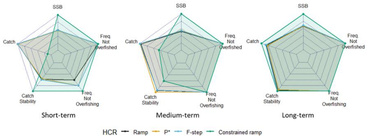
Figure 84. Harvest control rule (HCR) performance for Georges Bank haddock with a survey catchability stock assessment model misspecification (Not Overfished Misspecified Scenario) in the short- (1-5 years), medium- (6-10 years), and long-term (11-20 years). Metrics are standardized to the maximum value for each metric attained by the different HCRs and equally weighted. Spawning stock biomass (SSB) and catch are median SSB and catch for the time period.
