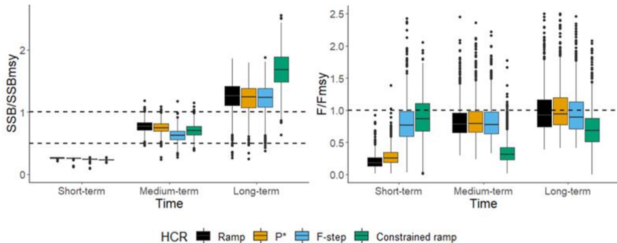
Figure 29. True median ratios of spawning stock biomass to the spawning stock biomass reference point ( SSB/SSB_{MSY} ) and fishing mortality to the fishing mortality biomass reference point ( F/F_{MSY} ) for Gulf of Maine cod with a recruitment stock assessment model misspecification (Overfished Recruitment Misspecified Scenario) in the short- (1-5 years), medium- (5-10 years), and long-term (10-20 years).
