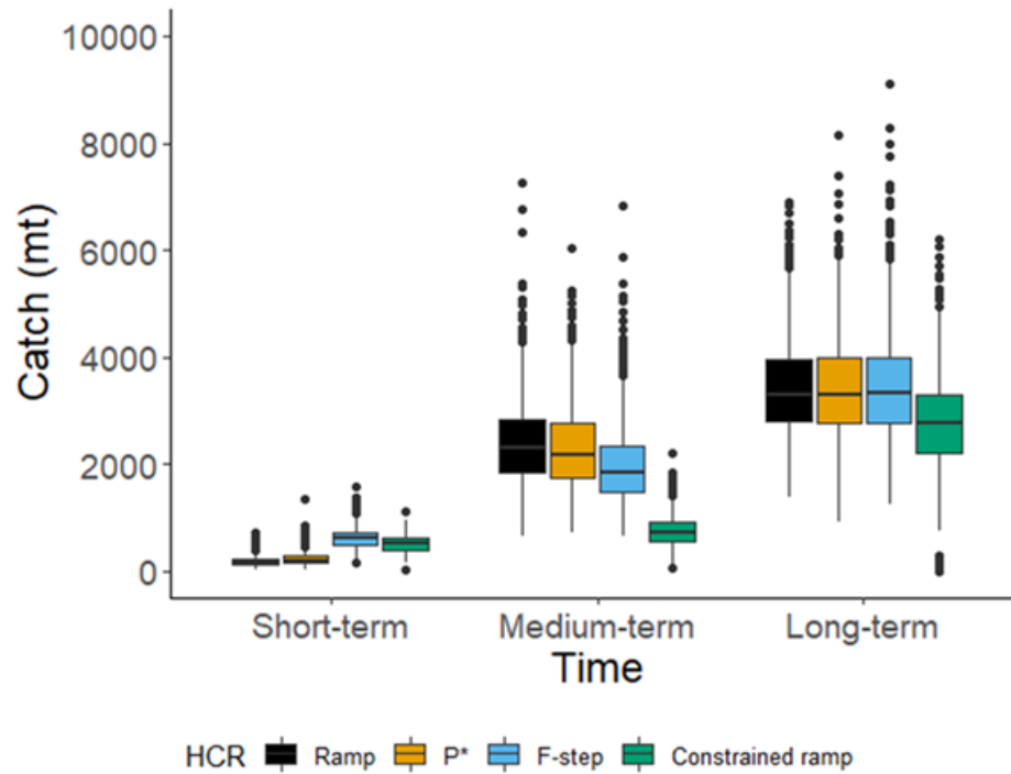
Figure 6. True median catch for Gulf of Maine cod with no stock assessment model misspecification (Base Case Overfished Scenario) in the short- (1-5 years), medium- (6-10 years), and long-term (11-21 years).
