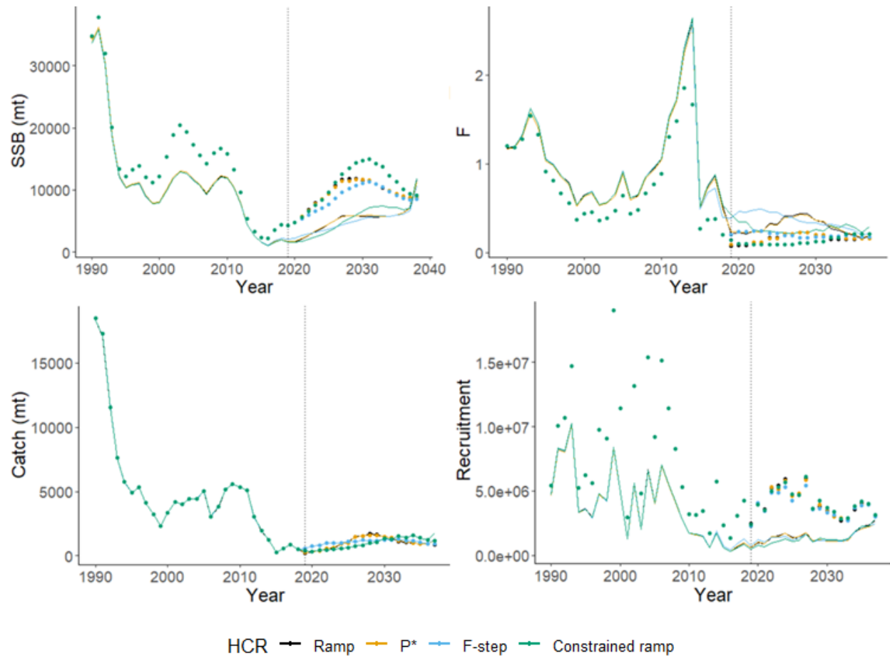
Figure 49. True operating model (closed circles) and estimated stock assessment values from the terminal assessment (stock assessment completed in 2039 with a terminal year of 2038; lines) of spawning stock biomass (SSB), fishing mortality (F), catch (mt), and recruits for Gulf of Maine cod with natural mortality and recruitment stock assessment model misspecifications (Overfished Mortality and Recruitment Misspecified Scenario) and a rho-adjustment (Rho Scenario 1) from 1982 to 2038 for SSB and 2037 for other metrics. The dashed line represents the beginning of the management procedure period (2019).
