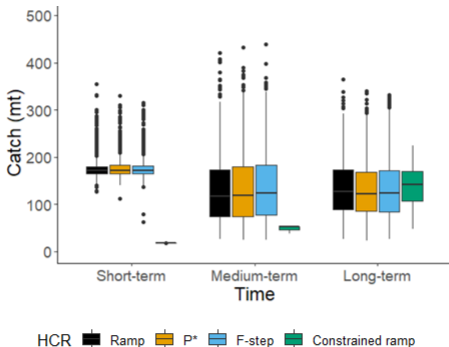
Figure 69. True median catch for Georges Bank haddock with no stock assessment model misspecification (Base Case Not Overfished Scenario) in the short- (1-5 years), medium- (6-10 years), and long-term (11-21 years).
